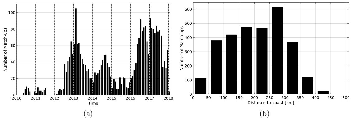
Figure 1: Number of match-ups between Argo and SMOS-L4-CATDS-CECOS-IFREMER-V2-WEEKLY-0.5DEG SSS as a function of time (a) and as function of the distance to coast (b) over the South China Sea Pi-MEP region and for the full satellite product period.
