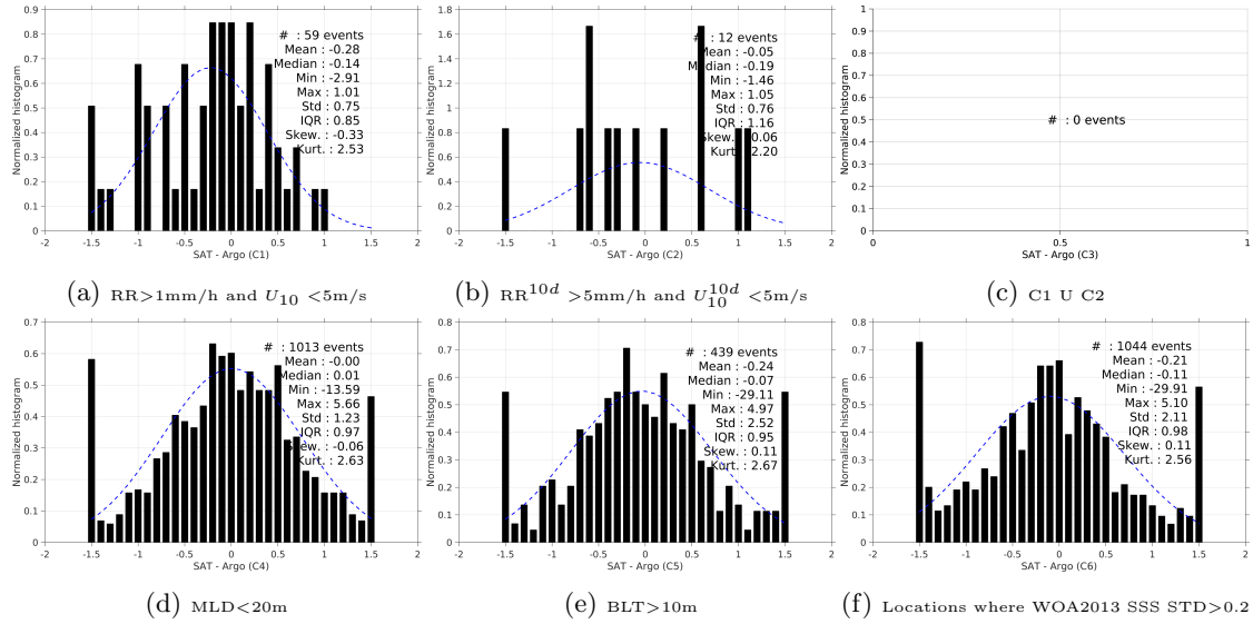
Figure 13: Normalized histogram of \Delta SSS (SMOS-L4-CATDS-CECOS-IFREMER-V2-WEEKLY-0.5DEG - Argo) for 6 different subdatasets corresponding to: RR>1mm/h and U_{10} < 5 m/s (a), RR^{10d} > 5 mm/h and U_{10}^{10d} < 5 m/s (b), C1 U C2 (c),MLD<20m (d),BLT>10m (e),Locations where WOA2013 SSS STD>0.2 (f).
