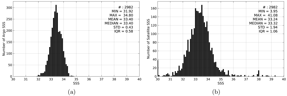
Figure 2: Histograms of SSS from Argo (a) and SMOS-L4-CATDS-CECOS-IFREMER-V2-WEEKLY-0.5DEG (b) considering all match-up pairs per bins of 0.1 over the South China Sea Pi-MEP region and for the full satellite product period.
