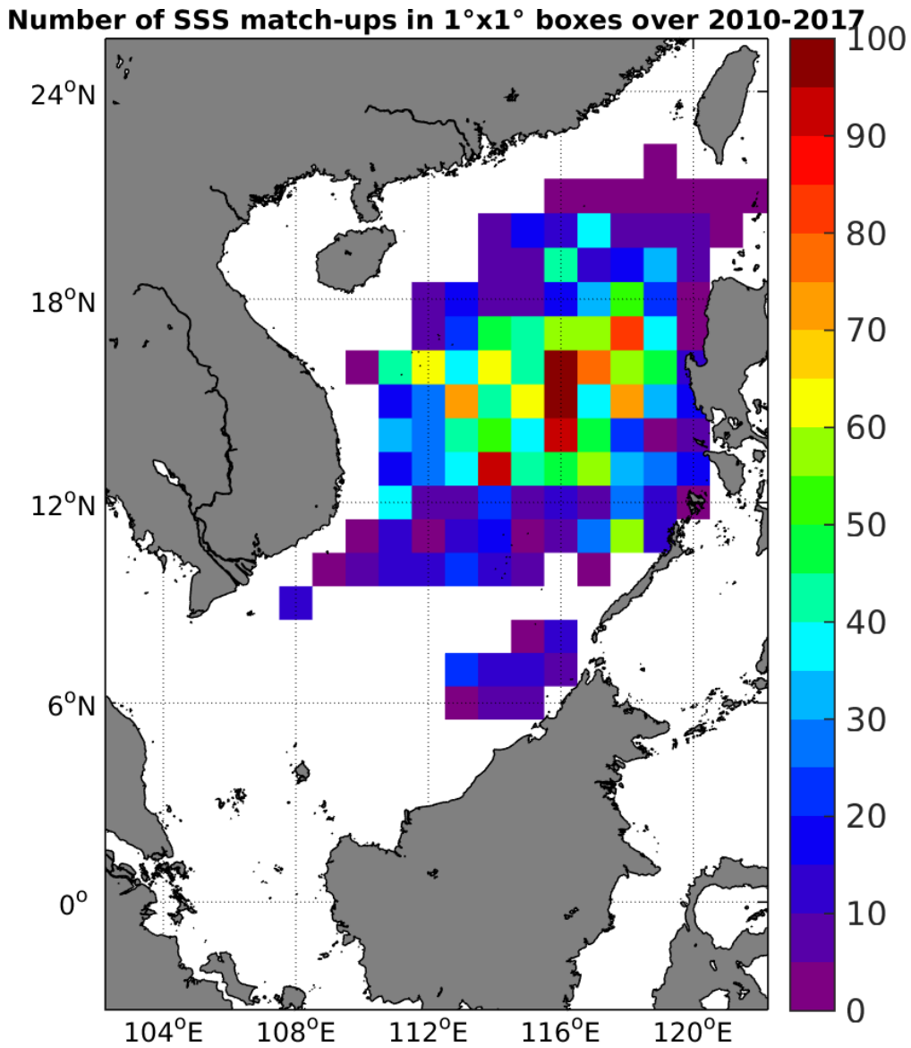
Figure 4: Number of SSS match-ups between Argo SSS and the SMOS-L4-CATDS-CECOS-IFREMER-V2-WEEKLY-0.5DEG SSS product for the South China Sea Pi-MEP region over 1°x1° boxes and for the full satellite product period.
