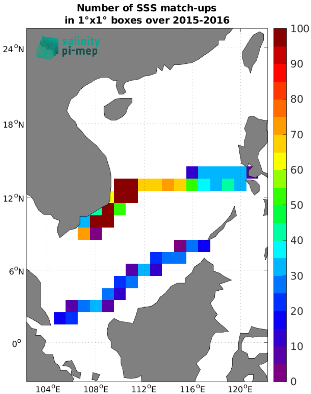
Figure 5: Number of SSS match-ups between TSG (SAMOS) SSS and the SMOS SSS L4 v2 - Daily (BEC) SSS product for the South China Sea Pi-MEP region over 1^{\circ} \times 1^{\circ} boxes and for the full satellite product period.
