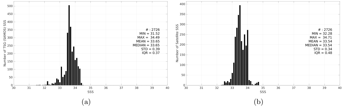
Figure 3: Histograms of SSS from TSG (SAMOS) (a) and SMOS SSS L4 v2 - Daily (BEC) (b) considering all match-up pairs per bins of 0.1 over the South China Sea Pi-MEP region and for the full satellite product period.
