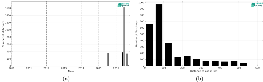
Figure 2: Number of match-ups between TSG (SAMOS) and SMOS SSS L4 v2 - Daily (BEC) SSS as a function of time (a) and as function of the distance to coast (b) over the South China Sea Pi-MEP region and for the full satellite product period.
