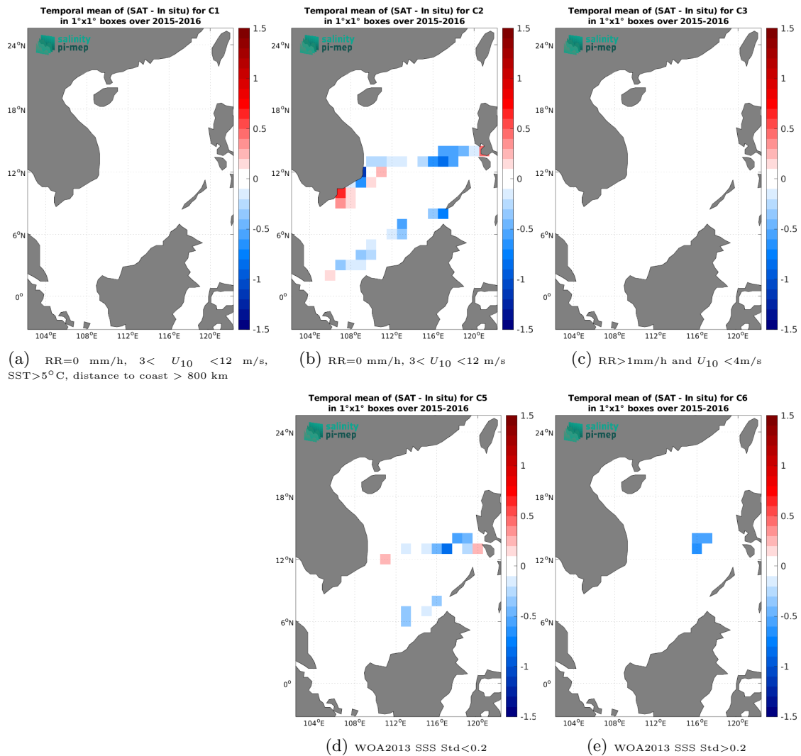
Figure 14: Temporal mean gridded over spatial boxes of size 1^\circ \times 1^\circ of \Delta\text{SSS} (SMOS SSS L4 v2 - Daily (BEC) - TSG (SAMOS)) for 5 different subdatasets corresponding to: RR=0 mm/h, 3 < U_{10} < 12 m/s, SST > 5^\circ\text{C} , distance to coast > 800 km (a), RR=0 mm/h, 3 < U_{10} < 12 m/s (b), RR > 1 mm/h and U_{10} < 4 m/s (c), WOA2013 SSS Std < 0.2 (d), WOA2013 SSS Std > 0.2 (e).
