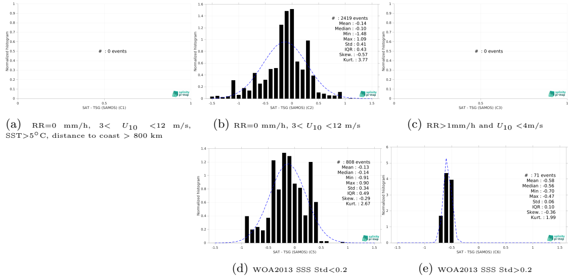
Figure 13: Normalized histogram of \Delta SSS (SMOS SSS L4 v2 - Daily (BEC) - TSG (SAMOS)) for 5 different subdatasets corresponding to: RR=0 mm/h, 3 < U_{10} < 12 m/s, SST>5°C, distance to coast > 800 km (a), RR=0 mm/h, 3 < U_{10} < 12 m/s (b), RR>1mm/h and U_{10} < 4 m/s (c), WOA2013 SSS Std<0.2 (d), WOA2013 SSS Std>0.2 (e).
