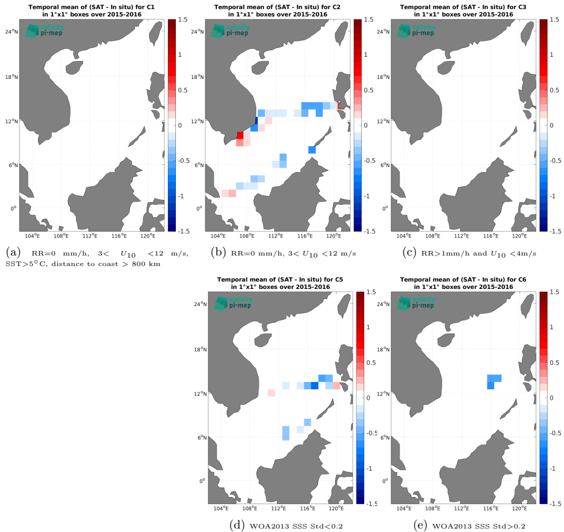
Figure 12: Temporal mean gridded over spatial boxes of size 1^\circ \times 1^\circ of \Delta\text{SSS} (SMOS SSS L4 v2 - Daily (BEC) - TSG (SAMOS)) for 5 different subdatasets corresponding to:RR=0 mm/h, 3 < U_{10} < 12 m/s, SST > 5^\circ\text{C} , distance to coast > 800 km (a), RR=0 mm/h, 3 < U_{10} < 12 m/s (b), RR > 1 mm/h and U_{10} < 4 m/s (c), WOA2013 SSS Std < 0.2 (d), WOA2013 SSS Std > 0.2 (e).
