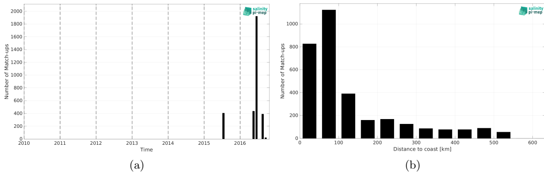
Figure 1: Number of match-ups between TSG (SAMOS) and SMOS SSS L4 v2 - Daily (BEC) SSS as a function of time (a) and as function of the distance to coast (b) over the South China Sea Pi-MEP region and for the full satellite product period.
