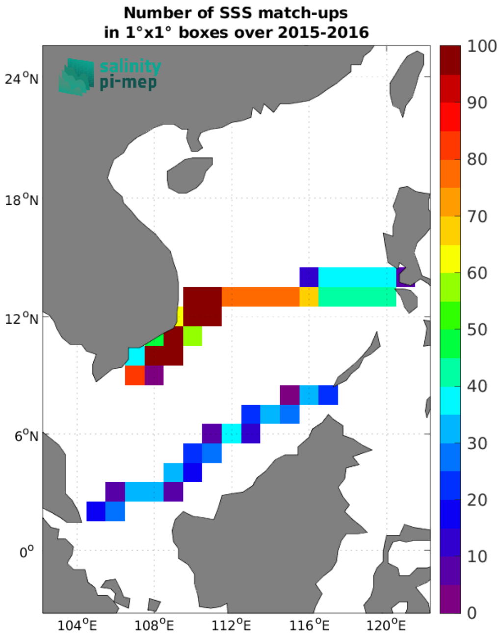
Figure 4: Number of SSS match-ups between TSG (SAMOS) SSS and the SMOS SSS L4 v2 - Daily (BEC) SSS product for the South China Sea Pi-MEP region over 1^{\circ} \times 1^{\circ} boxes and for the full satellite product period.
