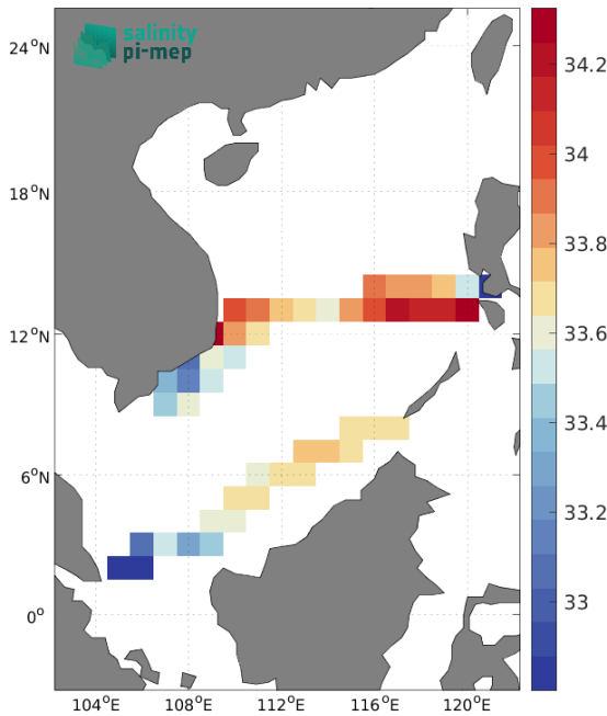
(c) MEAN(TSG (SAMOS) SSS)
