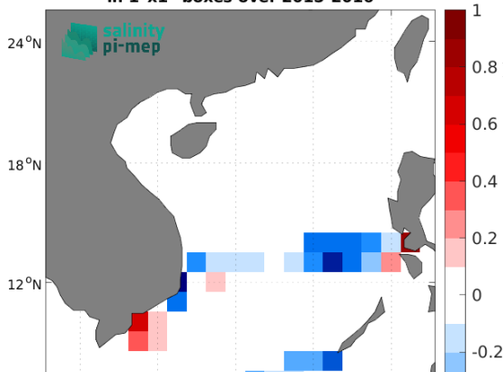
Temporal mean of (Sat - TSG (SAMOS)) in 1°x1° boxes over 2015-2016
