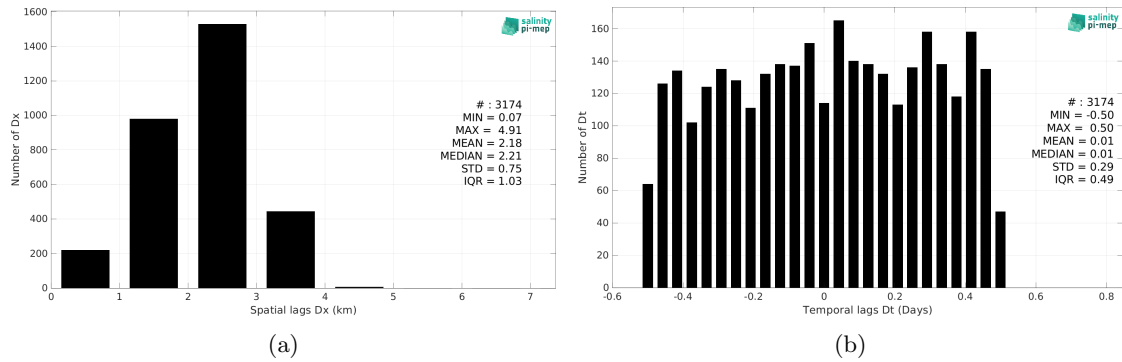
Figure 5: Histograms of the spatial (a) and temporal (b) lags between the location/time of the TSG (SAMOS) measurement and the date of the corresponding SMOS SSS L4 v2 - Daily (BEC) SSS pixel.
