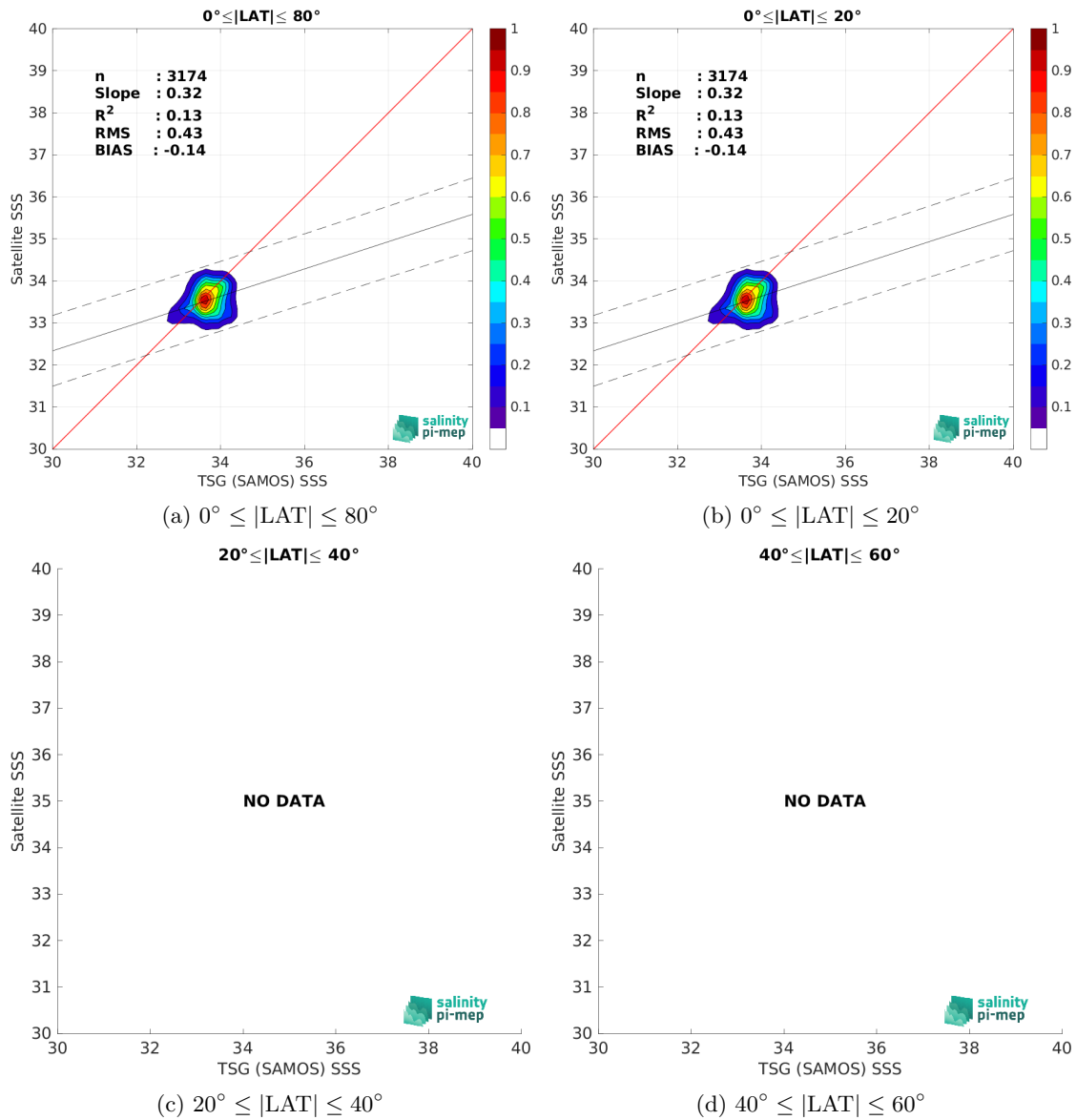
Figure 9: Contour maps of the concentration of SMOS SSS L4 v2 - Daily (BEC) SSS (y-axis) versus TSG (SAMOS) SSS (x-axis) at match-up pairs for different latitude bands. For each plot, the red line shows x=y . The black thin and dashed lines indicate a linear fit through the data cloud and the \pm 95\% confidence levels, respectively. The number match-up pairs n , the slope and R^2 coefficient of the linear fit, the root mean square (RMS) and the mean bias between satellite and in situ data are indicated for each latitude band in each plots.
