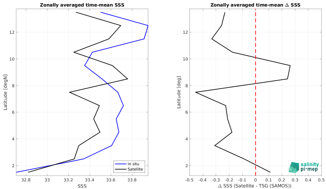
Figure 8: Left panel: Zonal mean SSS from SMOS SSS L4 v2 - Daily (BEC) satellite product (black) and from TSG (SAMOS) (blue). Right panel: Zonal mean of \Delta SSS (Satellite - TSG (SAMOS)) for all the collected Pi-MEP match-up pairs estimated over the full satellite product period.
