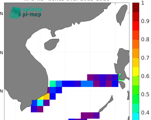
Temporal STD of (Sat - TSG (SAMOS)) in 1°x1° boxes over 2015-2016
