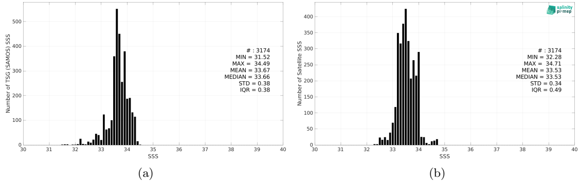
Figure 2: Histograms of SSS from TSG (SAMOS) (a) and SMOS SSS L4 v2 - Daily (BEC) (b) considering all match-up pairs per bins of 0.1 over the South China Sea Pi-MEP region and for the full satellite product period.
