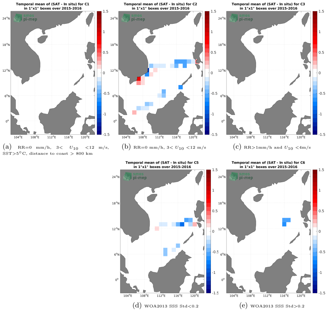
Figure 12: Temporal mean gridded over spatial boxes of size 1^\circ \times 1^\circ of \Delta SSS (SMOS SSS L4 v2 - Daily (BEC) - TSG (SAMOS)) for 5 different subdatasets corresponding to:RR=0 mm/h, 3 < U_{10} < 12 m/s, SST > 5°C, distance to coast > 800 km (a), RR=0 mm/h, 3 < U_{10} < 12 m/s (b), RR > 1mm/h and U_{10} < 4 m/s (c), WOA2013 SSS Std < 0.2 (d), WOA2013 SSS Std > 0.2 (e).
