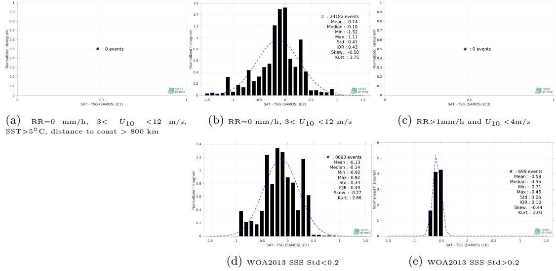
Figure 13: Normalized histogram of \Delta\text{SSS} (SMOS SSS L4 v2 - Daily (BEC) - TSG (SAMOS)) for 5 different subdatasets corresponding to: RR=0 mm/h, 3 < U_{10} < 12 m/s, SST>5°C, distance to coast > 800 km (a), RR=0 mm/h, 3 < U_{10} < 12 m/s (b), RR>1mm/h and U_{10} < 4 m/s (c), WOA2013 SSS Std<0.2 (d), WOA2013 SSS Std>0.2 (e).
