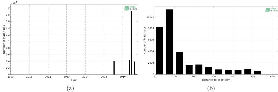
Figure 1: Number of match-ups between TSG (SAMOS) and SMOS SSS L4 v2 - Daily (BEC) SSS as a function of time (a) and as function of the distance to coast (b) over the South China Sea Pi-MEP region and for the full satellite product period.
