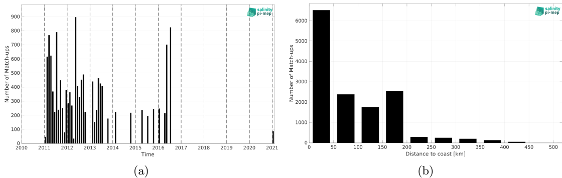
Figure 2: Number of match-ups between TSG (LEGOS-DM) and SMOS SSS L4 v2 - Daily (BEC) SSS as a function of time (a) and as function of the distance to coast (b) over the South China Sea Pi-MEP region and for the full satellite product period.
