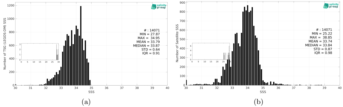
Figure 3: Histograms of SSS from TSG (LEGOS-DM) (a) and SMOS SSS L4 v2 - Daily (BEC) (b) considering all match-up pairs per bins of 0.1 over the South China Sea Pi-MEP region and for the full satellite product period.
