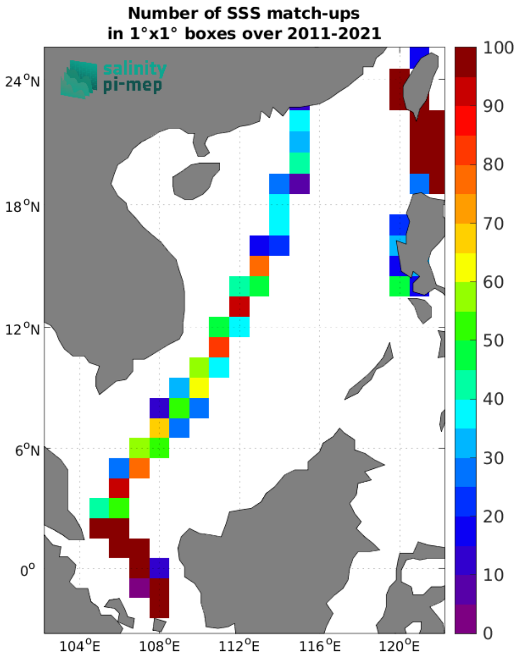
Figure 5: Number of SSS match-ups between TSG (LEGOS-DM) SSS and the SMOS SSS L4 v2 - Daily (BEC) SSS product for the South China Sea Pi-MEP region over 1°x1° boxes and for the full satellite product period.
