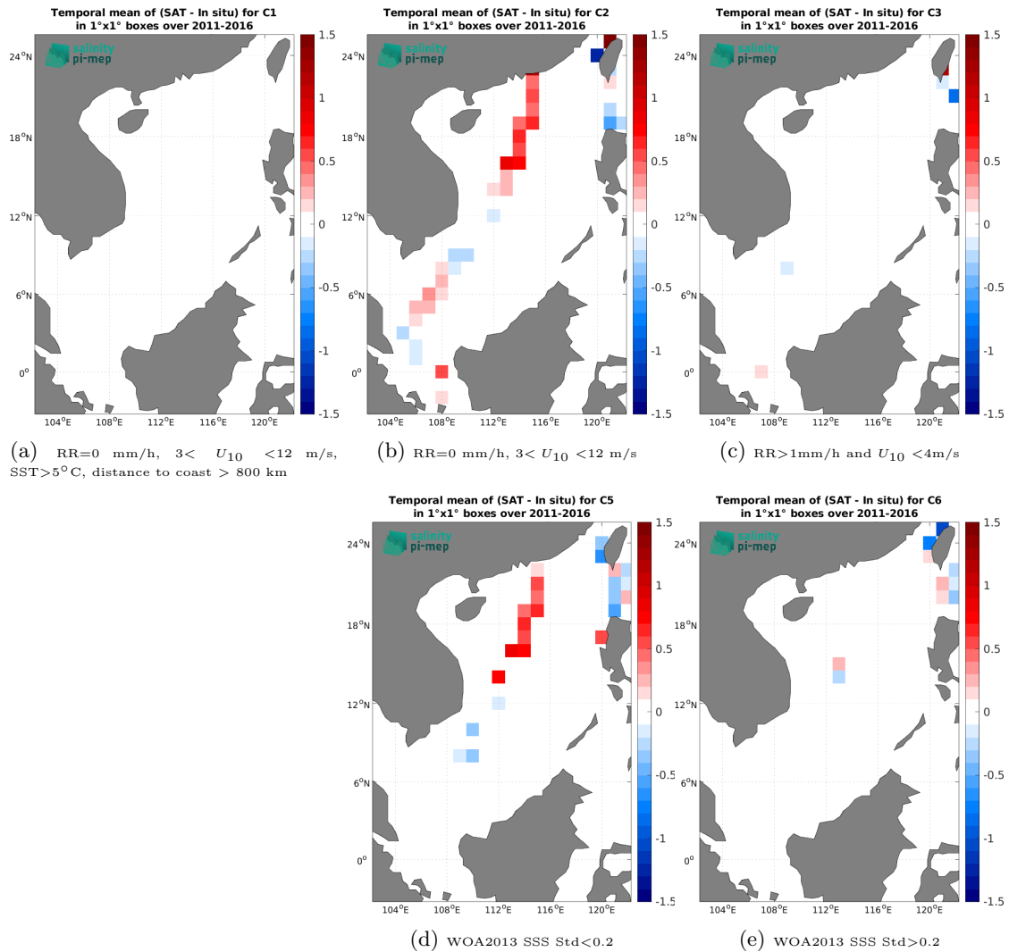
Figure 12: Temporal mean gridded over spatial boxes of size 1^\circ \times 1^\circ of \Delta\text{SSS} (SMOS SSS L4 v2 - Daily (BEC) - TSG (LEGOS-DM)) for 5 different subdatasets corresponding to:RR=0 mm/h, 3 < U_{10} < 12 m/s, SST>5°C, distance to coast > 800 km (a), RR=0 mm/h, 3 < U_{10} < 12 m/s (b), RR>1mm/h and U_{10} < 4 m/s (c), WOA2013 SSS Std<0.2 (d), WOA2013 SSS Std>0.2 (e).
