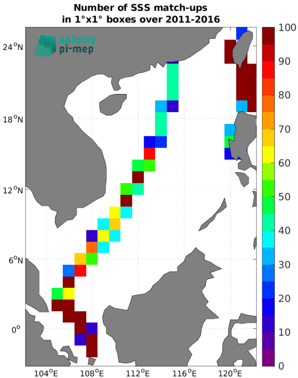
Figure 4: Number of SSS match-ups between TSG (LEGOS-DM) SSS and the SMOS SSS L4 v2 - Daily (BEC) SSS product for the South China Sea Pi-MEP region over 1^\circ \times 1^\circ boxes and for the full satellite product period.
