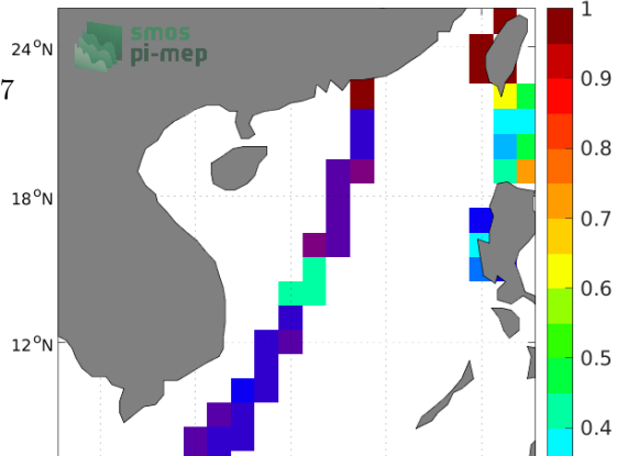
Temporal STD of (Sat - TSG (LEGOS-DM)) in 1°x1° boxes over 2011-2016
