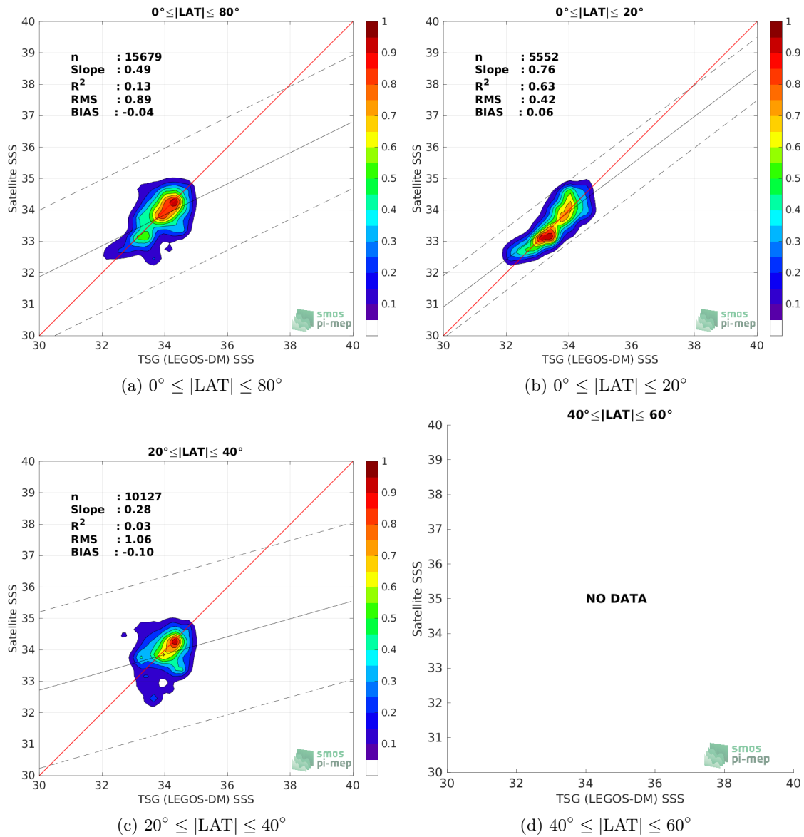
Figure 9: Contour maps of the concentration of SMOS SSS L4 v2 - Daily (BEC) SSS (y-axis) versus TSG (LEGOS-DM) SSS (x-axis) at match-up pairs for different latitude bands. For each plot, the red line shows x=y . The black thin and dashed lines indicate a linear fit through the data cloud and the \pm 95\% confidence levels, respectively. The number match-up pairs n , the slope and R^2 coefficient of the linear fit, the root mean square (RMS) and the mean bias between satellite and in situ data are indicated for each latitude band in each plots.
