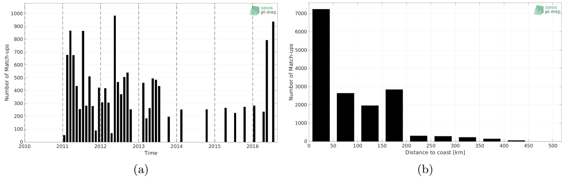
Figure 1: Number of match-ups between TSG (LEGOS-DM) and SMOS SSS L4 v2 - Daily (BEC) SSS as a function of time (a) and as function of the distance to coast (b) over the South China Sea Pi-MEP region and for the full satellite product period.
