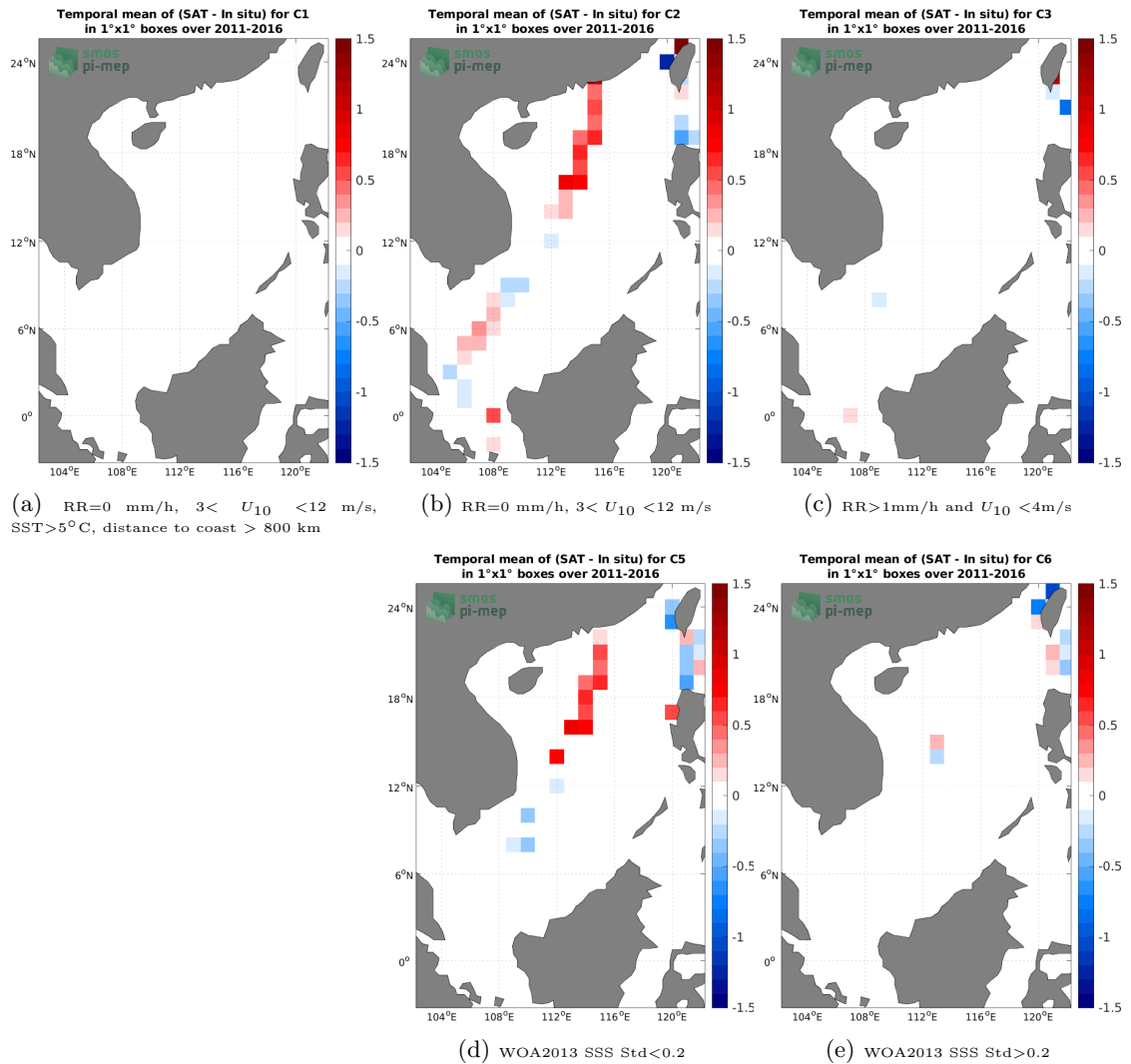
Figure 12: Temporal mean gridded over spatial boxes of size 1^\circ \times 1^\circ of \Delta SSS (SMOS SSS L4 v2 - Daily (BEC) - TSG (LEGOS-DM)) for 5 different subdatasets corresponding to:RR=0 mm/h, 3 < U_{10} < 12 m/s, SST>5°C, distance to coast > 800 km (a), RR=0 mm/h, 3 < U_{10} < 12 m/s (b), RR>1mm/h and U_{10} < 4 m/s (c), WOA2013 SSS Std<0.2 (d), WOA2013 SSS Std>0.2 (e).
