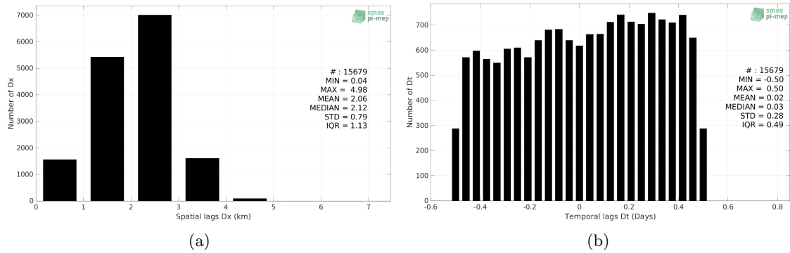
Figure 5: Histograms of the spatial (a) and temporal (b) lags between the location/time of the TSG (LEGOS-DM) measurement and the date of the corresponding SMOS SSS L4 v2 - Daily (BEC) SSS pixel.
