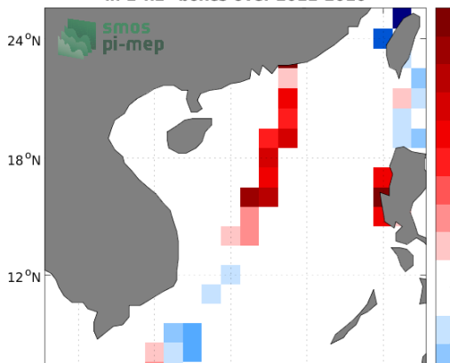
Temporal mean of (Sat - TSG (LEGOS-DM)) in 1°x1° boxes over 2011-2016
