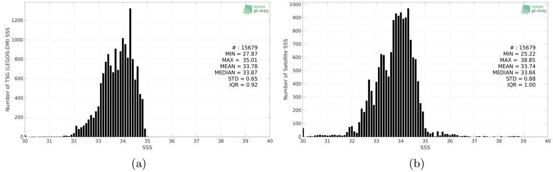
Figure 2: Histograms of SSS from TSG (LEGOS-DM) (a) and SMOS SSS L4 v2 - Daily (BEC) (b) considering all match-up pairs per bins of 0.1 over the South China Sea Pi-MEP region and for the full satellite product period.
