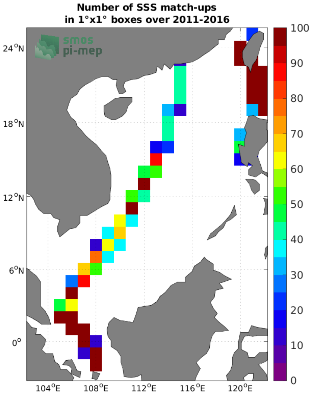
Figure 4: Number of SSS match-ups between TSG (LEGOS-DM) SSS and the SMOS SSS L4 v2 - Daily (BEC) SSS product for the South China Sea Pi-MEP region over 1°×1° boxes and for the full satellite product period.
