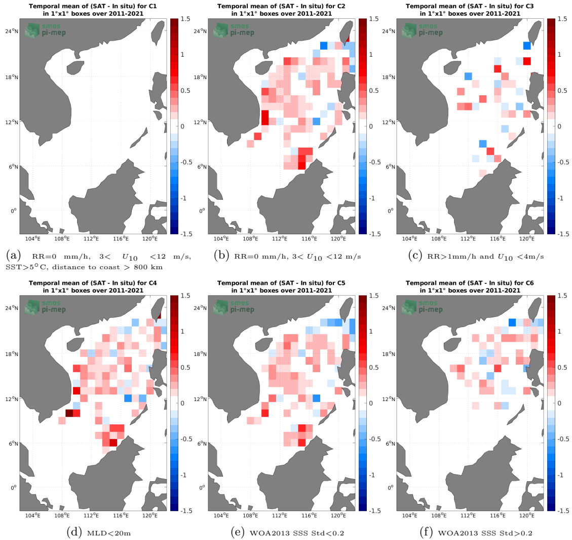
Figure 12: Temporal mean gridded over spatial boxes of size 1^\circ \times 1^\circ of \Delta SSS (SMOS SSS L4 v2 - Daily (BEC) - Argo) for 6 different subdatasets corresponding to:RR=0 mm/h, 3 < U_{10} < 12 m/s, SST>5°C, distance to coast > 800 km (a), RR=0 mm/h, 3 < U_{10} < 12 m/s (b), RR>1mm/h and U_{10} < 4 m/s (c),MLD<20m (d),WOA2013 SSS Std<0.2 (e),WOA2013 SSS Std>0.2 (f).
