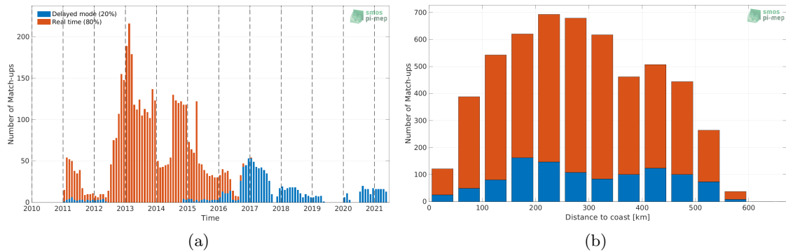
Figure 1: Number of match-ups between Argo and SMOS SSS L4 v2 - Daily (BEC) SSS as a function of time (a) and as function of the distance to coast (b) over the South China Sea Pi-MEP region and for the full satellite product period.
