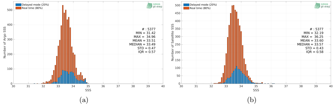
Figure 2: Histograms of SSS from Argo (a) and SMOS SSS L4 v2 - Daily (BEC) (b) considering all match-up pairs per bins of 0.1 over the South China Sea Pi-MEP region and for the full satellite product period.
