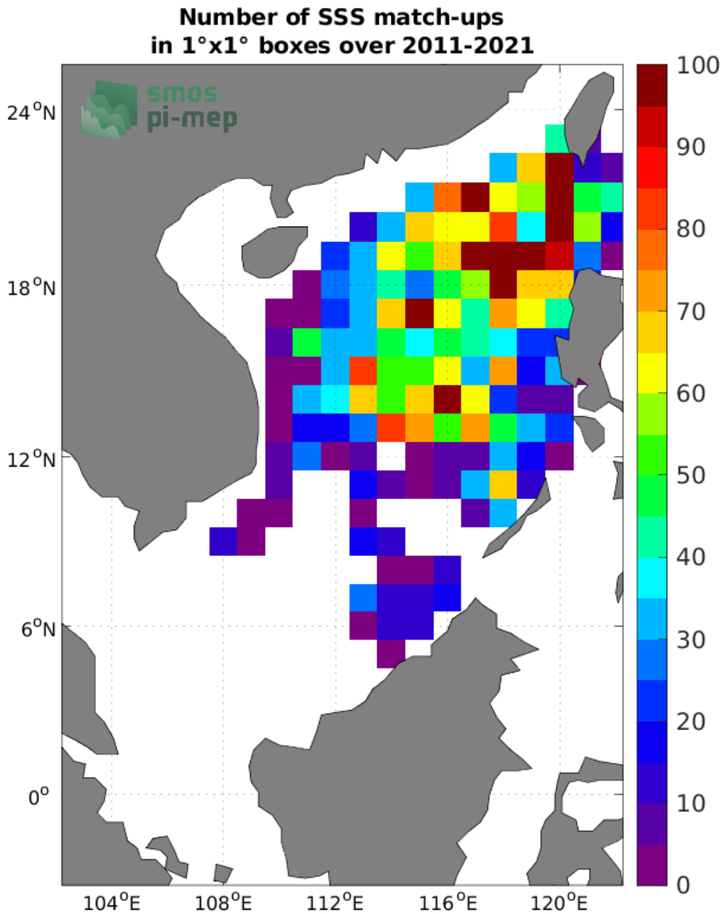
Figure 4: Number of SSS match-ups between Argo SSS and the SMOS SSS L4 v2 - Daily (BEC) SSS product for the South China Sea Pi-MEP region over 1°×1° boxes and for the full satellite product period.
