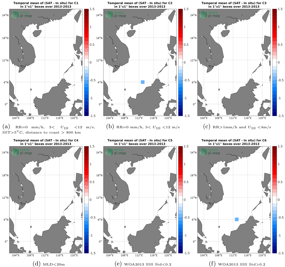
Figure 12: Temporal mean gridded over spatial boxes of size 1^\circ \times 1^\circ of \Delta SSS (SMOS SSS L3 v3 Monthly (ICDC) - Argo) for 6 different subdatasets corresponding to:RR=0 mm/h, 3 < U_{10} < 12 m/s, SST>5°C, distance to coast > 800 km (a), RR=0 mm/h, 3 < U_{10} < 12 m/s (b), RR>1mm/h and U_{10} < 4 m/s (c),MLD<20m (d),WOA2013 SSS Std<0.2 (e),WOA2013 SSS Std>0.2 (f).
