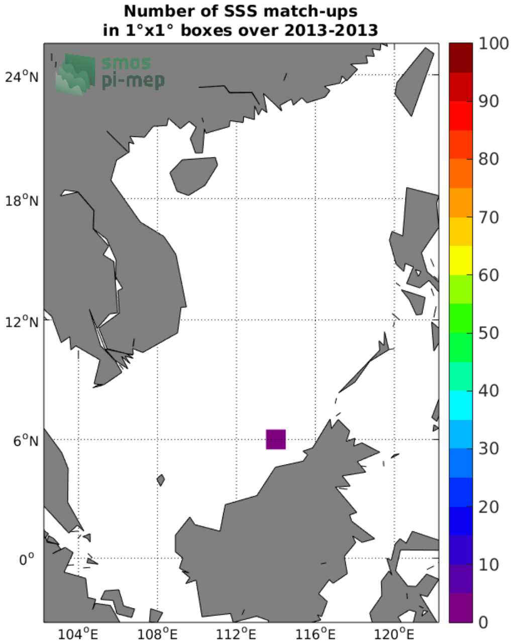
Figure 4: Number of SSS match-ups between Argo SSS and the SMOS SSS L3 v3 Monthly (ICDC) SSS product for the South China Sea Pi-MEP region over 1^\circ \times 1^\circ boxes and for the full satellite product period.
