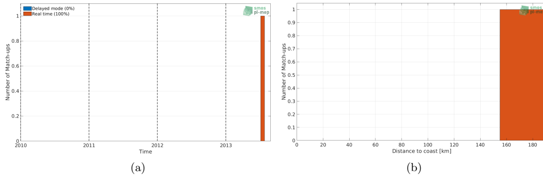
Figure 1: Number of match-ups between Argo and SMOS SSS L3 v3 Monthly (ICDC) SSS as a function of time (a) and as function of the distance to coast (b) over the South China Sea Pi-MEP region and for the full satellite product period.
