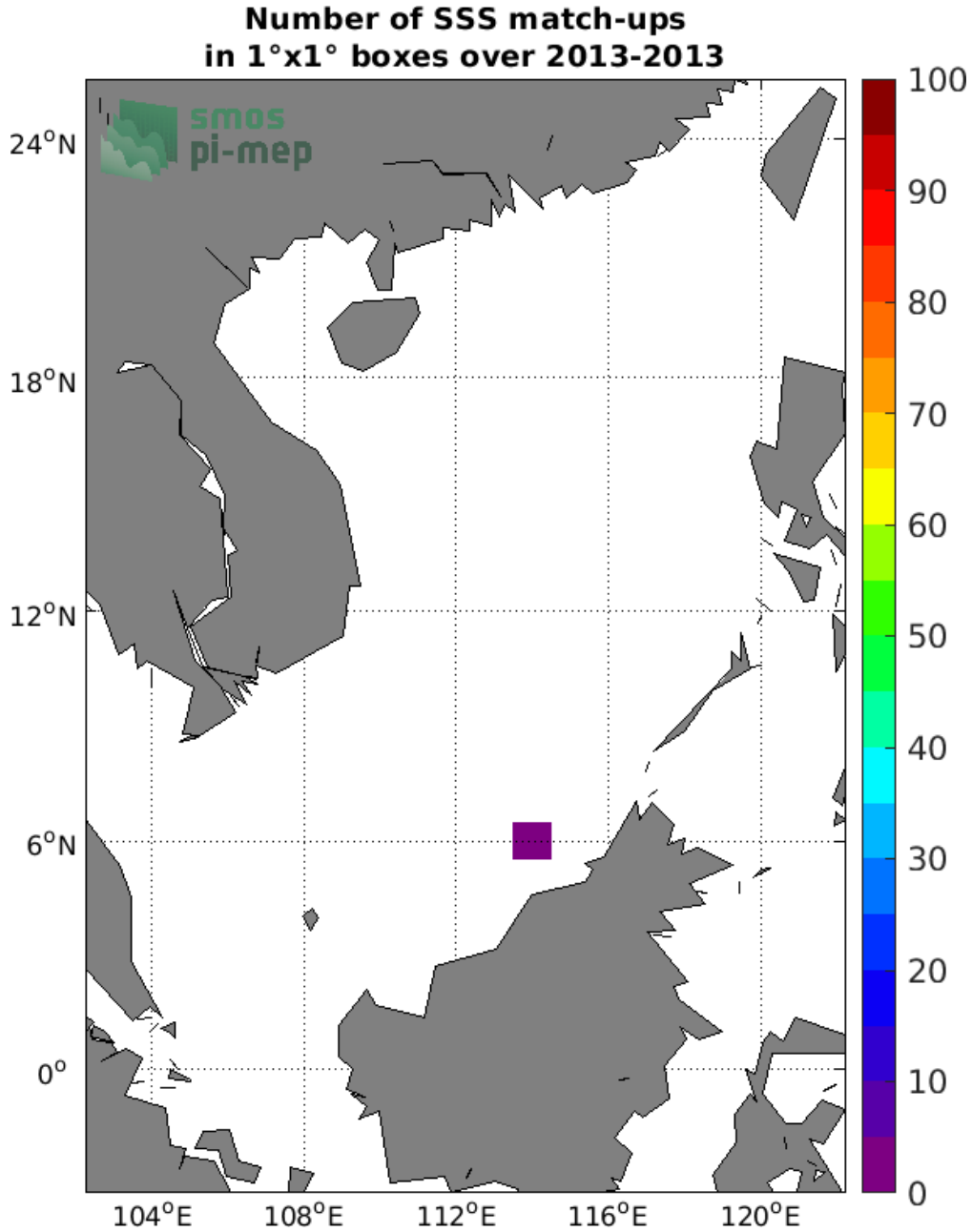
Figure 4: Number of SSS match-ups between Argo SSS and the SMOS SSS L3 v3 Monthly (ICDC) SSS product for the South China Sea Pi-MEP region over 1°x1° boxes and for the full satellite product period.
