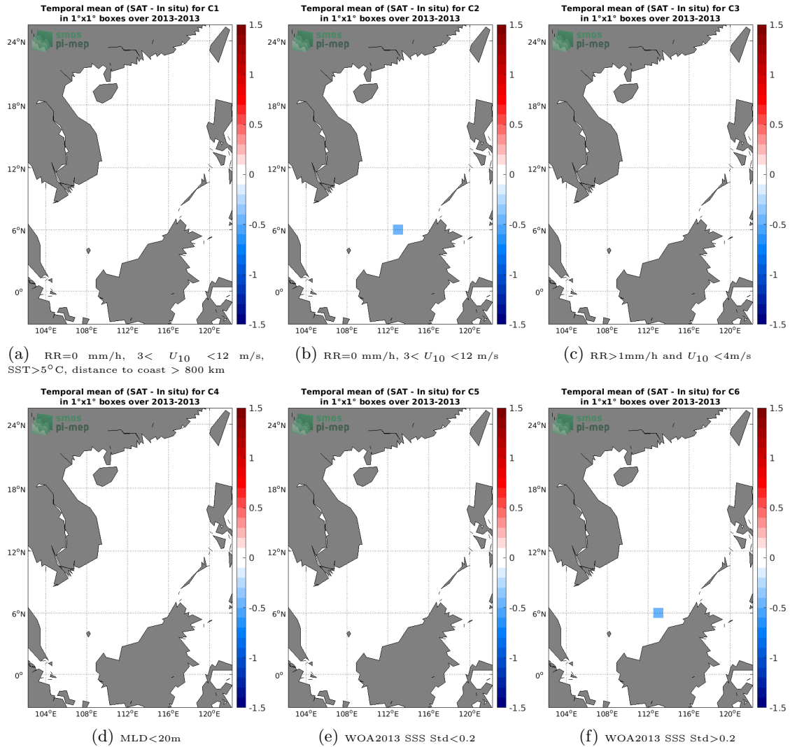
Figure 12: Temporal mean gridded over spatial boxes of size 1°x1° of \Delta SSS (SMOS SSS L3 v3 Monthly (ICDC) - Argo) for 6 different subdatasets corresponding to:RR=0 mm/h, 3 < U_{10} < 12 m/s, SST>5°C, distance to coast > 800 km (a), RR=0 mm/h, 3 < U_{10} < 12 m/s (b), RR>1mm/h and U_{10} < 4 m/s (c),MLD<20m (d),WOA2013 SSS Std<0.2 (e),WOA2013 SSS Std>0.2 (f).
