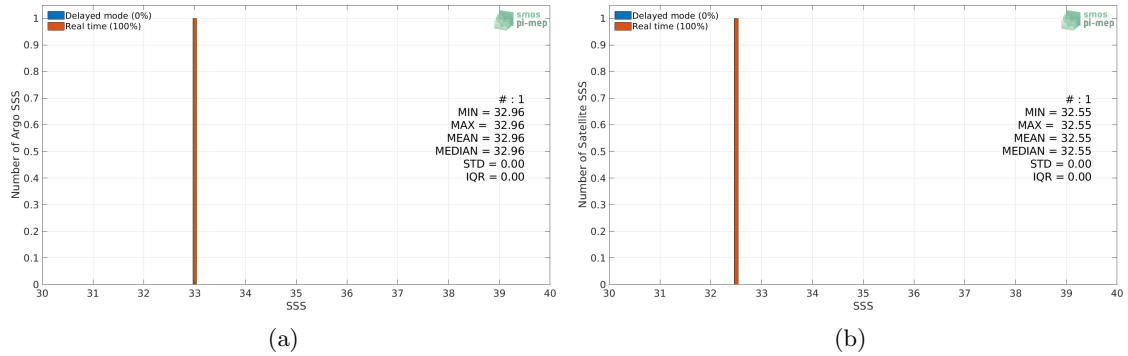
Figure 2: Histograms of SSS from Argo (a) and SMOS SSS L3 v3 Monthly (ICDC) (b) considering all match-up pairs per bins of 0.1 over the South China Sea Pi-MEP region and for the full satellite product period.
