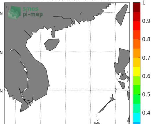
Temporal STD of (Sat - Argo) in 1°x1° boxes over 2013-2013
