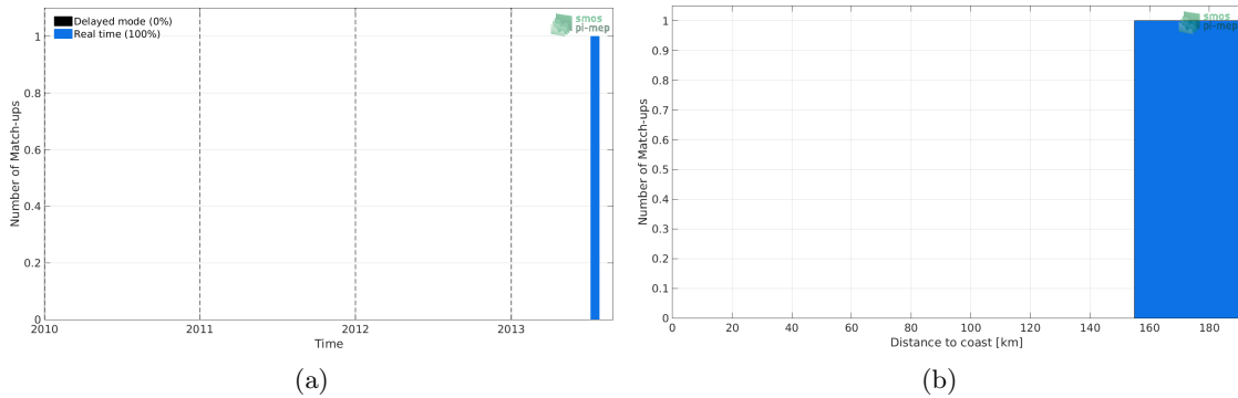
Figure 1: Number of match-ups between Argo and SMOS-L3-ICDC-V3-MONTHLY-0.5DEG SSS as a function of time (a) and as function of the distance to coast (b) over the South China Sea Pi-MEP region and for the full satellite product period.
