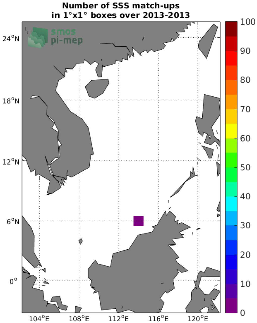
Figure 4: Number of SSS match-ups between Argo SSS and the SMOS-L3-ICDC-V3-MONTHLY-0.5DEG SSS product for the South China Sea Pi-MEP region over 1°x1° boxes and for the full satellite product period.
