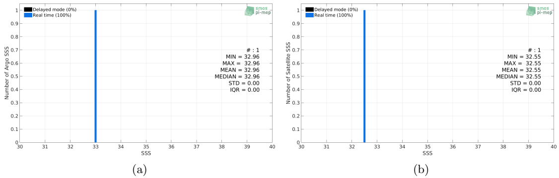
Figure 2: Histograms of SSS from Argo (a) and SMOS-L3-ICDC-V3-MONTHLY-0.5DEG (b) considering all match-up pairs per bins of 0.1 over the South China Sea Pi-MEP region and for the full satellite product period.
