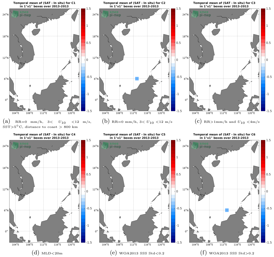
Figure 12: Temporal mean gridded over spatial boxes of size 1°x1° of \Delta SSS (SMOS-L3-ICDC-V3-MONTHLY-0.5DEG - Argo) for 6 different subdatasets corresponding to:RR=0 mm/h, 3 < U_{10} < 12 m/s, SST>5°C, distance to coast > 800 km (a), RR=0 mm/h, 3 < U_{10} < 12 m/s (b), RR>1mm/h and U_{10} < 4 m/s (c),MLD<20m (d),WOA2013 SSS Std<0.2 (e),WOA2013 SSS Std>0.2 (f).
