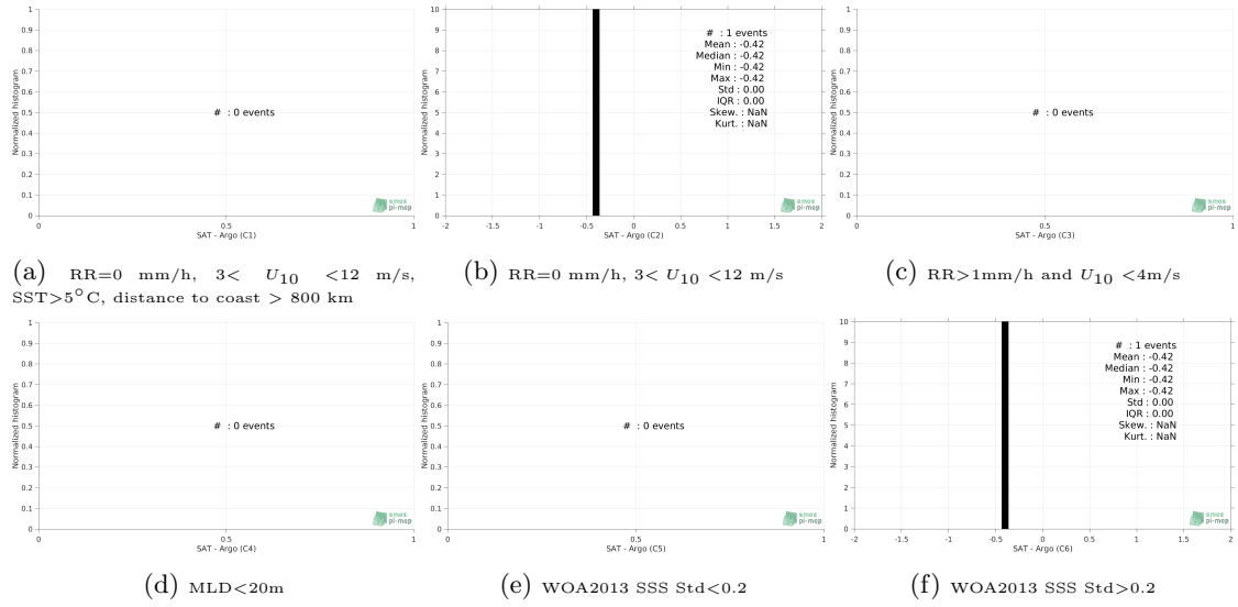
Figure 13: Normalized histogram of \Delta\text{SSS} (SMOS-L3-ICDC-V3-MONTHLY-0.5DEG - Argo) for 6 different subdatasets corresponding to: RR=0 mm/h, 3 < U_{10} < 12 m/s, SST>5°C, distance to coast > 800 km (a), RR=0 mm/h, 3 < U_{10} < 12 m/s (b), RR>1mm/h and U_{10} < 4 m/s (c), MLD<20m (d), WOA2013 SSS Std<0.2 (e), WOA2013 SSS Std>0.2 (f).
