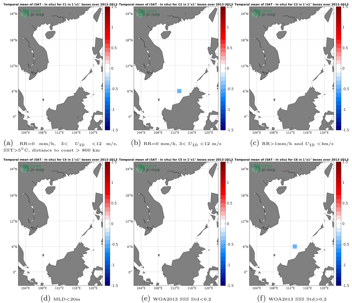
Figure 12: Temporal mean gridded over spatial boxes of size 1^\circ \times 1^\circ of \Delta SSS (SMOS-L3-ICDC-V3-MONTHLY-0.5DEG - Argo) for 6 different subdatasets corresponding to:RR=0 mm/h, 3 < U_{10} < 12 m/s, SST >5^\circ C, distance to coast > 800 km (a), RR=0 mm/h, 3 < U_{10} < 12 m/s (b), RR >1 mm/h and U_{10} < 4 m/s (c),MLD <20 m (d),WOA2013 SSS Std <0.2 (e),WOA2013 SSS Std >0.2 (f).
