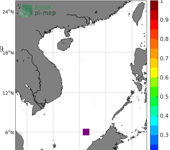
Temporal STD of (Sat-Argo) in 1°x1° boxes over 2013-2013
