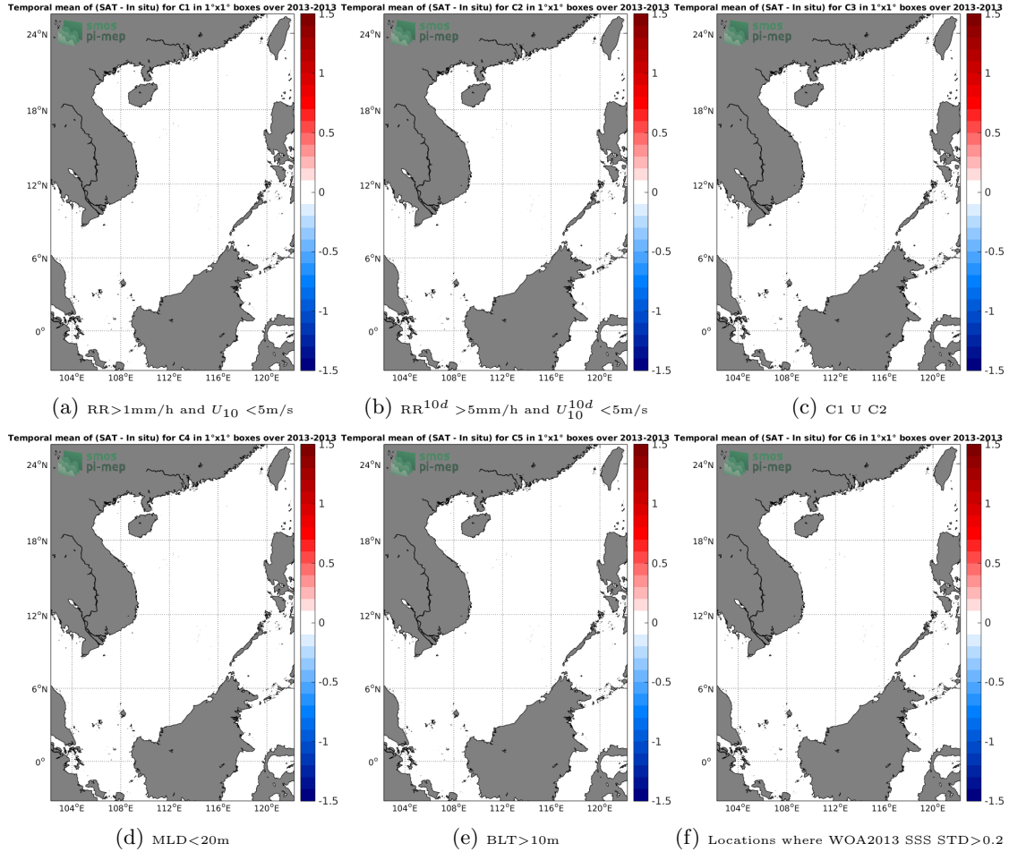
Figure 12: Temporal mean gridded over spatial boxes of size 1°x1° of \Delta SSS (SMOS-L3-ICDC-V3-MONTHLY-0.5DEG - Argo) for 6 different subdatasets corresponding to: RR > 1\text{mm/h} and U_{10} < 5\text{m/s} (a), RR^{10d} > 5\text{mm/h} and U_{10}^{10d} < 5\text{m/s} (b), C1 U C2 (c), MLD < 20\text{m} (d), BLT > 10\text{m} (e), Locations where WOA2013 SSS STD > 0.2 (f).
