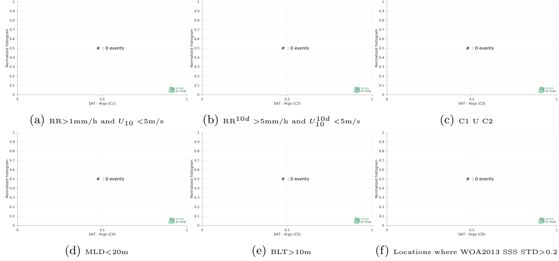
Figure 13: Normalized histogram of \Delta\text{SSS} (SMOS-L3-ICDC-V3-MONTHLY-0.5DEG - Argo) for 6 different subdatasets corresponding to: RR > 1\text{mm/h} and U_{10} < 5\text{m/s} (a), RR^{10d} > 5\text{mm/h} and U_{10}^{10d} < 5\text{m/s} (b), C1 U C2 (c), MLD < 20\text{m} (d), BLT > 10\text{m} (e), Locations where WOA2013 SSS STD > 0.2 (f).
