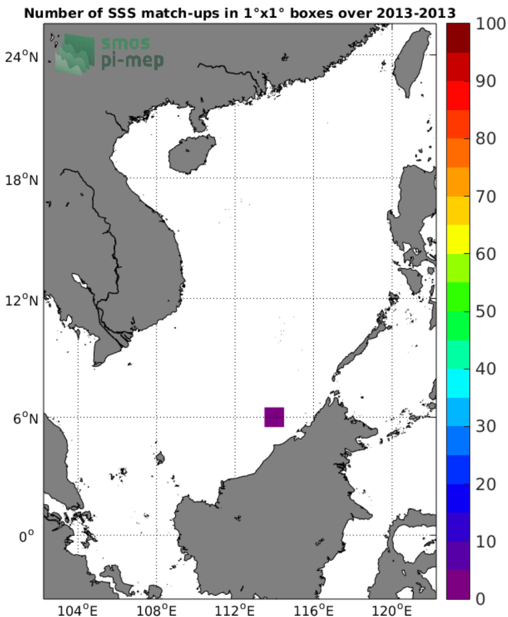
Figure 4: Number of SSS match-ups between Argo SSS and the SMOS-L3-ICDC-V3-MONTHLY-0.5DEG SSS product for the South China Sea Pi-MEP region over 1°x1° boxes and for the full satellite product period.
