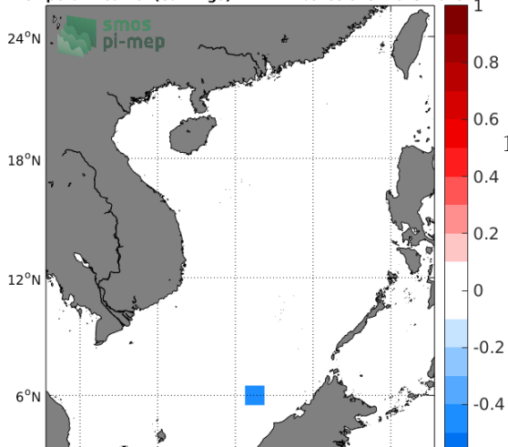
Temporal mean of (Sat-Argo) in 1°x1° boxes over 2013-2013
