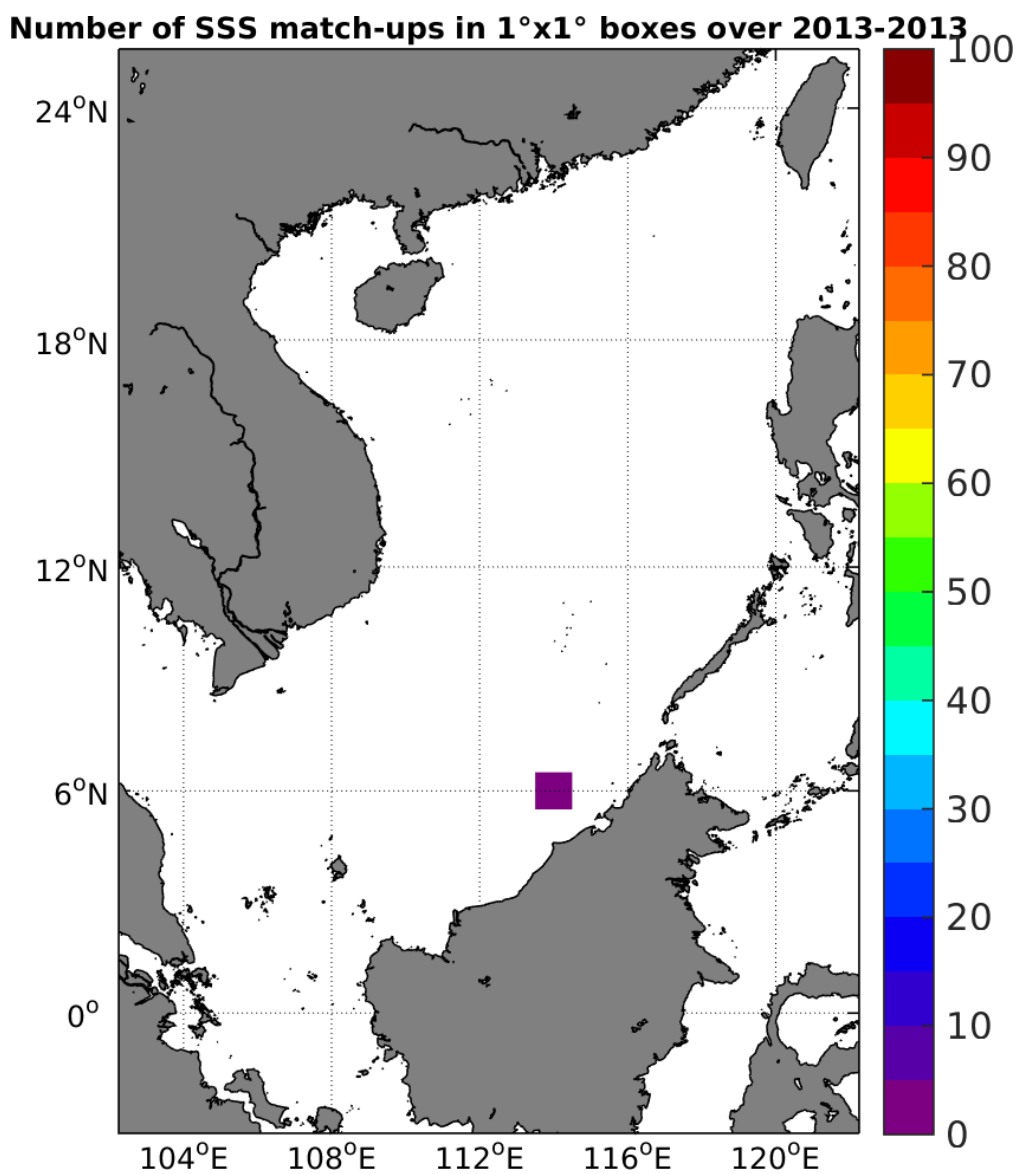
Figure 4: Number of SSS match-ups between Argo SSS and the SMOS-L3-ICDC-V3-MONTHLY-0.5DEG SSS product for the South China Sea Pi-MEP region over 1°x1° boxes and for the full satellite product period.
