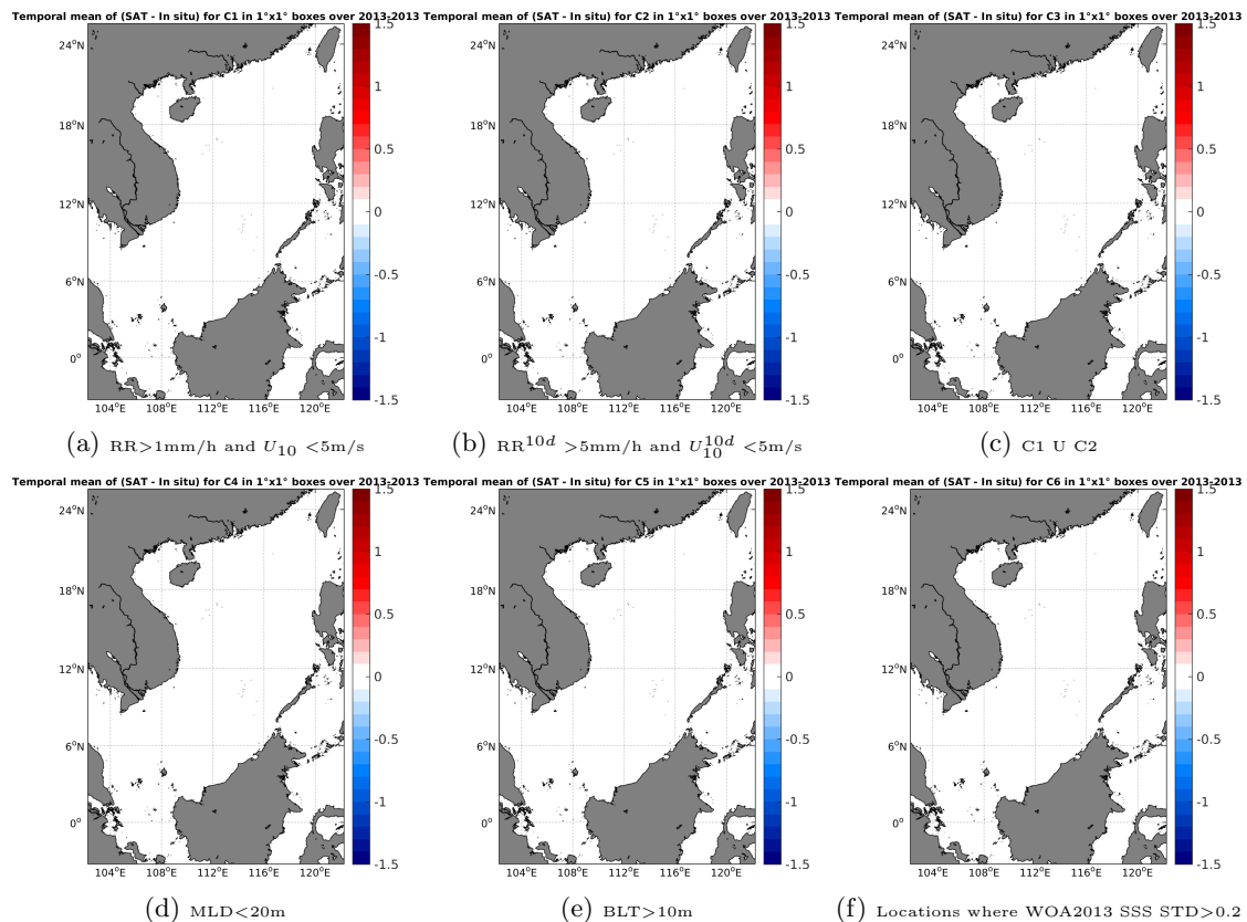
Figure 12: Temporal mean gridded over spatial boxes of size 1^\circ \times 1^\circ of \Delta SSS (SMOS-L3-ICDC-V3-MONTHLY-0.5DEG - Argo) for 6 different subdatasets corresponding to: RR > 1\text{mm/h} and U_{10} < 5\text{m/s} (a), RR^{10d} > 5\text{mm/h} and U_{10}^{10d} < 5\text{m/s} (b), C1 U C2 (c), MLD < 20\text{m} (d), BLT > 10\text{m} (e), Locations where WOA2013 SSS STD > 0.2 (f).
