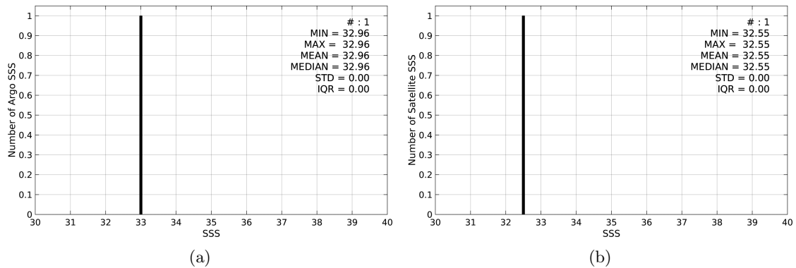
Figure 2: Histograms of SSS from Argo (a) and SMOS-L3-ICDC-V3-MONTHLY-0.5DEG (b) considering all match-up pairs per bins of 0.1 over the South China Sea Pi-MEP region and for the full satellite product period.
