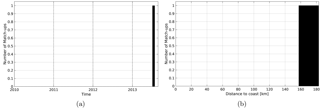
Figure 1: Number of match-ups between Argo and SMOS-L3-ICDC-V3-MONTHLY-0.5DEG SSS as a function of time (a) and as function of the distance to coast (b) over the South China Sea Pi-MEP region and for the full satellite product period.
