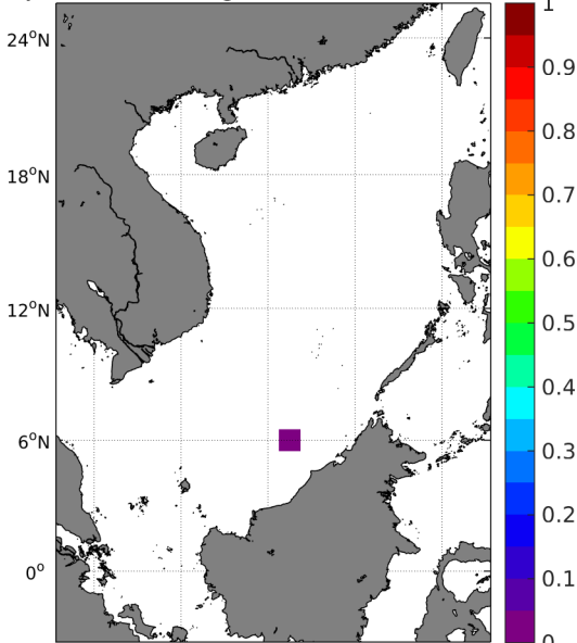
Temporal STD of (Sat-Argo) in 1°x1° boxes over 2013-2013
