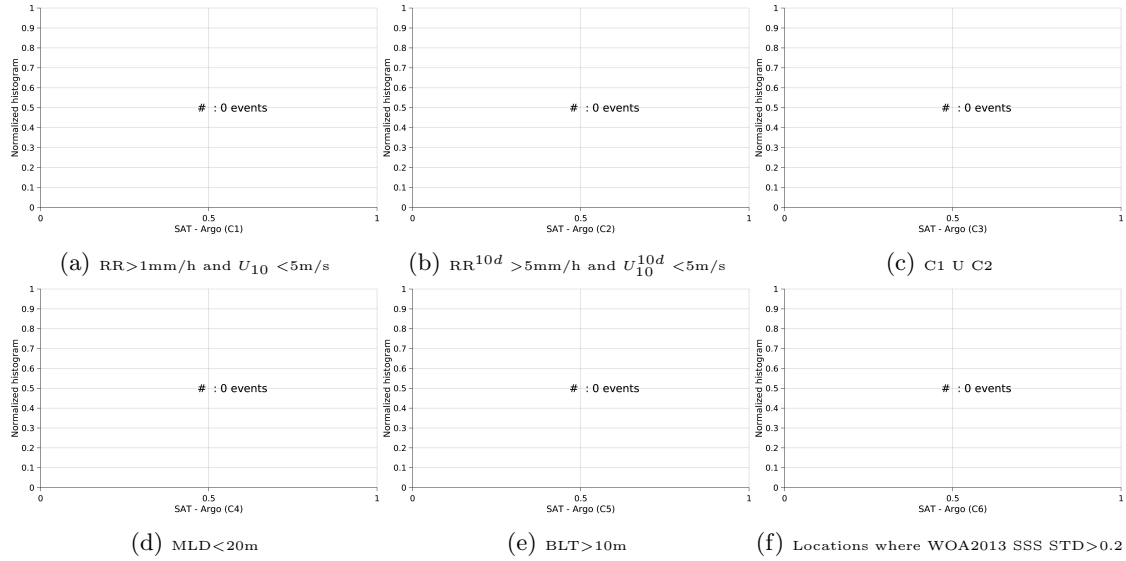
Figure 13: Normalized histogram of \Delta\text{SSS} (SMOS-L3-ICDC-V3-MONTHLY-0.5DEG - Argo) for 6 different subdatasets corresponding to: RR > 1\text{mm/h} and U_{10} < 5\text{m/s} (a), RR^{10d} > 5\text{mm/h} and U_{10}^{10d} < 5\text{m/s} (b), C1 U C2 (c), MLD < 20\text{m} (d), BLT > 10\text{m} (e), Locations where WOA2013 SSS STD > 0.2 (f).
