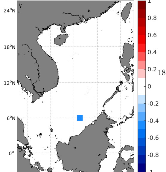
Temporal mean of (Sat-Argo) in 1°x1° boxes over 2013-2013
