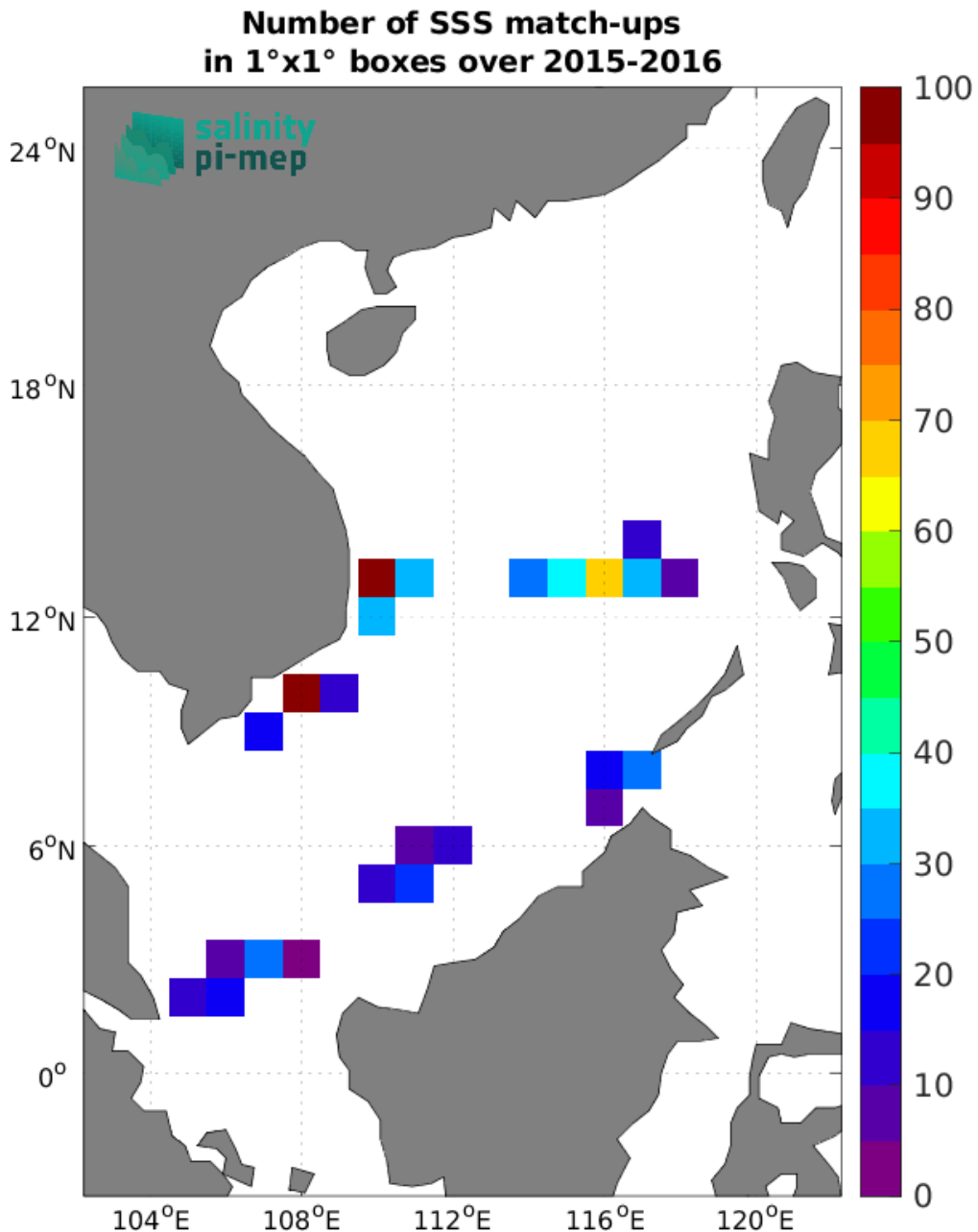
Figure 5: Number of SSS match-ups between TSG (SAMOS) SSS and the SMOS SSS L2Q v331 - With FLAG (CMEMS-CATDS-CPDC) SSS product for the South China Sea Pi-MEP region over 1°×1° boxes and for the full satellite product period.
