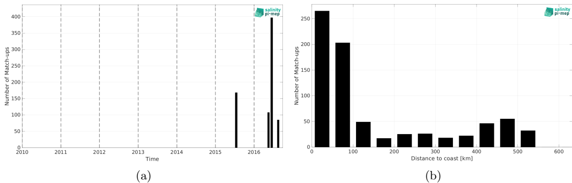
Figure 2: Number of match-ups between TSG (SAMOS) and SMOS SSS L2Q v331 - With FLAG (CMEMS-CATDS-CPDC) SSS as a function of time (a) and as function of the distance to coast (b) over the South China Sea Pi-MEP region and for the full satellite product period.
