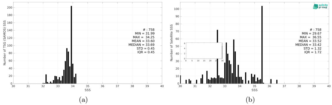
Figure 3: Histograms of SSS from TSG (SAMOS) (a) and SMOS SSS L2Q v331 - With FLAG (CMEMS-CATDS-CPDC) (b) considering all match-up pairs per bins of 0.1 over the South China Sea Pi-MEP region and for the full satellite product period.
