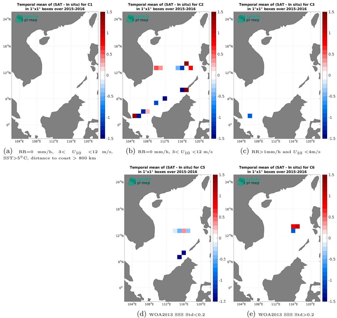
Figure 14: Temporal mean gridded over spatial boxes of size 1^\circ \times 1^\circ of \Delta\text{SSS} (SMOS SSS L2Q v331 - With FLAG (CMEMS-CATDS-CPDC) - TSG (SAMOS)) for 5 different subdatasets corresponding to: RR=0 mm/h, 3 < U_{10} < 12 m/s, SST > 5^\circ\text{C} , distance to coast > 800 km (a), RR=0 mm/h, 3 < U_{10} < 12 m/s (b), RR > 1 mm/h and U_{10} < 4 m/s (c), WOA2013 SSS Std < 0.2 (d), WOA2013 SSS Std > 0.2 (e).
