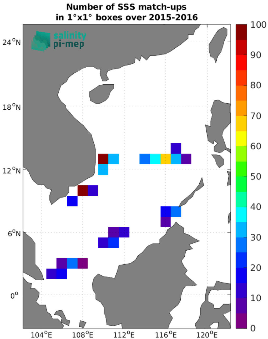
Figure 4: Number of SSS match-ups between TSG (SAMOS) SSS and the SMOS SSS L2Q v331 - With FLAG (CMEMS-CATDS-CPDC) SSS product for the South China Sea Pi-MEP region over 1°x1° boxes and for the full satellite product period.
