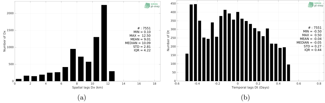
Figure 5: Histograms of the spatial (a) and temporal (b) lags between the location/time of the TSG (SAMOS) measurement and the date of the corresponding SMOS SSS L2Q v331 - With FLAG (CMEMS-CATDS-CPDC) SSS pixel.
