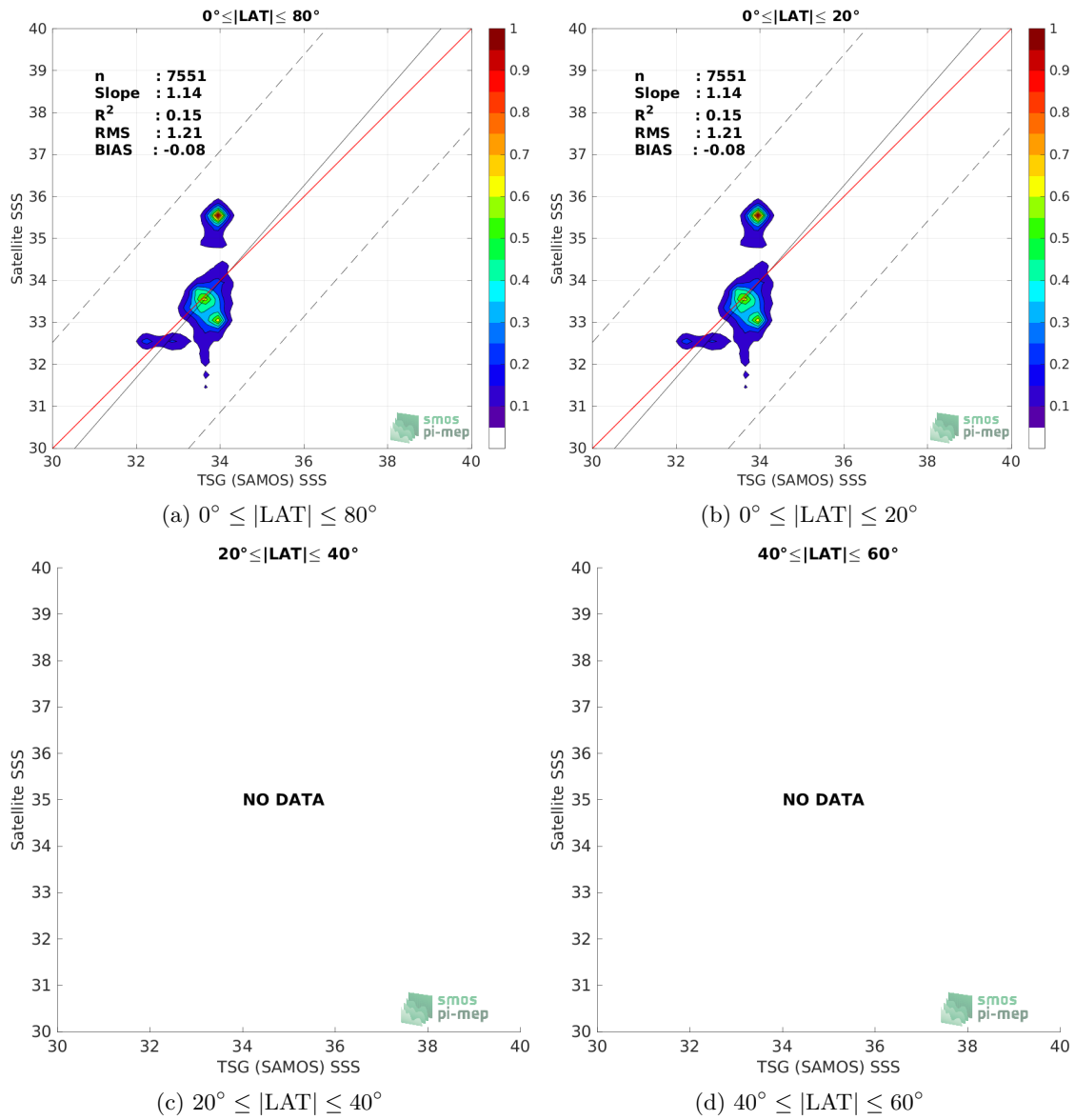
Figure 9: Contour maps of the concentration of SMOS SSS L2Q v331 - With FLAG (CMEMS-CATDS-CPDC) SSS (y-axis) versus TSG (SAMOS) SSS (x-axis) at match-up pairs for different latitude bands. For each plot, the red line shows x=y . The black thin and dashed lines indicate a linear fit through the data cloud and the \pm 95\% confidence levels, respectively. The number match-up pairs n , the slope and R^2 coefficient of the linear fit, the root mean square (RMS) and the mean bias between satellite and in situ data are indicated for each latitude band in each plots.
