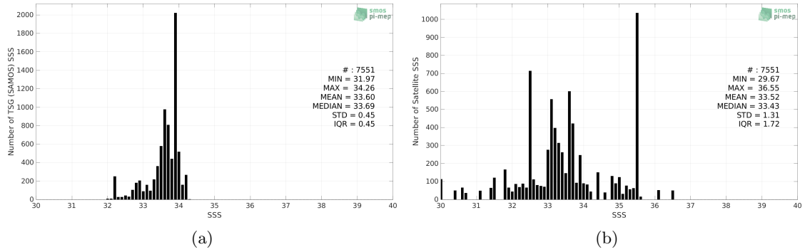
Figure 2: Histograms of SSS from TSG (SAMOS) (a) and SMOS SSS L2Q v331 - With FLAG (CMEMS-CATDS-CPDC) (b) considering all match-up pairs per bins of 0.1 over the South China Sea Pi-MEP region and for the full satellite product period.
