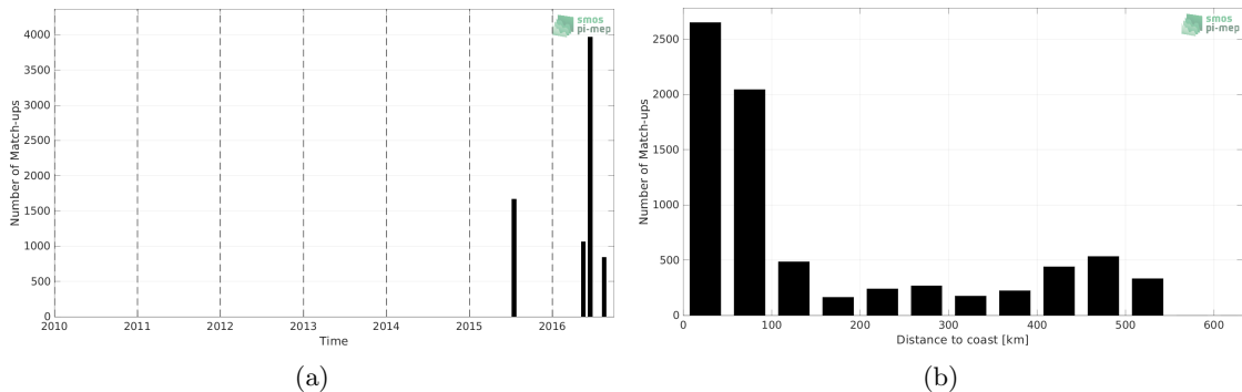
Figure 1: Number of match-ups between TSG (SAMOS) and SMOS SSS L2Q v331 - With FLAG (CMEMS-CATDS-CPDC) SSS as a function of time (a) and as function of the distance to coast (b) over the South China Sea Pi-MEP region and for the full satellite product period.
