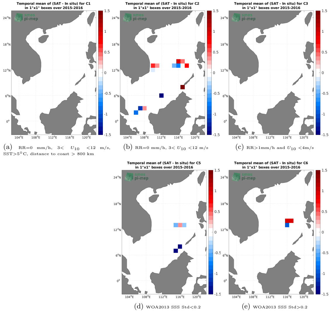
Figure 12: Temporal mean gridded over spatial boxes of size 1^\circ \times 1^\circ of \Delta SSS (SMOS SSS L2Q v331 - With FLAG (CMEMS-CATDS-CPDC) - TSG (SAMOS)) for 5 different subdatasets corresponding to:RR=0 mm/h, 3 < U_{10} < 12 m/s, SST>5°C, distance to coast > 800 km (a), RR=0 mm/h, 3 < U_{10} < 12 m/s (b), RR>1mm/h and U_{10} < 4 m/s (c), WOA2013 SSS Std<0.2 (d), WOA2013 SSS Std>0.2 (e).
