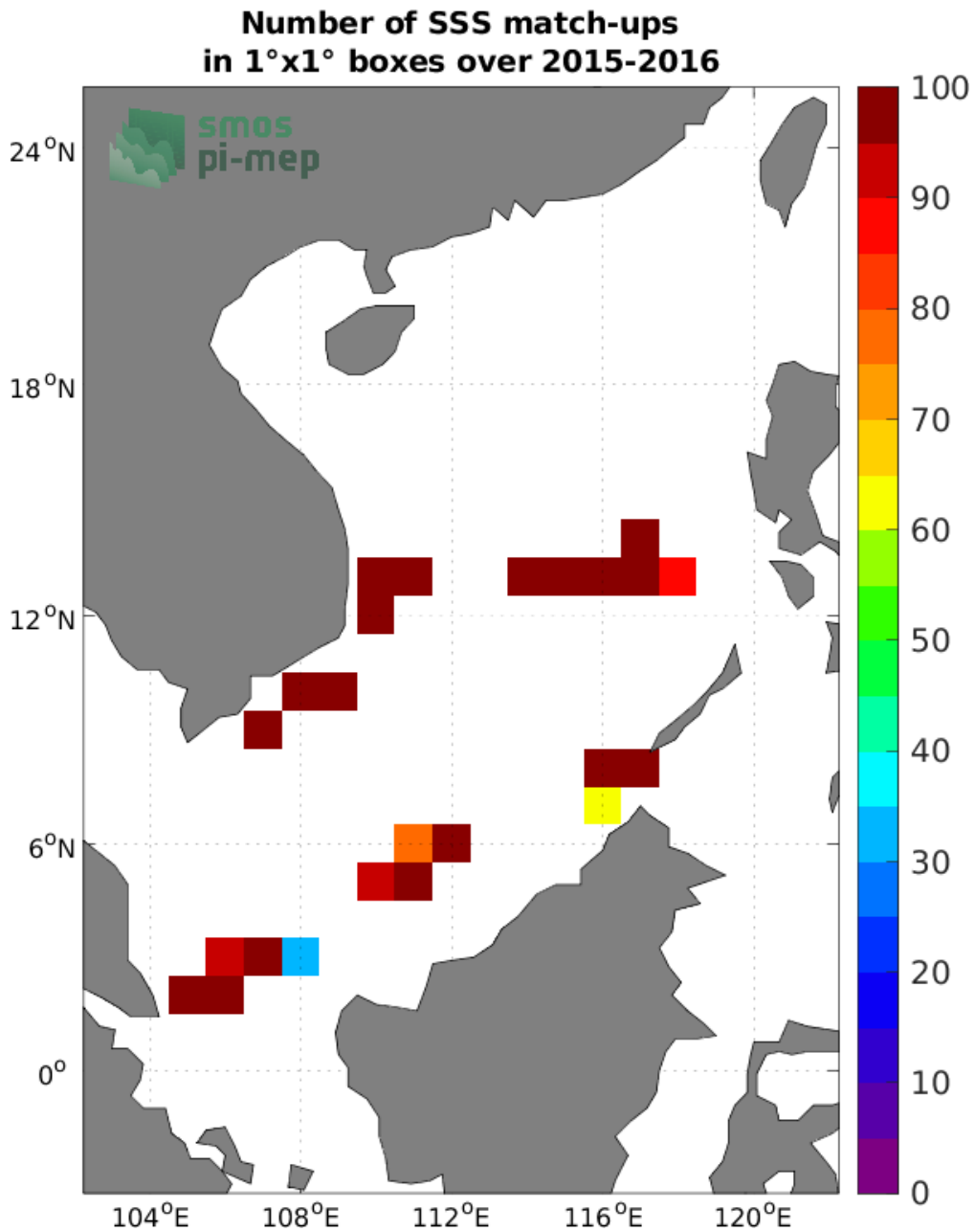
Figure 4: Number of SSS match-ups between TSG (SAMOS) SSS and the SMOS SSS L2Q v331 - With FLAG (CMEMS-CATDS-CPDC) SSS product for the South China Sea Pi-MEP region over 1°×1° boxes and for the full satellite product period.
