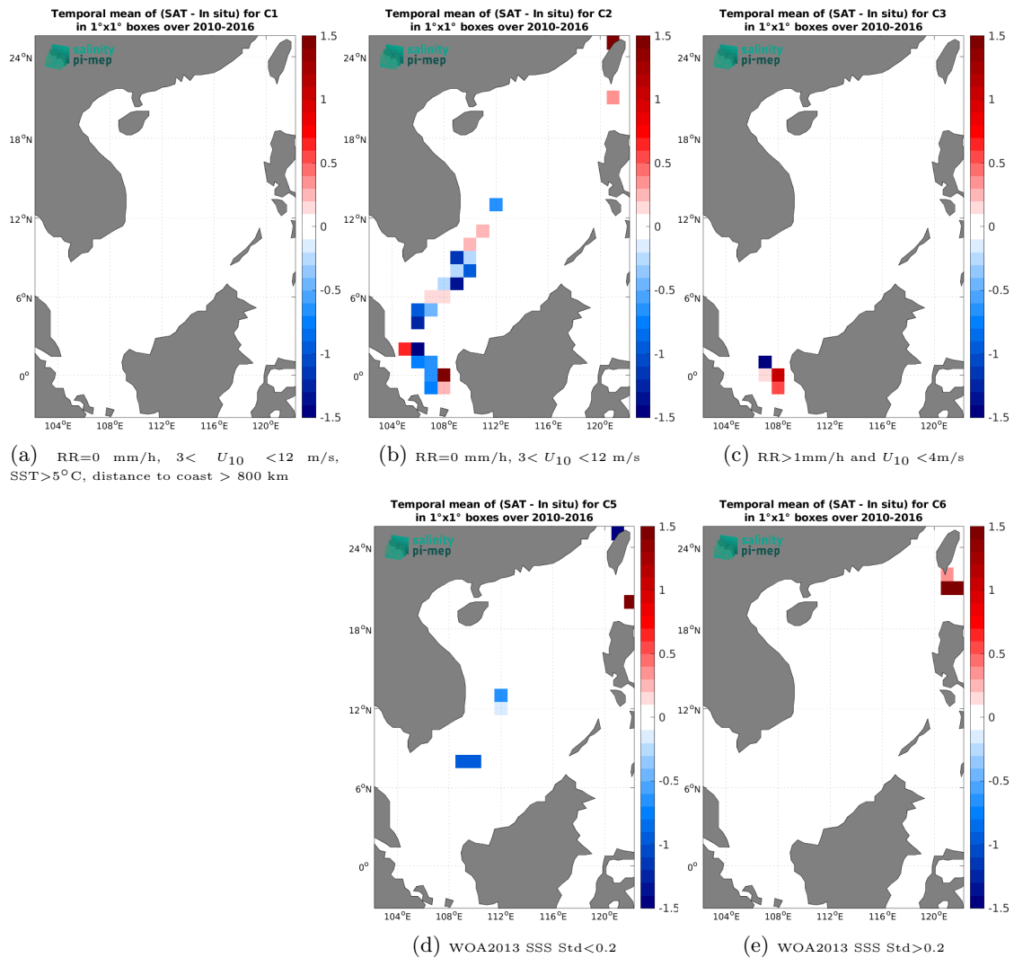
Figure 14: Temporal mean gridded over spatial boxes of size 1^\circ \times 1^\circ of \Delta SSS (SMOS SSS L2Q v331 - With FLAG (CMEMS-CATDS-CPDC) - TSG (LEGOS-DM)) for 5 different subdatasets corresponding to:RR=0 mm/h, 3 < U_{10} < 12 m/s, SST>5°C, distance to coast > 800 km (a), RR=0 mm/h, 3 < U_{10} < 12 m/s (b), RR>1mm/h and U_{10} < 4 m/s (c), WOA2013 SSS Std<0.2 (d), WOA2013 SSS Std>0.2 (e).
