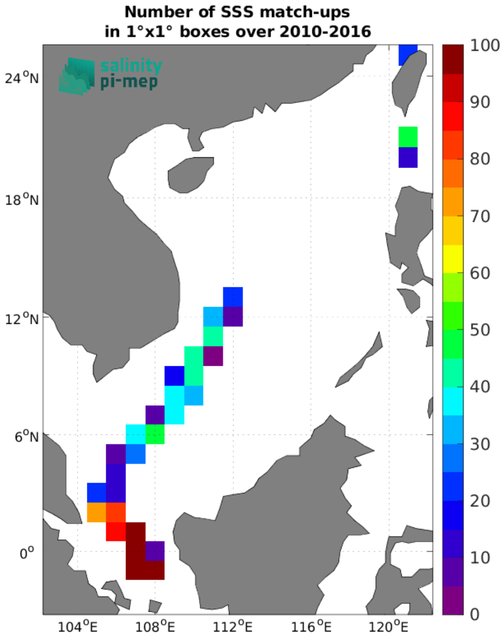
Figure 5: Number of SSS match-ups between TSG (LEGOS-DM) SSS and the SMOS SSS L2Q v331 - With FLAG (CMEMS-CATDS-CPDC) SSS product for the South China Sea Pi-MEP region over 1°x1° boxes and for the full satellite product period.
