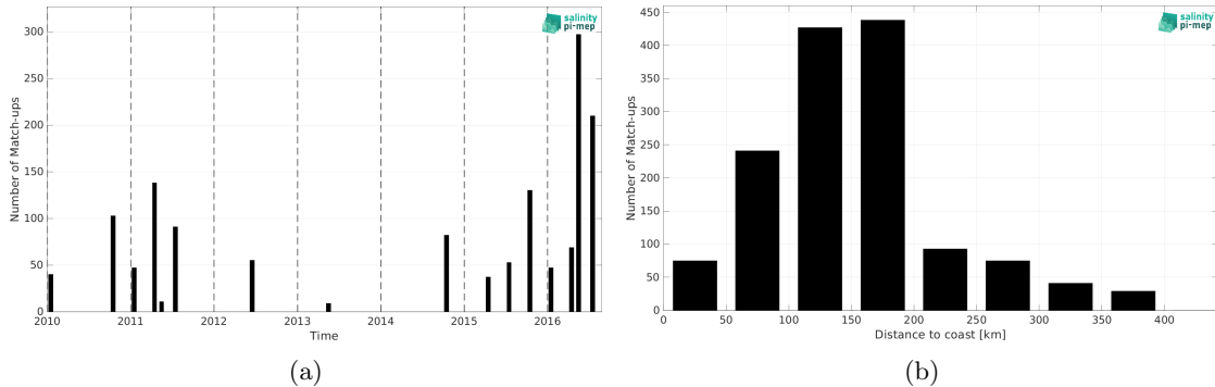
Figure 1: Number of match-ups between TSG (LEGOS-DM) and SMOS SSS L2Q v331 - With FLAG (CMEMS-CATDS-CPDC) SSS as a function of time (a) and as function of the distance to coast (b) over the South China Sea Pi-MEP region and for the full satellite product period.
