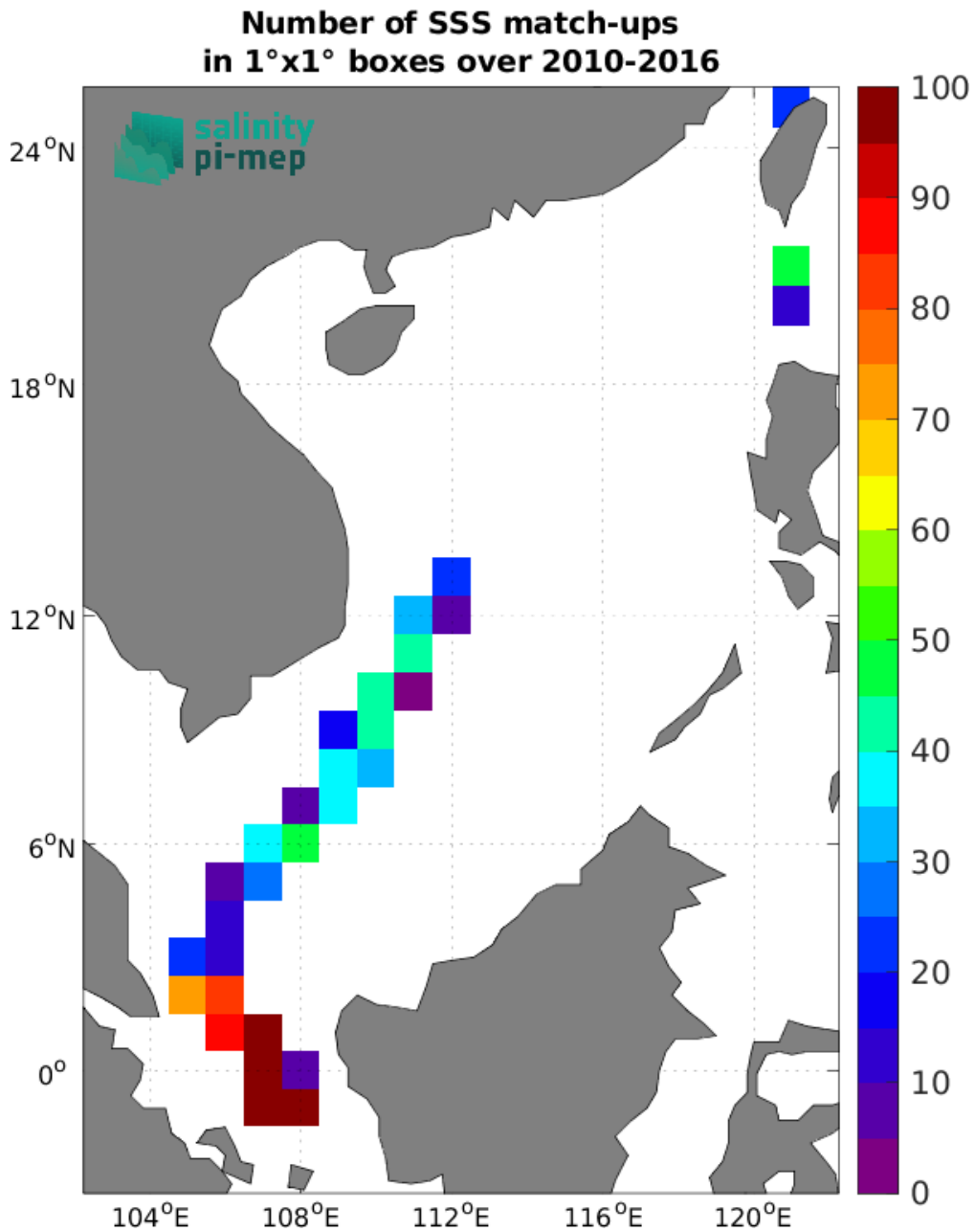
Figure 4: Number of SSS match-ups between TSG (LEGOS-DM) SSS and the SMOS SSS L2Q v331 - With FLAG (CMEMS-CATDS-CPDC) SSS product for the South China Sea Pi-MEP region over 1°x1° boxes and for the full satellite product period.
