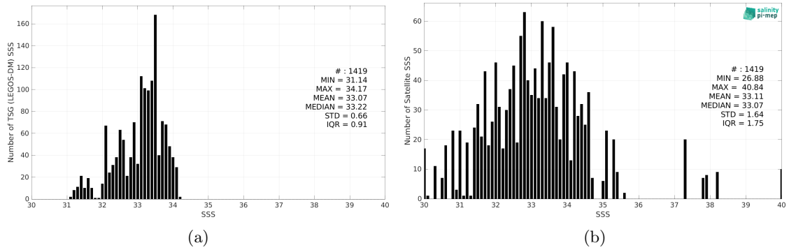
Figure 2: Histograms of SSS from TSG (LEGOS-DM) (a) and SMOS SSS L2Q v331 - With FLAG (CMEMS-CATDS-CPDC) (b) considering all match-up pairs per bins of 0.1 over the South China Sea Pi-MEP region and for the full satellite product period.
