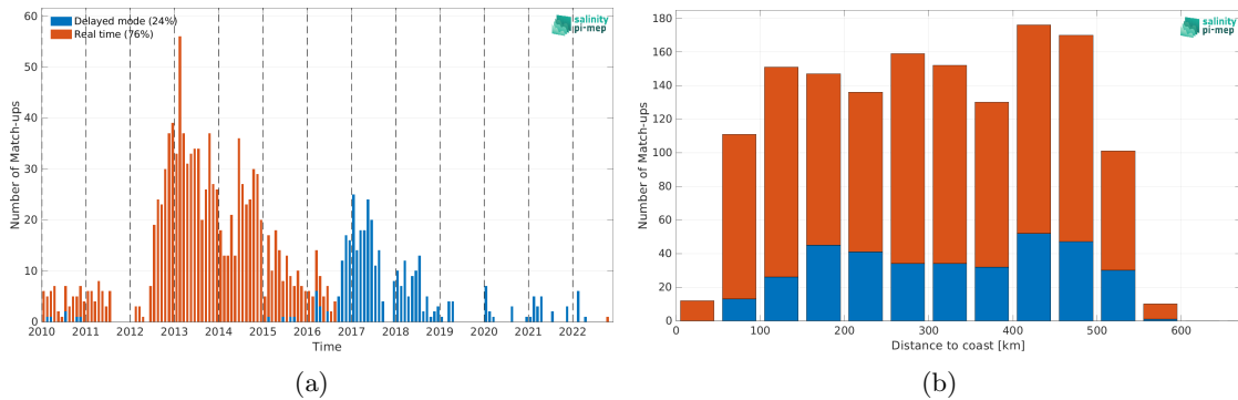
Figure 1: Number of match-ups between Argo and SMOS SSS L2Q v331 - With FLAG (CMEMS-CATDS-CPDC) SSS as a function of time (a) and as function of the distance to coast (b) over the South China Sea Pi-MEP region and for the full satellite product period.
