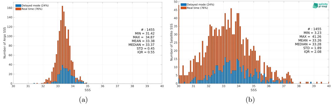
Figure 2: Histograms of SSS from Argo (a) and SMOS SSS L2Q v331 - With FLAG (CMEMS-CATDS-CPDC) (b) considering all match-up pairs per bins of 0.1 over the South China Sea Pi-MEP region and for the full satellite product period.
