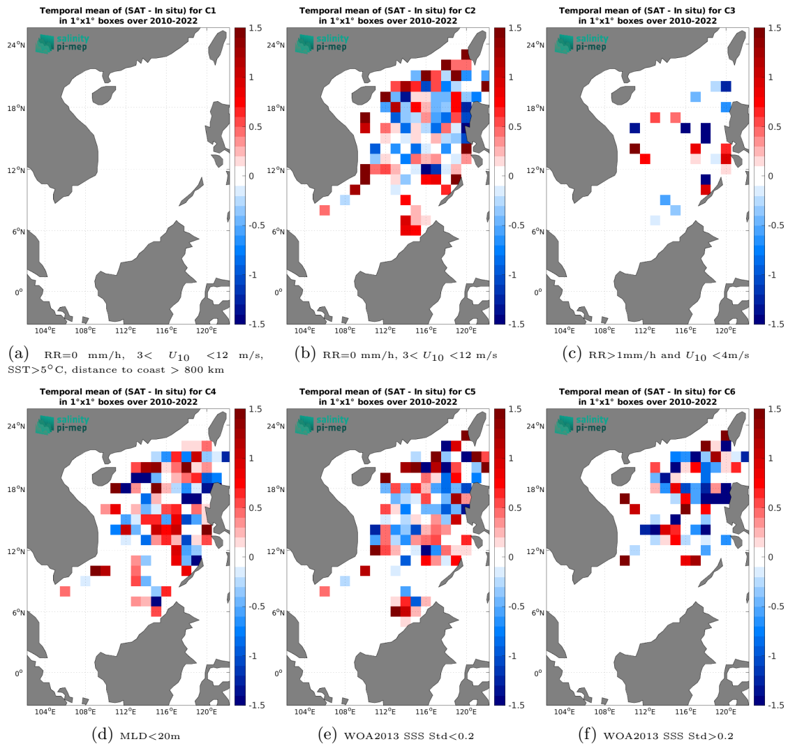
Figure 12: Temporal mean gridded over spatial boxes of size 1^\circ \times 1^\circ of \Delta SSS (SMOS SSS L2Q v331 - With FLAG (CMEMS-CATDS-CPDC) - Argo) for 6 different subdatasets corresponding to: RR=0 mm/h, 3 < U_{10} < 12 m/s, SST>5°C, distance to coast > 800 km (a), RR=0 mm/h, 3 < U_{10} < 12 m/s (b), RR>1mm/h and U_{10} < 4 m/s (c),MLD<20m (d),WOA2013 SSS Std<0.2 (e),WOA2013 SSS Std>0.2 (f).
