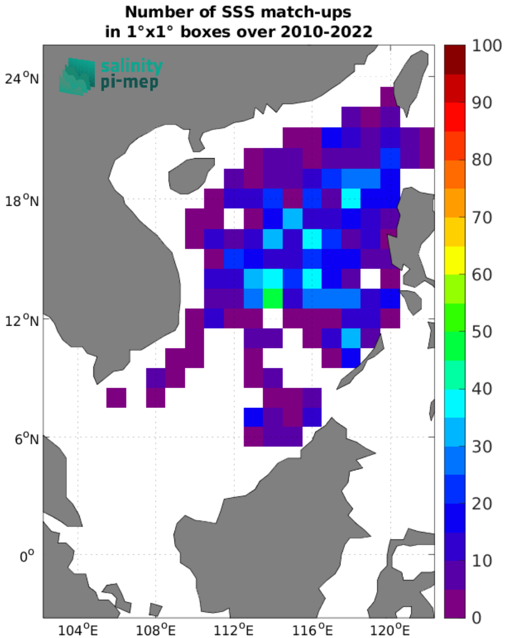
Figure 4: Number of SSS match-ups between Argo SSS and the SMOS SSS L2Q v331 - With FLAG (CMEMS-CATDS-CPDC) SSS product for the South China Sea Pi-MEP region over 1°x1° boxes and for the full satellite product period.
