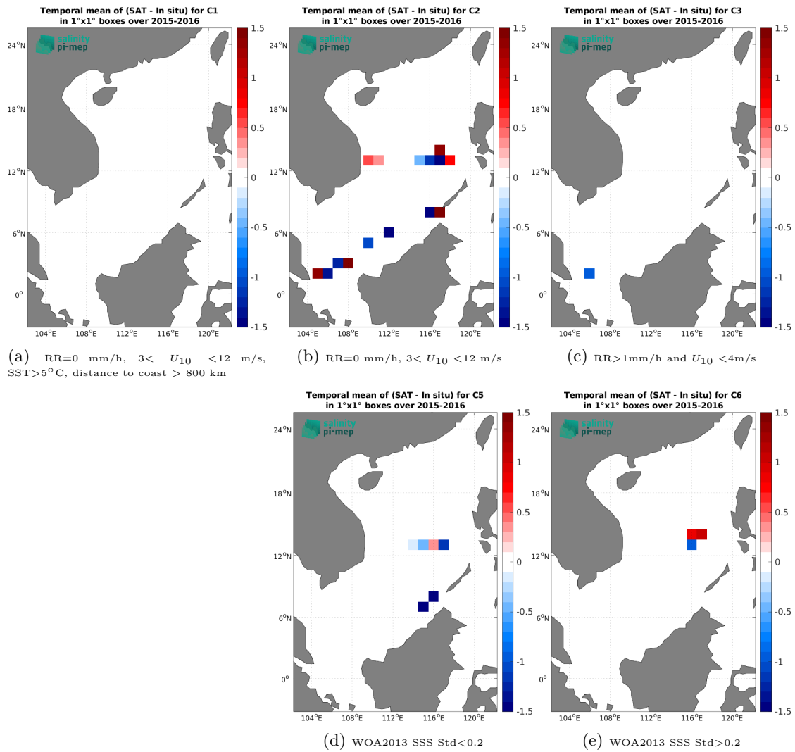
Figure 14: Temporal mean gridded over spatial boxes of size 1^\circ \times 1^\circ of \Delta SSS (SMOS SSS L2Q v331 - No FLAG (CMEMS-CATDS-CPDC) - TSG (SAMOS)) for 5 different subdatasets corresponding to: RR=0 mm/h, 3 < U_{10} < 12 m/s, SST>5°C, distance to coast > 800 km (a), RR=0 mm/h, 3 < U_{10} < 12 m/s (b), RR>1mm/h and U_{10} < 4 m/s (c), WOA2013 SSS Std<0.2 (d), WOA2013 SSS Std>0.2 (e).
