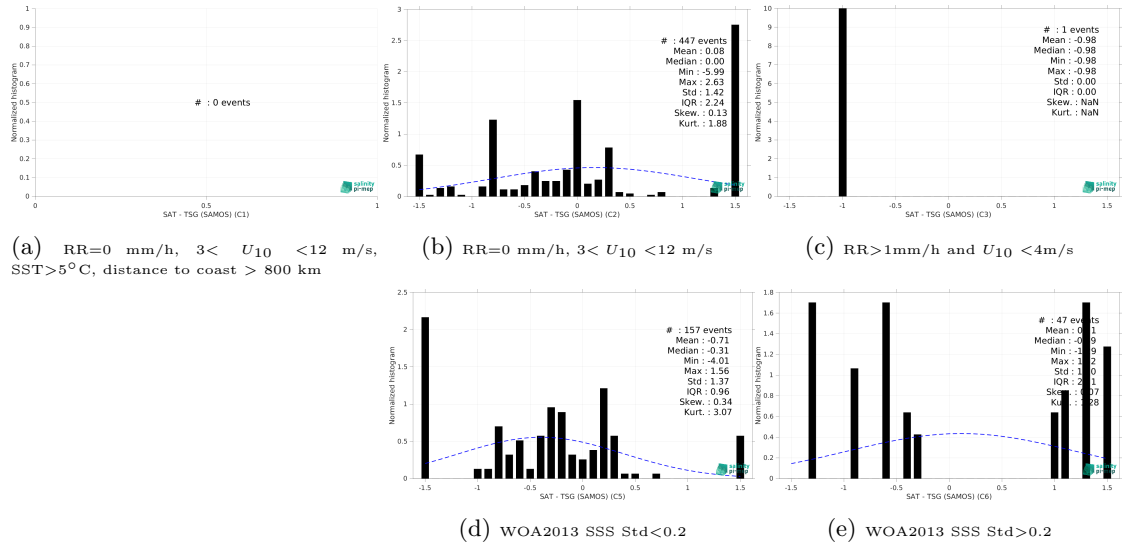
Figure 15: Normalized histogram of \Delta\text{SSS} (SMOS SSS L2Q v331 - No FLAG (CMEMS-CATDS-CPDC) - TSG (SAMOS)) for 5 different subdatasets corresponding to: RR=0 mm/h, 3 < U_{10} < 12 m/s, SST > 5^\circ\text{C} , distance to coast > 800 km (a), RR=0 mm/h, 3 < U_{10} < 12 m/s (b), RR > 1 mm/h and U_{10} < 4 m/s (c), WOA2013 SSS Std < 0.2 (d), WOA2013 SSS Std > 0.2 (e).
