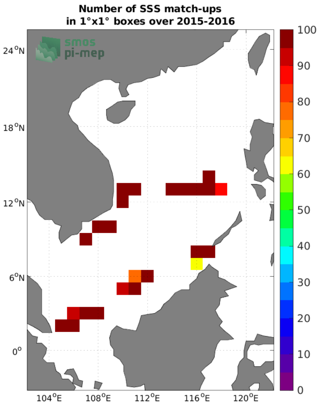
Figure 4: Number of SSS match-ups between TSG (SAMOS) SSS and the SMOS SSS L2Q v331 - No FLAG (CMEMS-CATDS-CPDC) SSS product for the South China Sea Pi-MEP region over 1°x1° boxes and for the full satellite product period.
