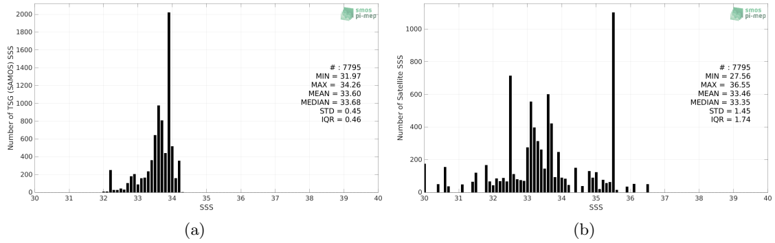
Figure 2: Histograms of SSS from TSG (SAMOS) (a) and SMOS SSS L2Q v331 - No FLAG (CMEMS-CATDS-CPDC) (b) considering all match-up pairs per bins of 0.1 over the South China Sea Pi-MEP region and for the full satellite product period.
