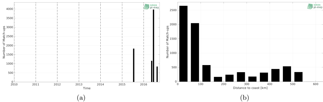
Figure 1: Number of match-ups between TSG (SAMOS) and SMOS SSS L2Q v331 - No FLAG (CMEMS-CATDS-CPDC) SSS as a function of time (a) and as function of the distance to coast (b) over the South China Sea Pi-MEP region and for the full satellite product period.
