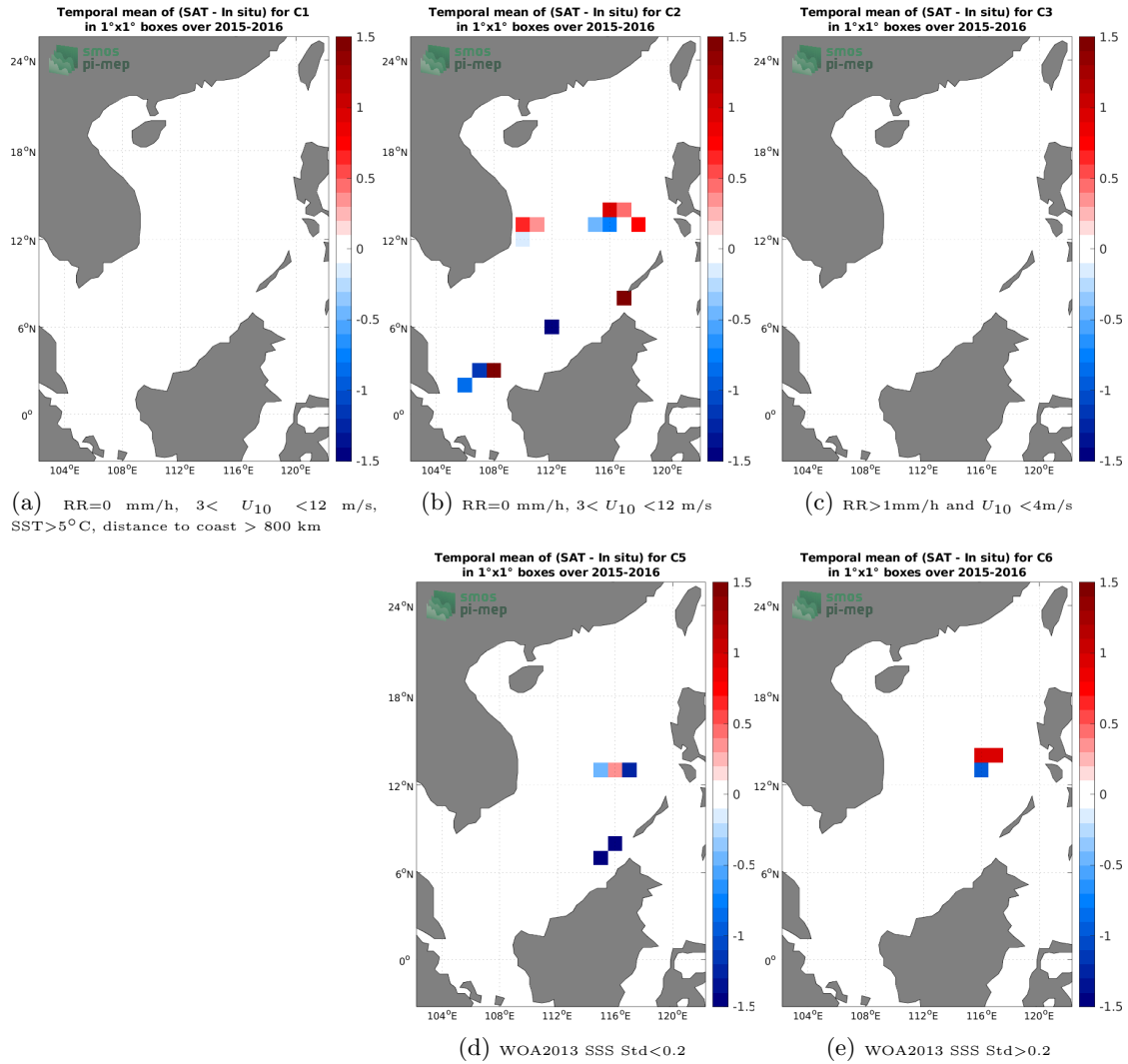
Figure 12: Temporal mean gridded over spatial boxes of size 1^\circ \times 1^\circ of \Delta SSS (SMOS SSS L2Q v331 - No FLAG (CMEMS-CATDS-CPDC) - TSG (SAMOS)) for 5 different subdatasets corresponding to: RR=0 mm/h, 3 < U_{10} < 12 m/s, SST > 5°C, distance to coast > 800 km (a), RR=0 mm/h, 3 < U_{10} < 12 m/s (b), RR > 1mm/h and U_{10} < 4 m/s (c), WOA2013 SSS Std < 0.2 (d), WOA2013 SSS Std > 0.2 (e).
