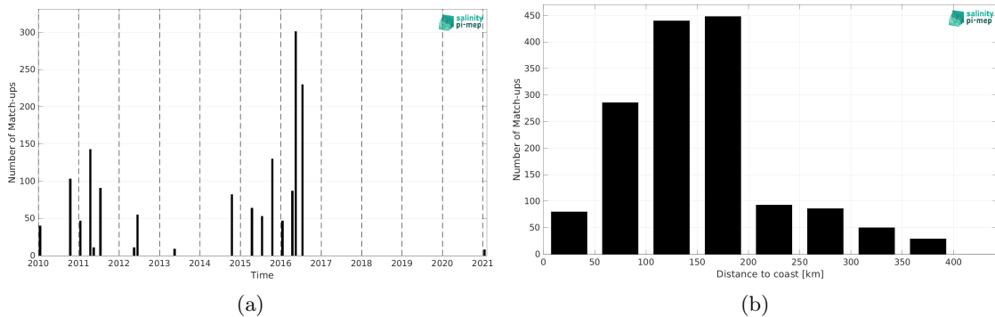
Figure 2: Number of match-ups between TSG (LEGOS-DM) and SMOS SSS L2Q v331 - No FLAG (CMEMS-CATDS-CPDC) SSS as a function of time (a) and as function of the distance to coast (b) over the South China Sea Pi-MEP region and for the full satellite product period.
