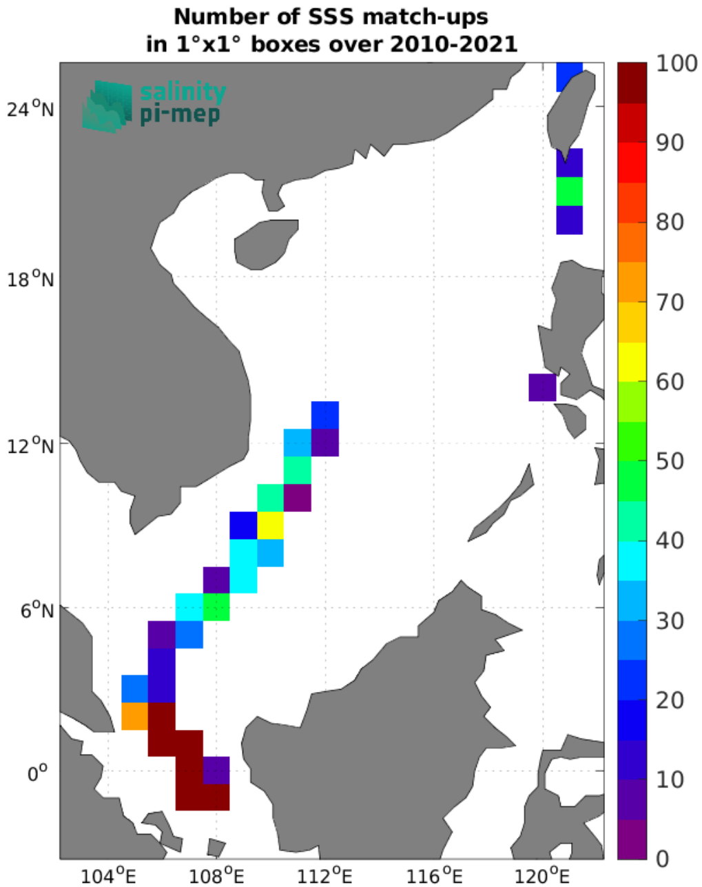
Figure 5: Number of SSS match-ups between TSG (LEGOS-DM) SSS and the SMOS SSS L2Q v331 - No FLAG (CMEMS-CATDS-CPDC) SSS product for the South China Sea Pi-MEP region over 1°×1° boxes and for the full satellite product period.
