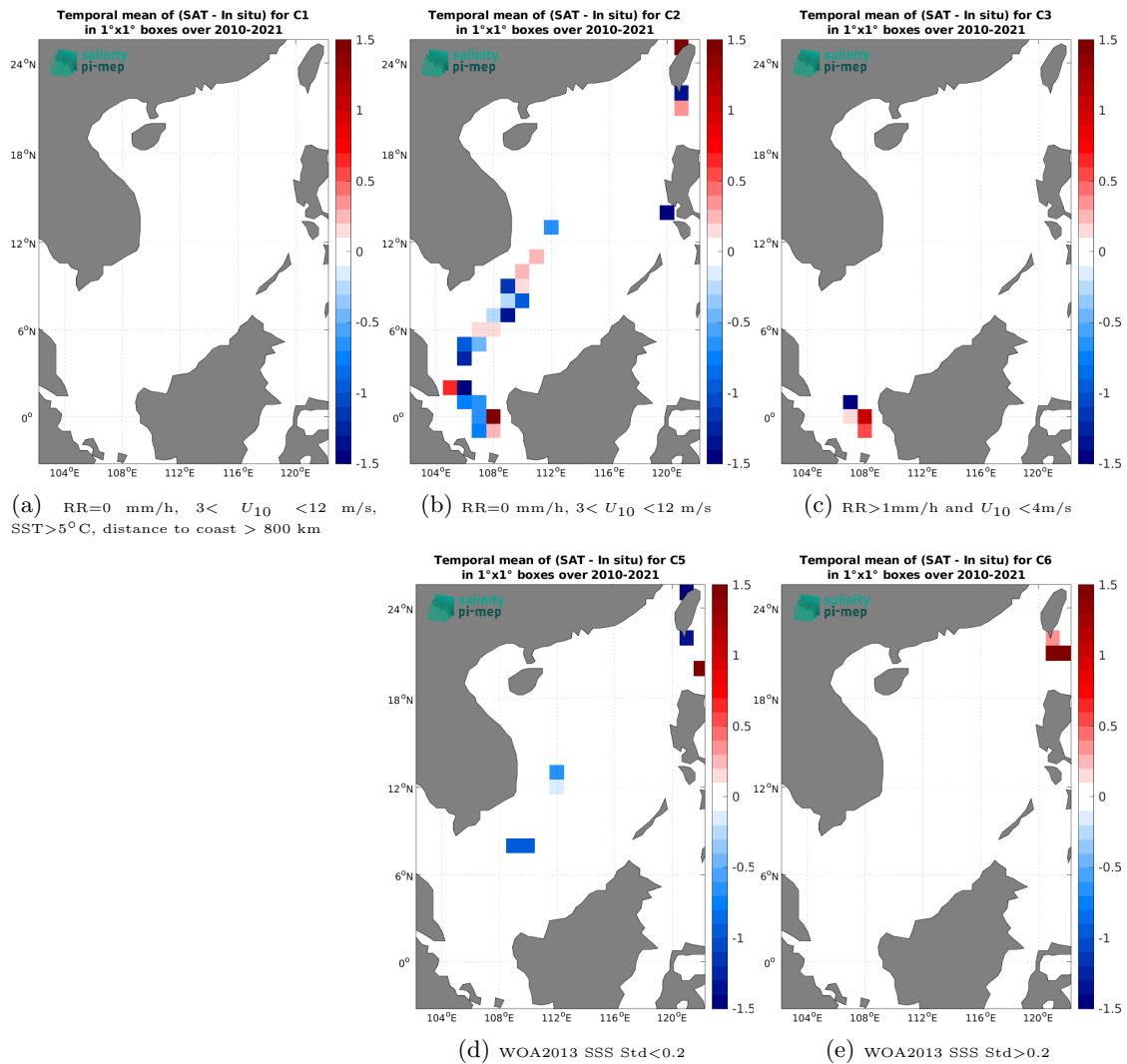
Figure 14: Temporal mean gridded over spatial boxes of size 1^\circ \times 1^\circ of \Delta\text{SSS} (SMOS SSS L2Q v331 - No FLAG (CMEMS-CATDS-CPDC) - TSG (LEGOS-DM)) for 5 different subdatasets corresponding to: RR=0 mm/h, 3 < U_{10} < 12 m/s, SST > 5^\circ\text{C} , distance to coast > 800 km (a), RR=0 mm/h, 3 < U_{10} < 12 m/s (b), RR > 1 mm/h and U_{10} < 4 m/s (c), WOA2013 SSS Std < 0.2 (d), WOA2013 SSS Std > 0.2 (e).
