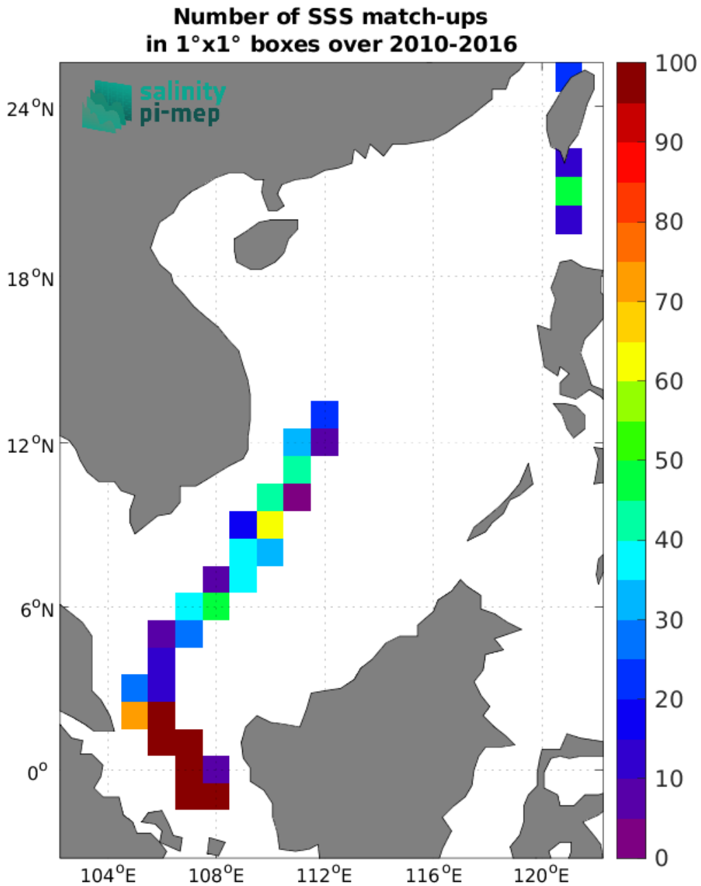
Figure 4: Number of SSS match-ups between TSG (LEGOS-DM) SSS and the SMOS SSS L2Q v331 - No FLAG (CMEMS-CATDS-CPDC) SSS product for the South China Sea Pi-MEP region over 1°x1° boxes and for the full satellite product period.
