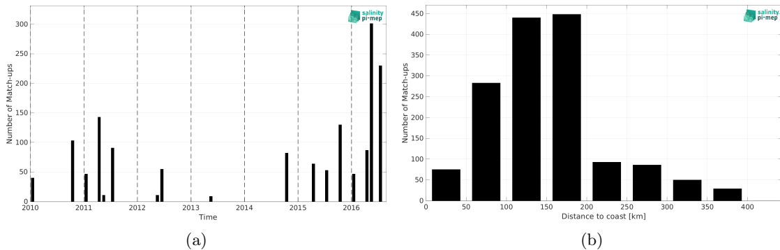
Figure 1: Number of match-ups between TSG (LEGOS-DM) and SMOS SSS L2Q v331 - No FLAG (CMEMS-CATDS-CPDC) SSS as a function of time (a) and as function of the distance to coast (b) over the South China Sea Pi-MEP region and for the full satellite product period.
