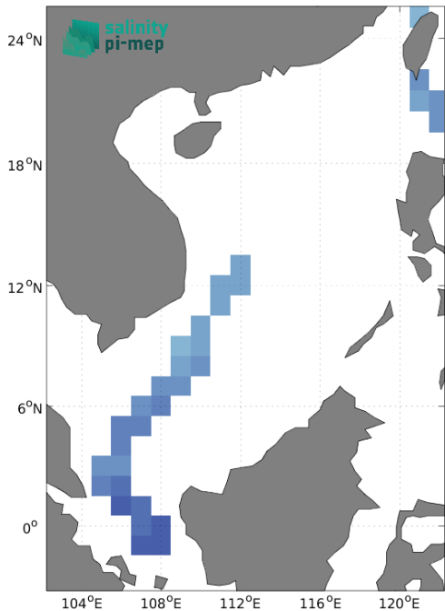
(c) MEAN(TSG (LEGOS-DM) SSS)
