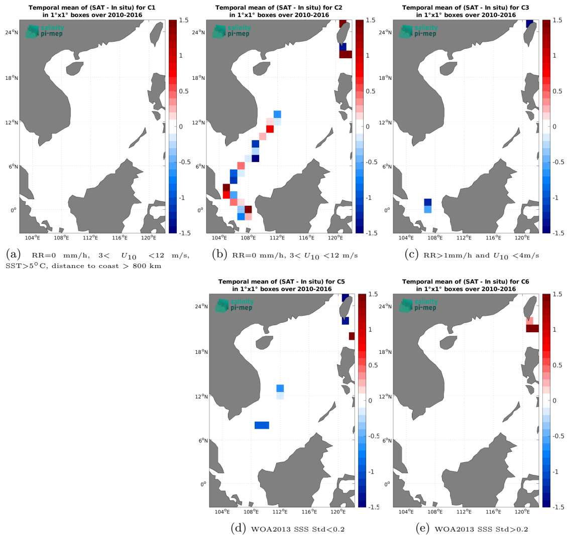
Figure 12: Temporal mean gridded over spatial boxes of size 1^\circ \times 1^\circ of \Delta SSS (SMOS SSS L2Q v331 - No FLAG (CMEMS-CATDS-CPDC) - TSG (LEGOS-DM)) for 5 different subdatasets corresponding to:RR=0 mm/h, 3 < U_{10} < 12 m/s, SST>5°C, distance to coast > 800 km (a), RR=0 mm/h, 3 < U_{10} < 12 m/s (b), RR>1mm/h and U_{10} < 4 m/s (c), WOA2013 SSS Std<0.2 (d), WOA2013 SSS Std>0.2 (e).
