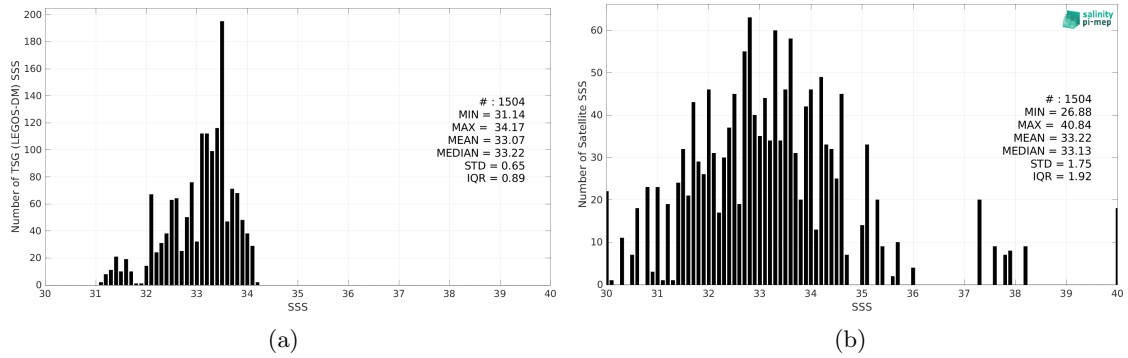
Figure 2: Histograms of SSS from TSG (LEGOS-DM) (a) and SMOS SSS L2Q v331 - No FLAG (CMEMS-CATDS-CPDC) (b) considering all match-up pairs per bins of 0.1 over the South China Sea Pi-MEP region and for the full satellite product period.
