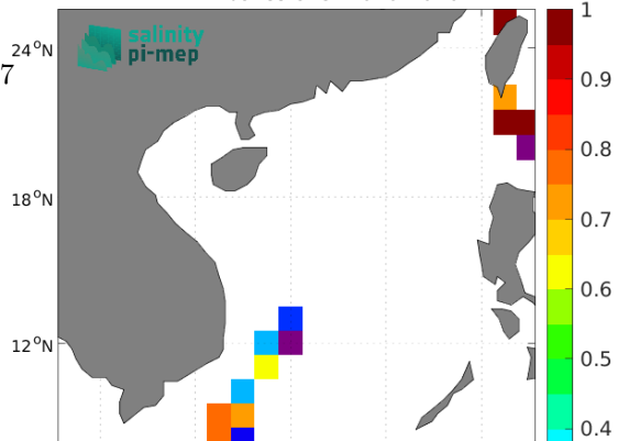
Temporal STD of (Sat - TSG (LEGOS-DM)) in 1°x1° boxes over 2010-2016
