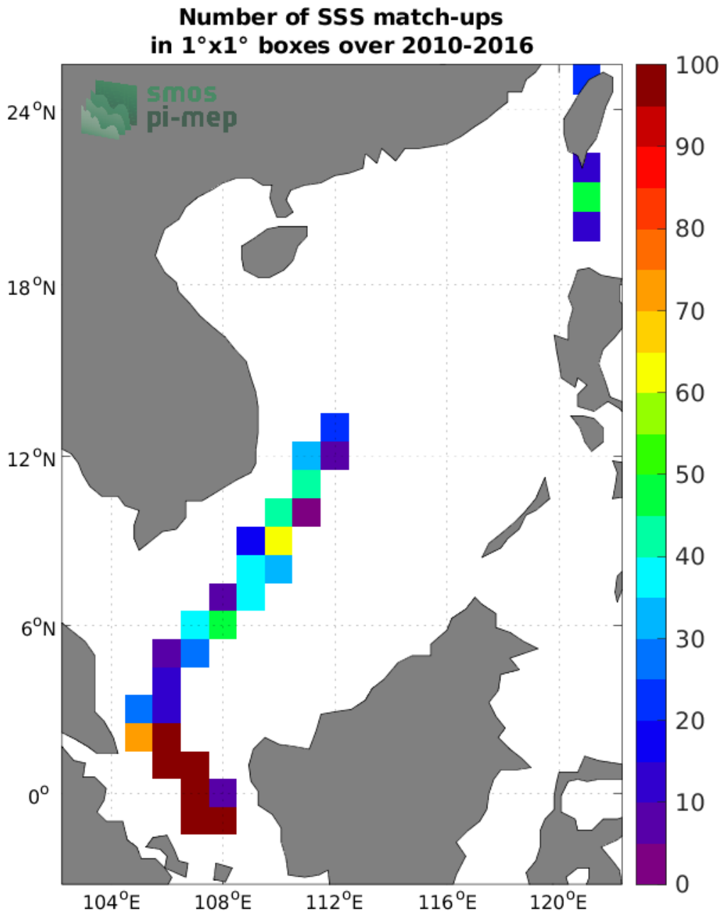
Figure 4: Number of SSS match-ups between TSG (LEGOS-DM) SSS and the SMOS SSS L2Q v331 - No FLAG (CMEMS-CATDS-CPDC) SSS product for the South China Sea Pi-MEP region over 1°×1° boxes and for the full satellite product period.
