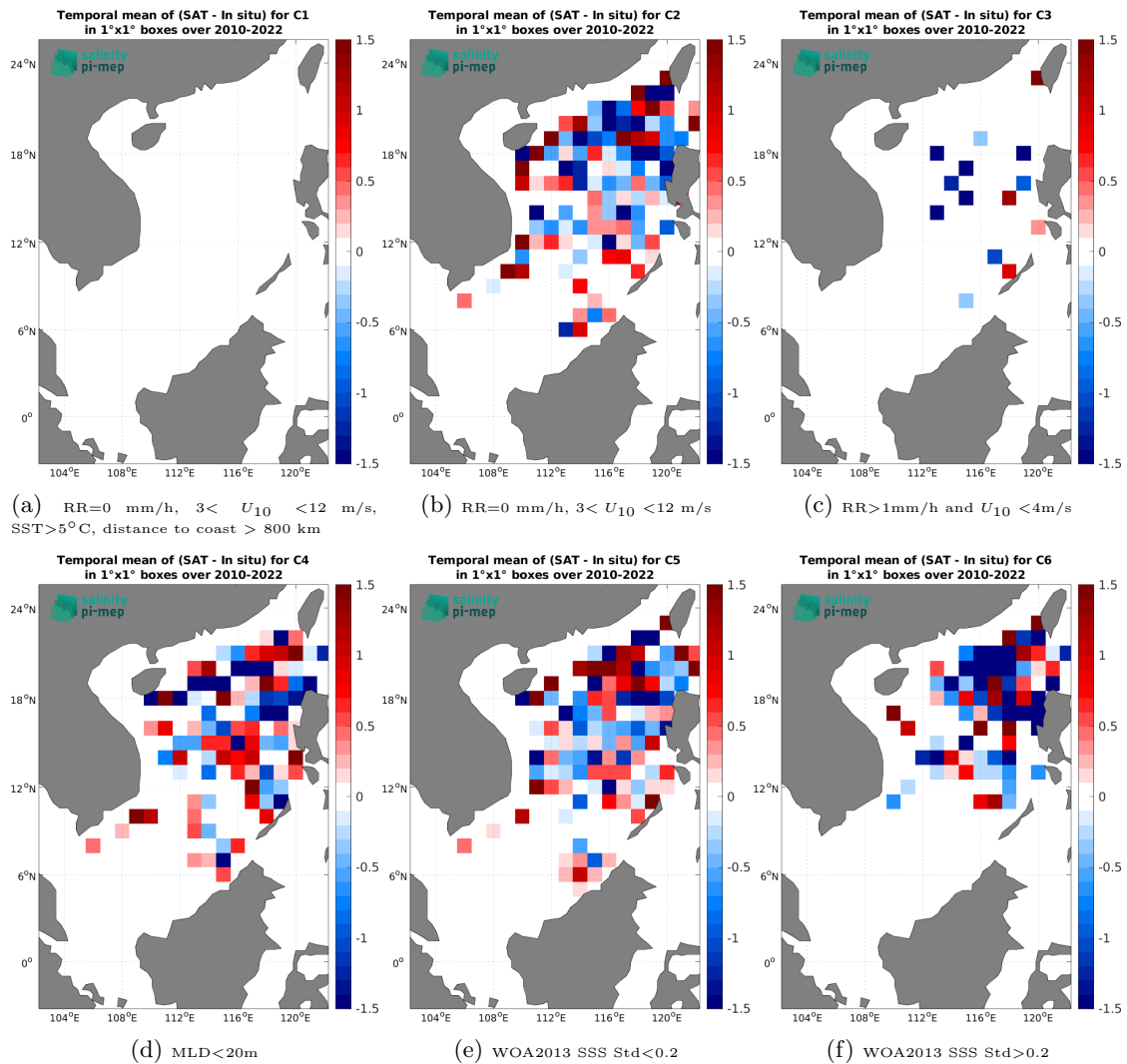
Figure 14: Temporal mean gridded over spatial boxes of size 1^\circ \times 1^\circ of \Delta SSS (SMOS SSS L2Q v331 - No FLAG (CMEMS-CATDS-CPDC) - Argo) for 6 different subdatasets corresponding to:RR=0 mm/h, 3 < U_{10} < 12 m/s, SST>5°C, distance to coast > 800 km (a), RR=0 mm/h, 3 < U_{10} < 12 m/s (b), RR>1mm/h and U_{10} < 4 m/s (c),MLD<20m (d),WOA2013 SSS Std<0.2 (e),WOA2013 SSS Std>0.2 (f).
