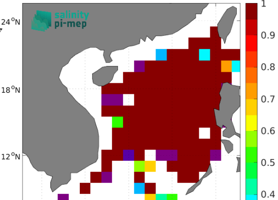
Temporal STD of (Sat - Argo) in 1°x1° boxes over 2010-2022
