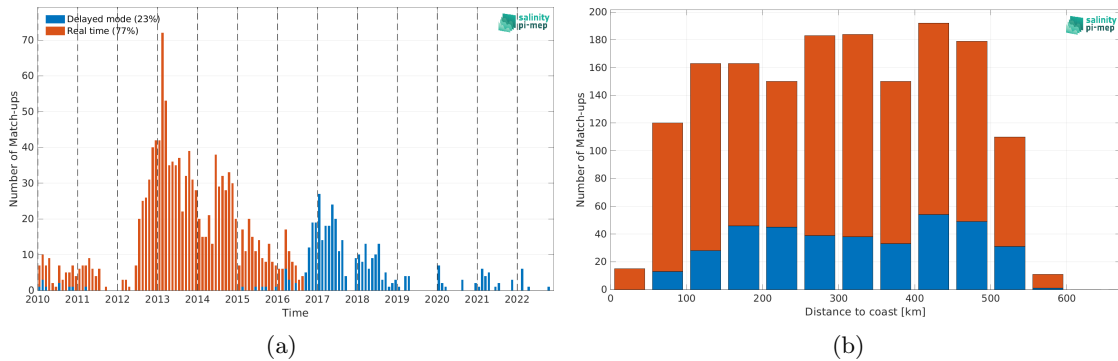
Figure 2: Number of match-ups between Argo and SMOS SSS L2Q v331 - No FLAG (CMEMS-CATDS-CPDC) SSS as a function of time (a) and as function of the distance to coast (b) over the South China Sea Pi-MEP region and for the full satellite product period.
