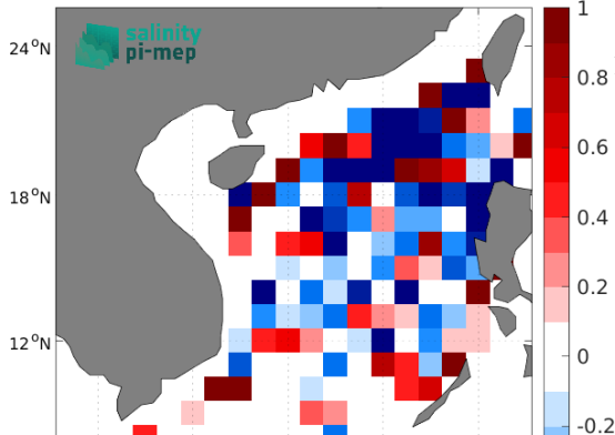
Temporal mean of (Sat - Argo) in 1°x1° boxes over 2010-2022
