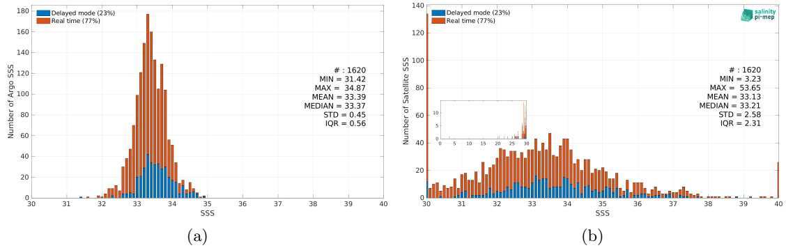
Figure 3: Histograms of SSS from Argo (a) and SMOS SSS L2Q v331 - No FLAG (CMEMS-CATDS-CPDC) (b) considering all match-up pairs per bins of 0.1 over the South China Sea Pi-MEP region and for the full satellite product period.
