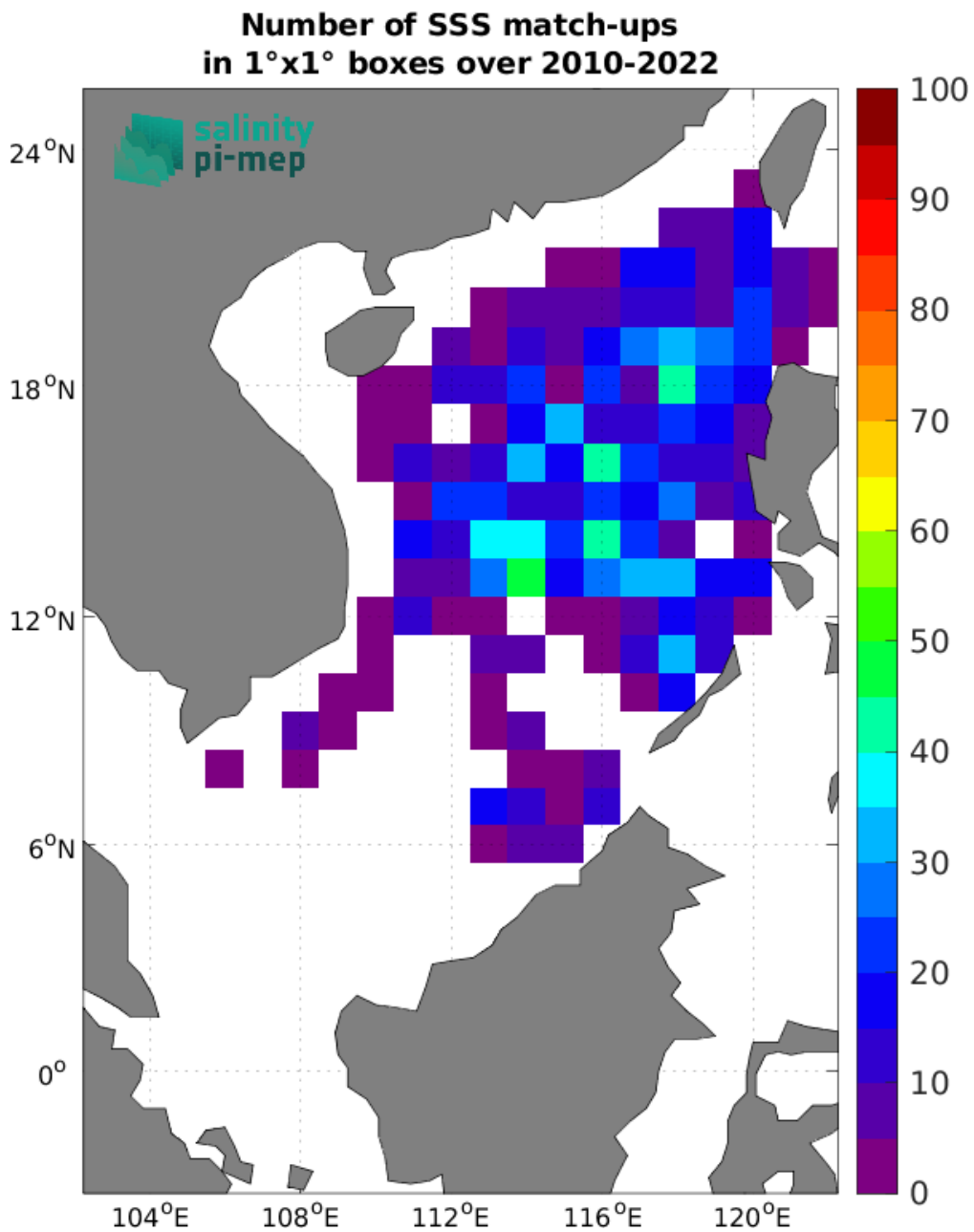
Figure 4: Number of SSS match-ups between Argo SSS and the SMOS SSS L2Q v331 - No FLAG (CMEMS-CATDS-CPDC) SSS product for the South China Sea Pi-MEP region over 1^\circ \times 1^\circ boxes and for the full satellite product period.
