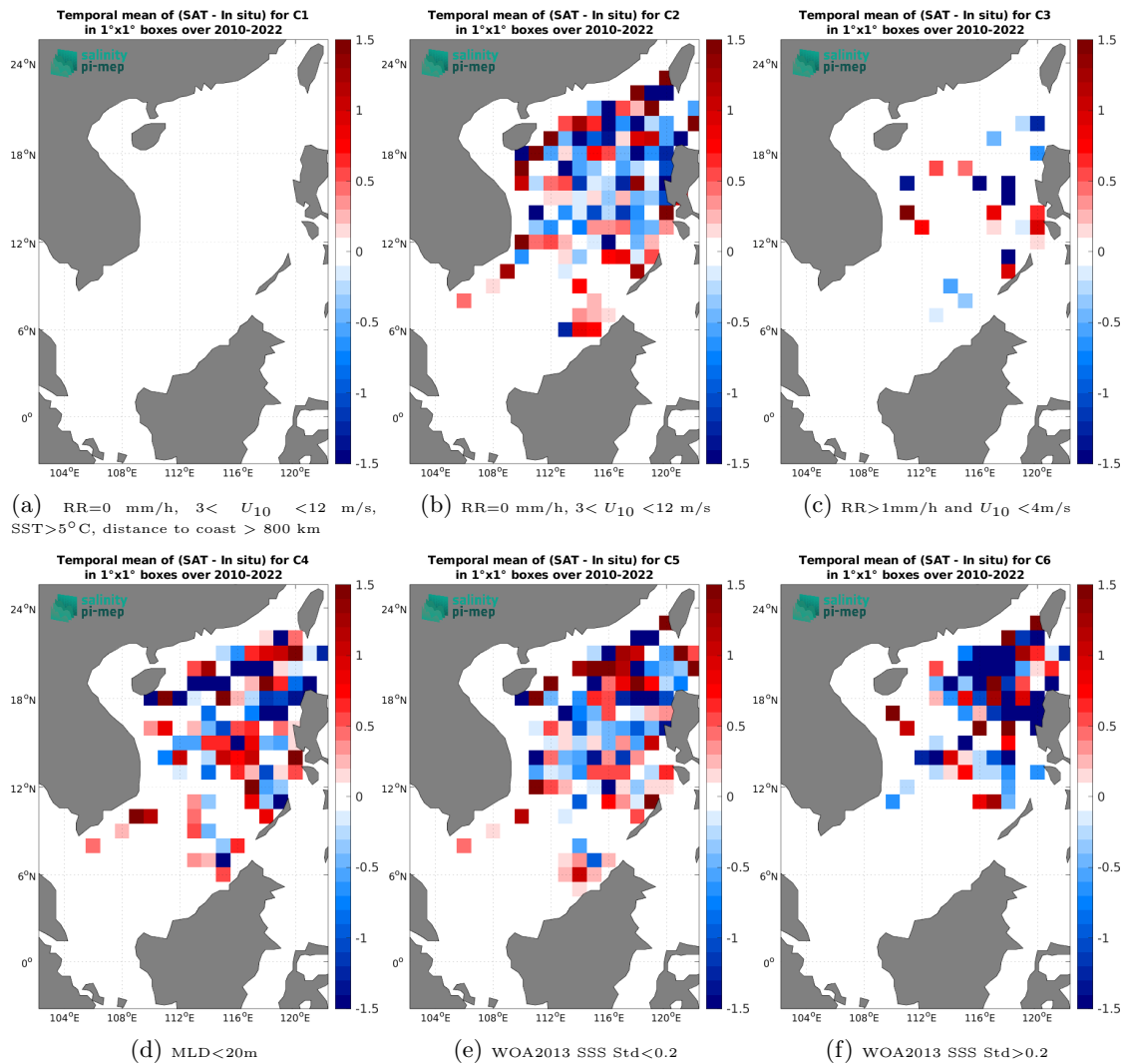
Figure 12: Temporal mean gridded over spatial boxes of size 1^\circ \times 1^\circ of \Delta\text{SSS} (SMOS SSS L2Q v331 - No FLAG (CMEMS-CATDS-CPDC) - Argo) for 6 different subdatasets corresponding to: RR=0 mm/h, 3 < U_{10} < 12 m/s, SST >5^\circ\text{C} , distance to coast > 800 km (a), RR=0 mm/h, 3 < U_{10} < 12 m/s (b), RR >1 mm/h and U_{10} < 4 m/s (c),MLD <20 m (d),WOA2013 SSS Std <0.2 (e),WOA2013 SSS Std >0.2 (f).
