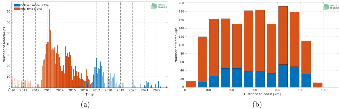
Figure 1: Number of match-ups between Argo and SMOS SSS L2Q v331 - No FLAG (CMEMS-CATDS-CPDC) SSS as a function of time (a) and as function of the distance to coast (b) over the South China Sea Pi-MEP region and for the full satellite product period.
