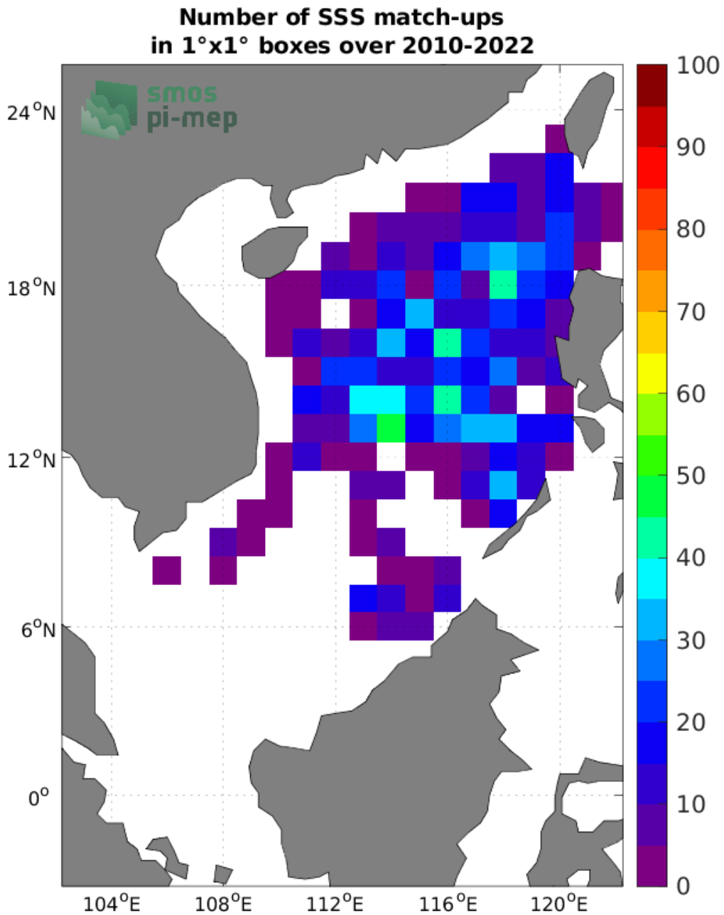
Figure 4: Number of SSS match-ups between Argo SSS and the SMOS SSS L2Q v331 - No FLAG (CMEMS-CATDS-CPDC) SSS product for the South China Sea Pi-MEP region over 1°x1° boxes and for the full satellite product period.
