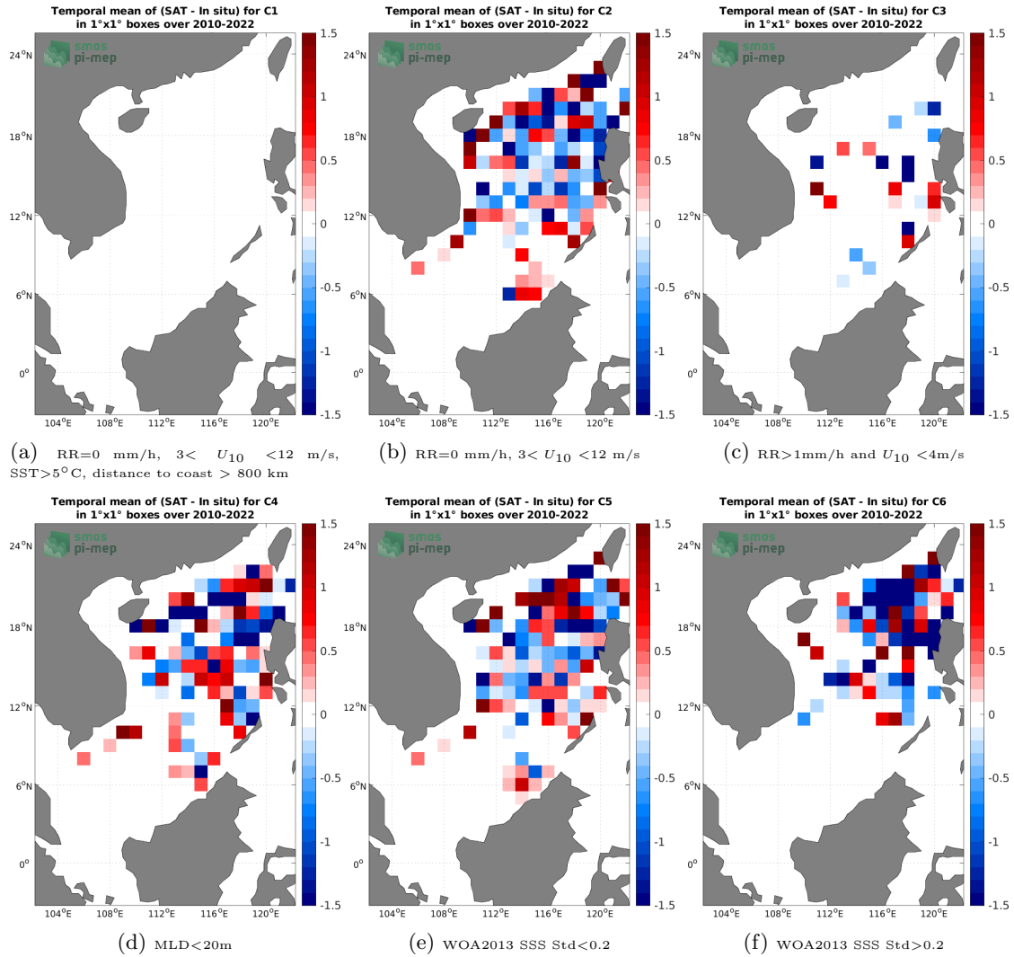
Figure 12: Temporal mean gridded over spatial boxes of size 1^\circ \times 1^\circ of \Delta SSS (SMOS SSS L2Q v331 - No FLAG (CMEMS-CATDS-CPDC) - Argo) for 6 different subdatasets corresponding to:RR=0 mm/h, 3 < U_{10} < 12 m/s, SST>5°C, distance to coast > 800 km (a), RR=0 mm/h, 3 < U_{10} < 12 m/s (b), RR>1mm/h and U_{10} < 4 m/s (c),MLD<20m (d),WOA2013 SSS Std<0.2 (e),WOA2013 SSS Std>0.2 (f).
