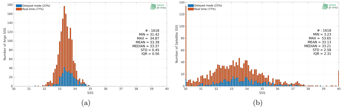
Figure 2: Histograms of SSS from Argo (a) and SMOS SSS L2Q v331 - No FLAG (CMEMS-CATDS-CPDC) (b) considering all match-up pairs per bins of 0.1 over the South China Sea Pi-MEP region and for the full satellite product period.
