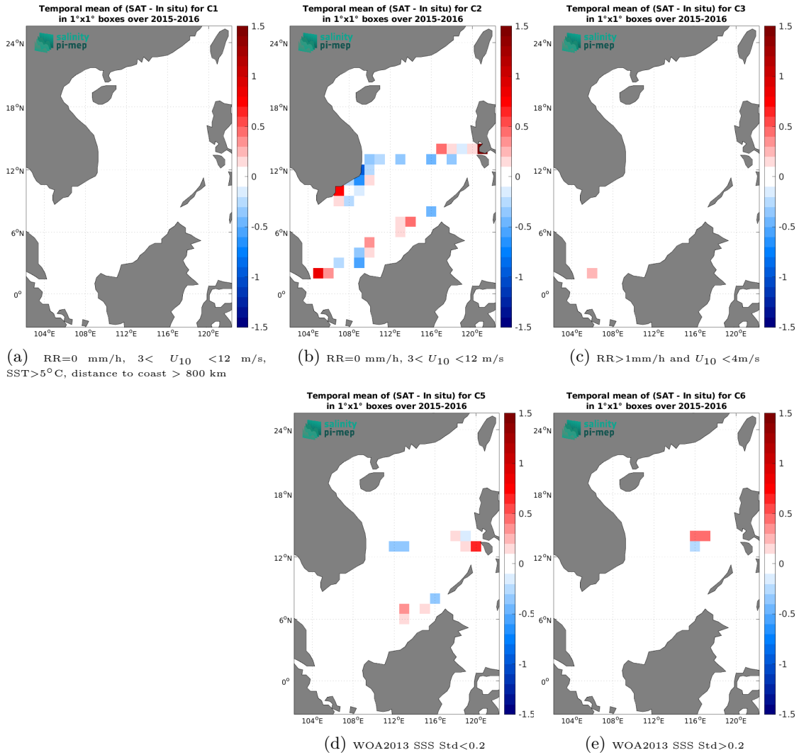
Figure 14: Temporal mean gridded over spatial boxes of size 1^\circ \times 1^\circ of \Delta\text{SSS} (SMOS SSS L3 v9 - 9 Days (CATDS-CEC-LOCEAN) - TSG (SAMOS)) for 5 different subdatasets corresponding to: RR=0 mm/h, 3 < U_{10} < 12 m/s, SST > 5^\circ\text{C} , distance to coast > 800 km (a), RR=0 mm/h, 3 < U_{10} < 12 m/s (b), RR > 1 mm/h and U_{10} < 4 m/s (c), WOA2013 SSS Std < 0.2 (d), WOA2013 SSS Std > 0.2 (e).
