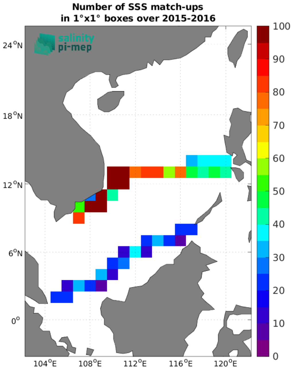
Figure 5: Number of SSS match-ups between TSG (SAMOS) SSS and the SMOS SSS L3 v9 - 9 Days (CATDS-CEC-LOCEAN) SSS product for the South China Sea Pi-MEP region over 1^\circ \times 1^\circ boxes and for the full satellite product period.
