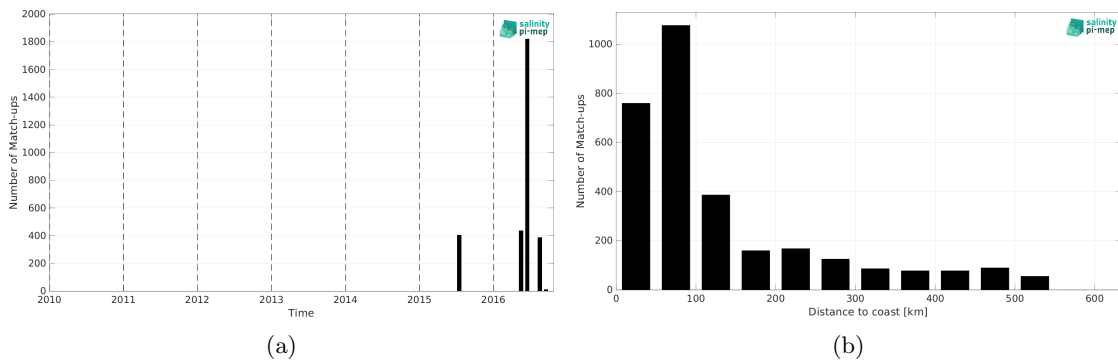
Figure 1: Number of match-ups between TSG (SAMOS) and SMOS SSS L3 v9 - 9 Days (CATDS-CEC-LOCEAN) SSS as a function of time (a) and as function of the distance to coast (b) over the South China Sea Pi-MEP region and for the full satellite product period.
