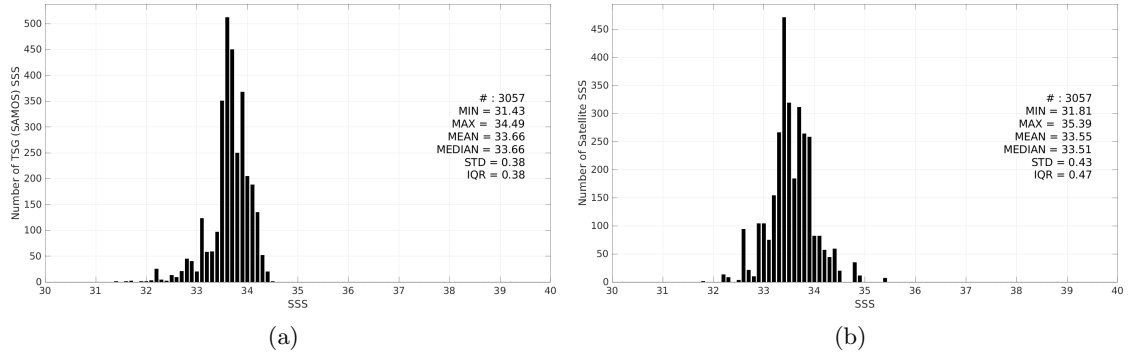
Figure 2: Histograms of SSS from TSG (SAMOS) (a) and SMOS SSS L3 v9 - 9 Days (CATDS-CEC-LOCEAN) (b) considering all match-up pairs per bins of 0.1 over the South China Sea Pi-MEP region and for the full satellite product period.
