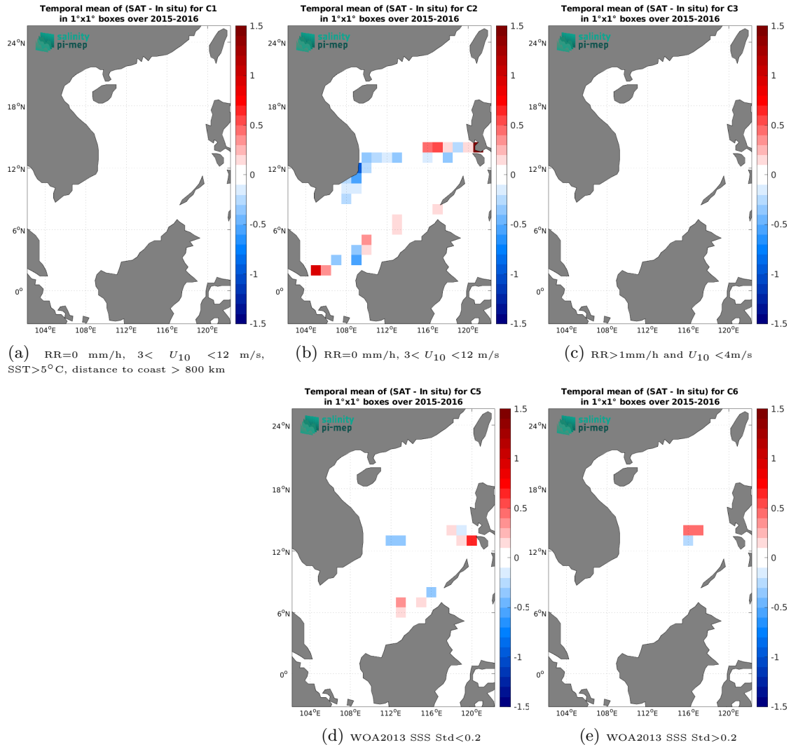
Figure 12: Temporal mean gridded over spatial boxes of size 1^\circ \times 1^\circ of \Delta SSS (SMOS SSS L3 v9 - 9 Days (CATDS-CEC-LOCEAN) - TSG (SAMOS)) for 5 different subdatasets corresponding to: RR=0 mm/h, 3 < U_{10} < 12 m/s, SST >5^\circ C, distance to coast > 800 km (a), RR=0 mm/h, 3 < U_{10} < 12 m/s (b), RR >1 mm/h and U_{10} < 4 m/s (c), WOA2013 SSS Std <0.2 (d), WOA2013 SSS Std >0.2 (e).
