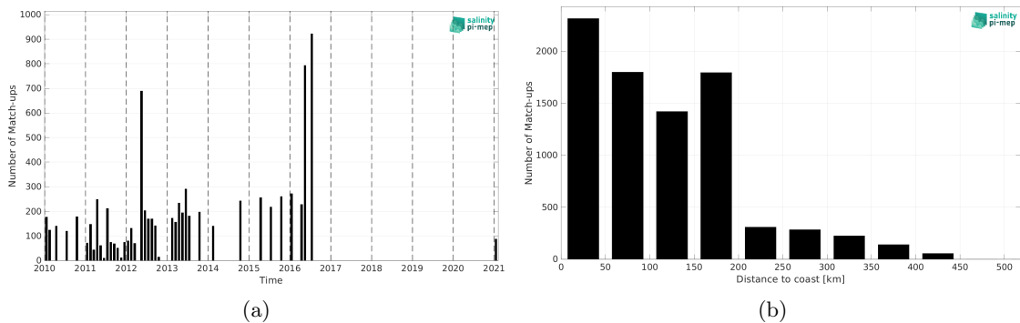
Figure 2: Number of match-ups between TSG (LEGOS-DM) and SMOS SSS L3 v9 - 9 Days (CATDS-CEC-LOCEAN) SSS as a function of time (a) and as function of the distance to coast (b) over the South China Sea Pi-MEP region and for the full satellite product period.
