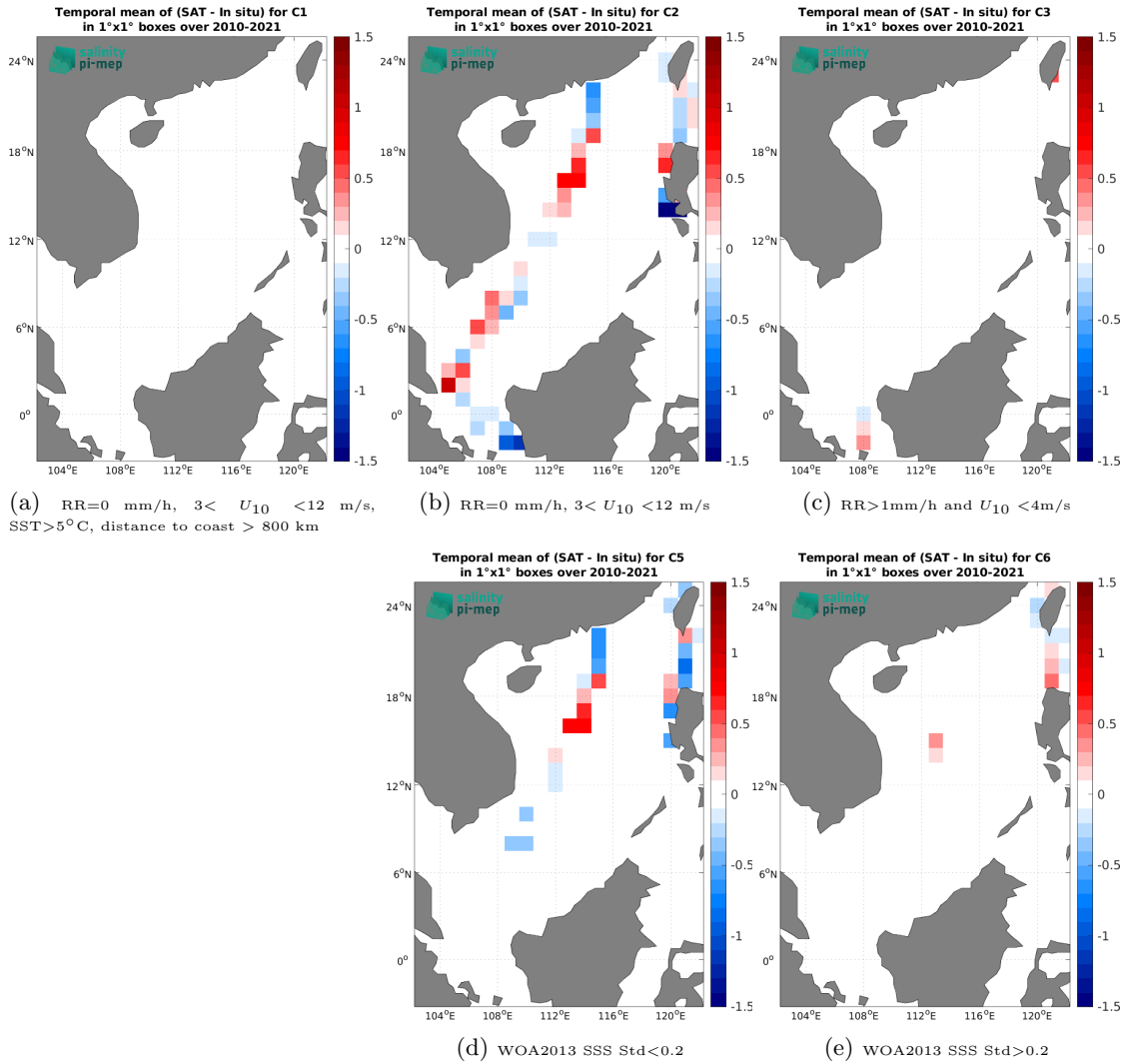
Figure 14: Temporal mean gridded over spatial boxes of size 1^\circ \times 1^\circ of \Delta SSS (SMOS SSS L3 v9 - 9 Days (CATDS-CEC-LOCEAN) - TSG (LEGOS-DM)) for 5 different subdatasets corresponding to:RR=0 mm/h, 3 < U_{10} < 12 m/s, SST>5°C, distance to coast > 800 km (a), RR=0 mm/h, 3 < U_{10} < 12 m/s (b), RR>1mm/h and U_{10} < 4 m/s (c), WOA2013 SSS Std<0.2 (d), WOA2013 SSS Std>0.2 (e).
