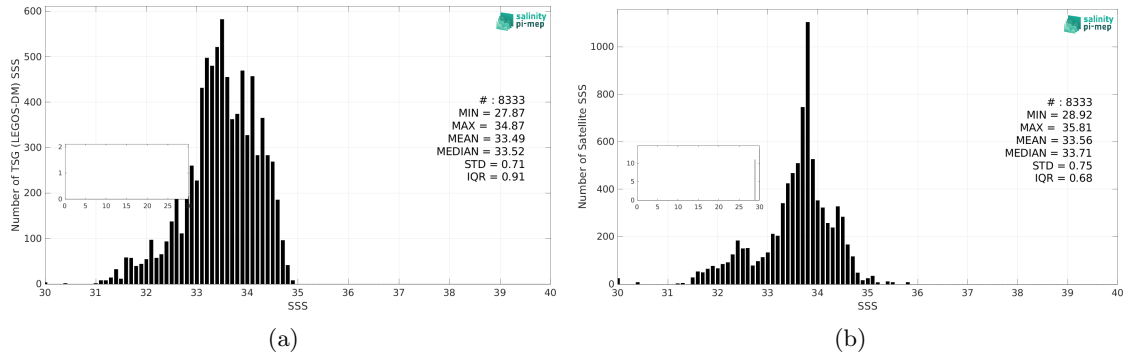
Figure 3: Histograms of SSS from TSG (LEGOS-DM) (a) and SMOS SSS L3 v9 - 9 Days (CATDS-CEC-LOCEAN) (b) considering all match-up pairs per bins of 0.1 over the South China Sea Pi-MEP region and for the full satellite product period.
