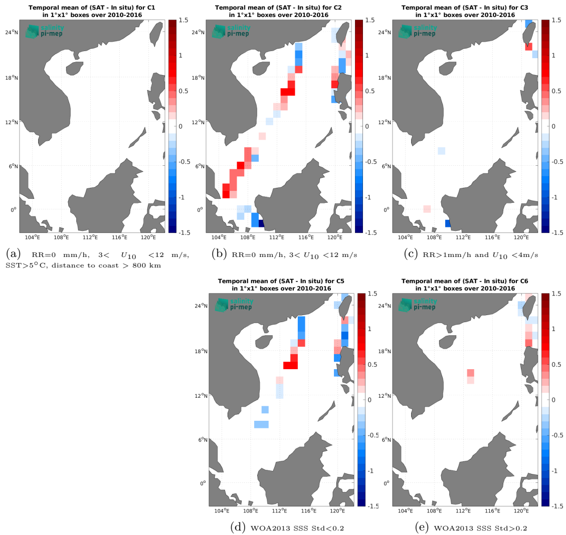
Figure 12: Temporal mean gridded over spatial boxes of size 1^\circ \times 1^\circ of \Delta\text{SSS} (SMOS SSS L3 v9 - 9 Days (CATDS-CEC-LOCEAN) - TSG (LEGOS-DM)) for 5 different subdatasets corresponding to: RR=0 mm/h, 3 < U_{10} < 12 m/s, SST > 5^\circ\text{C} , distance to coast > 800 km (a), RR=0 mm/h, 3 < U_{10} < 12 m/s (b), RR > 1 mm/h and U_{10} < 4 m/s (c), WOA2013 SSS Std < 0.2 (d), WOA2013 SSS Std > 0.2 (e).
