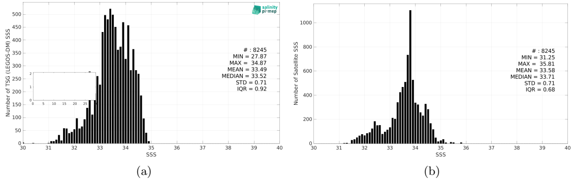
Figure 2: Histograms of SSS from TSG (LEGOS-DM) (a) and SMOS SSS L3 v9 - 9 Days (CATDS-CEC-LOCEAN) (b) considering all match-up pairs per bins of 0.1 over the South China Sea Pi-MEP region and for the full satellite product period.
