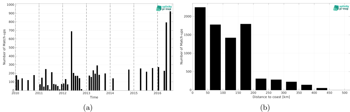
Figure 1: Number of match-ups between TSG (LEGOS-DM) and SMOS SSS L3 v9 - 9 Days (CATDS-CEC-LOCEAN) SSS as a function of time (a) and as function of the distance to coast (b) over the South China Sea Pi-MEP region and for the full satellite product period.
