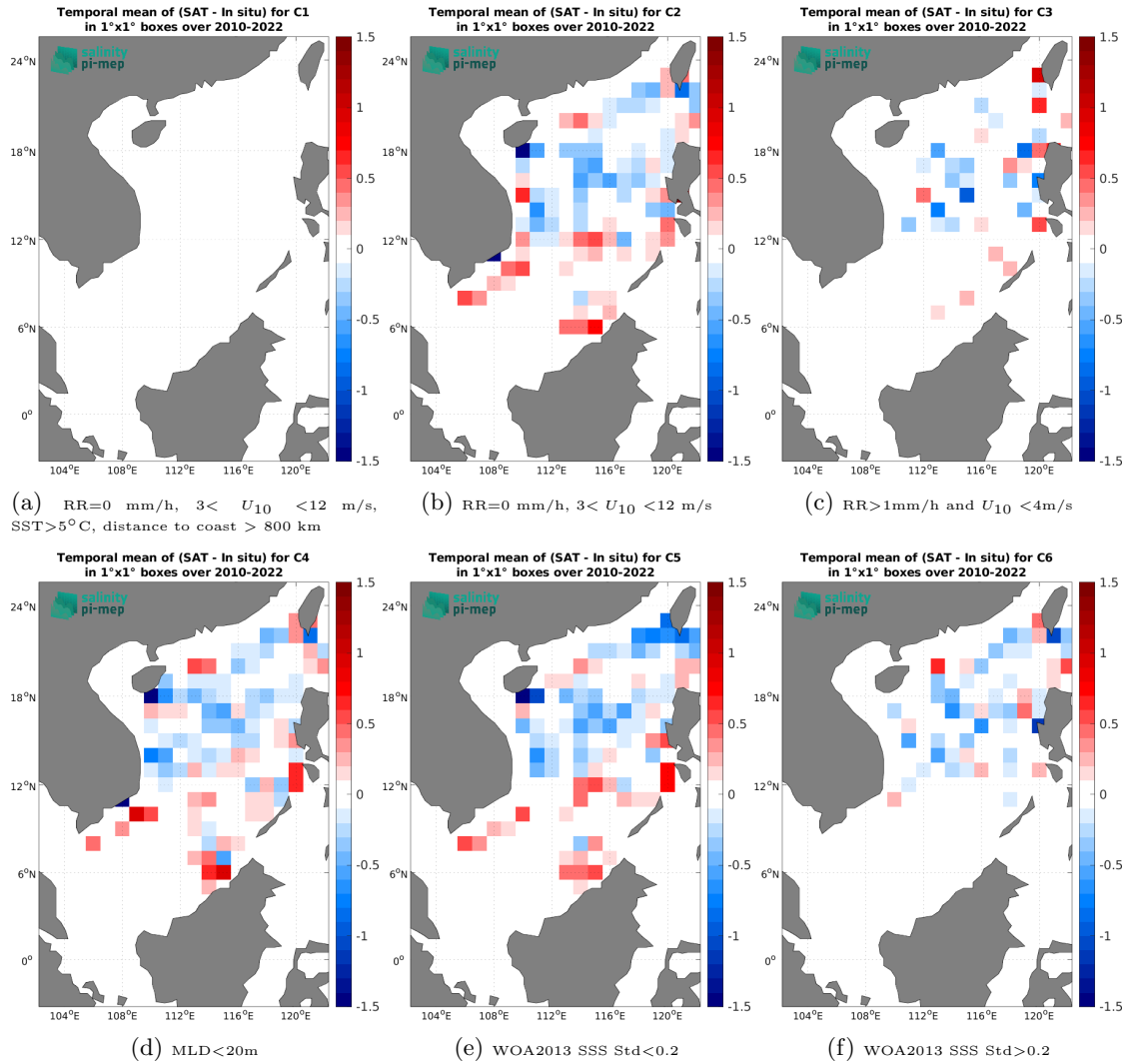
Figure 14: Temporal mean gridded over spatial boxes of size 1^\circ \times 1^\circ of \Delta SSS (SMOS SSS L3 v9 - 9 Days (CATDS-CEC-LOCEAN) - Argo) for 6 different subdatasets corresponding to:RR=0 mm/h, 3 < U_{10} < 12 m/s, SST>5°C, distance to coast > 800 km (a), RR=0 mm/h, 3 < U_{10} < 12 m/s (b), RR>1mm/h and U_{10} < 4 m/s (c),MLD<20m (d),WOA2013 SSS Std<0.2 (e),WOA2013 SSS Std>0.2 (f).
