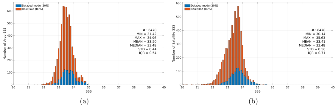
Figure 2: Histograms of SSS from Argo (a) and SMOS SSS L3 v9 - 9 Days (CATDS-CEC-LOCEAN) (b) considering all match-up pairs per bins of 0.1 over the South China Sea Pi-MEP region and for the full satellite product period.
