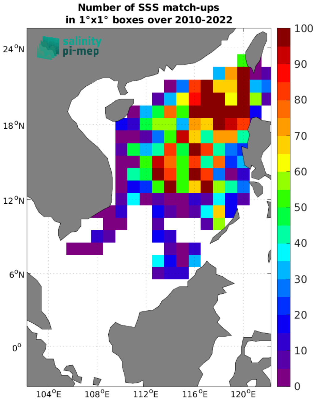
Figure 4: Number of SSS match-ups between Argo SSS and the SMOS SSS L3 v9 - 9 Days (CATDS-CEC-LOCEAN) SSS product for the South China Sea Pi-MEP region over 1^\circ \times 1^\circ boxes and for the full satellite product period.
