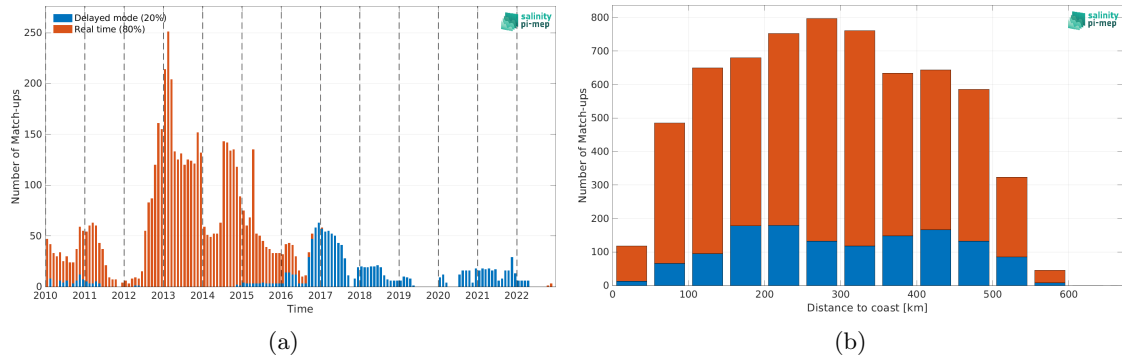
Figure 1: Number of match-ups between Argo and SMOS SSS L3 v9 - 9 Days (CATDS-CEC-LOCEAN) SSS as a function of time (a) and as function of the distance to coast (b) over the South China Sea Pi-MEP region and for the full satellite product period.
