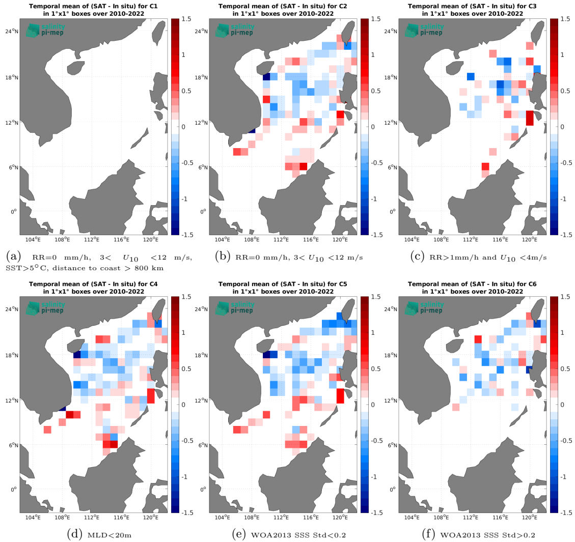
Figure 12: Temporal mean gridded over spatial boxes of size 1^\circ \times 1^\circ of \Delta\text{SSS} (SMOS SSS L3 v9 - 9 Days (CATDS-CEC-LOCEAN) - Argo) for 6 different subdatasets corresponding to: RR=0 mm/h, 3 < U_{10} < 12 m/s, SST > 5^\circ\text{C} , distance to coast > 800 km (a), RR=0 mm/h, 3 < U_{10} < 12 m/s (b), RR > 1 mm/h and U_{10} < 4 m/s (c), MLD < 20 m (d), WOA2013 SSS Std < 0.2 (e), WOA2013 SSS Std > 0.2 (f).
