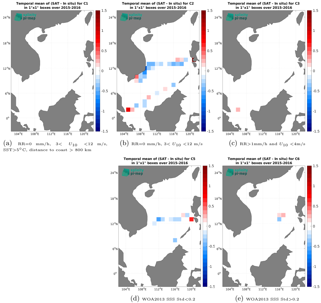
Figure 14: Temporal mean gridded over spatial boxes of size 1^\circ \times 1^\circ of \Delta\text{SSS} (SMOS SSS L3 v9 - 18 Days (CATDS-CEC-LOCEAN) - TSG (SAMOS)) for 5 different subdatasets corresponding to: RR=0 mm/h, 3 < U_{10} < 12 m/s, SST > 5^\circ\text{C} , distance to coast > 800 km (a), RR=0 mm/h, 3 < U_{10} < 12 m/s (b), RR > 1 mm/h and U_{10} < 4 m/s (c), WOA2013 SSS Std < 0.2 (d), WOA2013 SSS Std > 0.2 (e).
