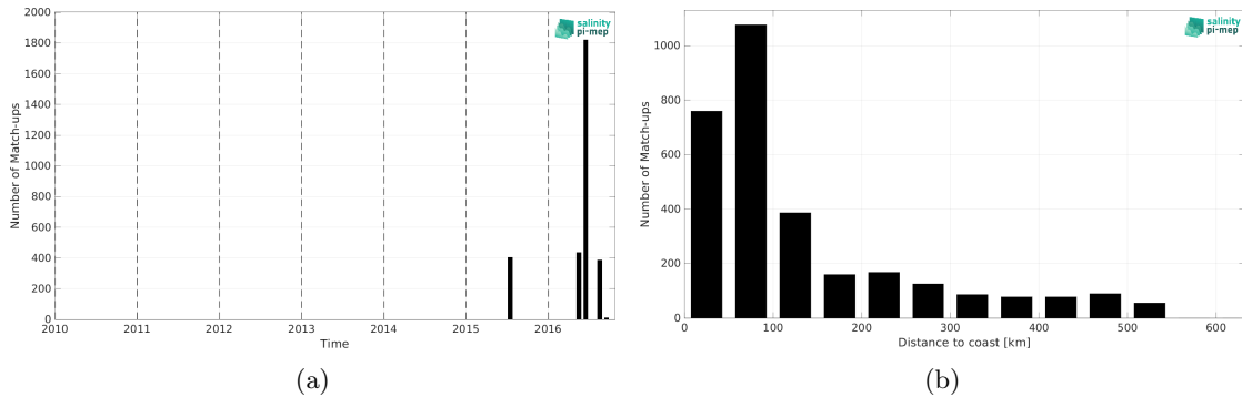
Figure 2: Number of match-ups between TSG (SAMOS) and SMOS SSS L3 v9 - 18 Days (CATDS-CEC-LOCEAN) SSS as a function of time (a) and as function of the distance to coast (b) over the South China Sea Pi-MEP region and for the full satellite product period.
