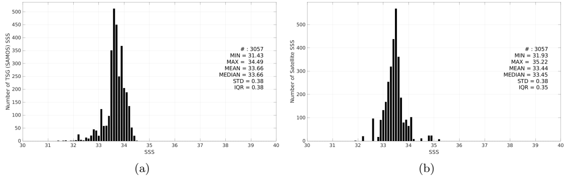
Figure 3: Histograms of SSS from TSG (SAMOS) (a) and SMOS SSS L3 v9 - 18 Days (CATDS-CEC-LOCEAN) (b) considering all match-up pairs per bins of 0.1 over the South China Sea Pi-MEP region and for the full satellite product period.
