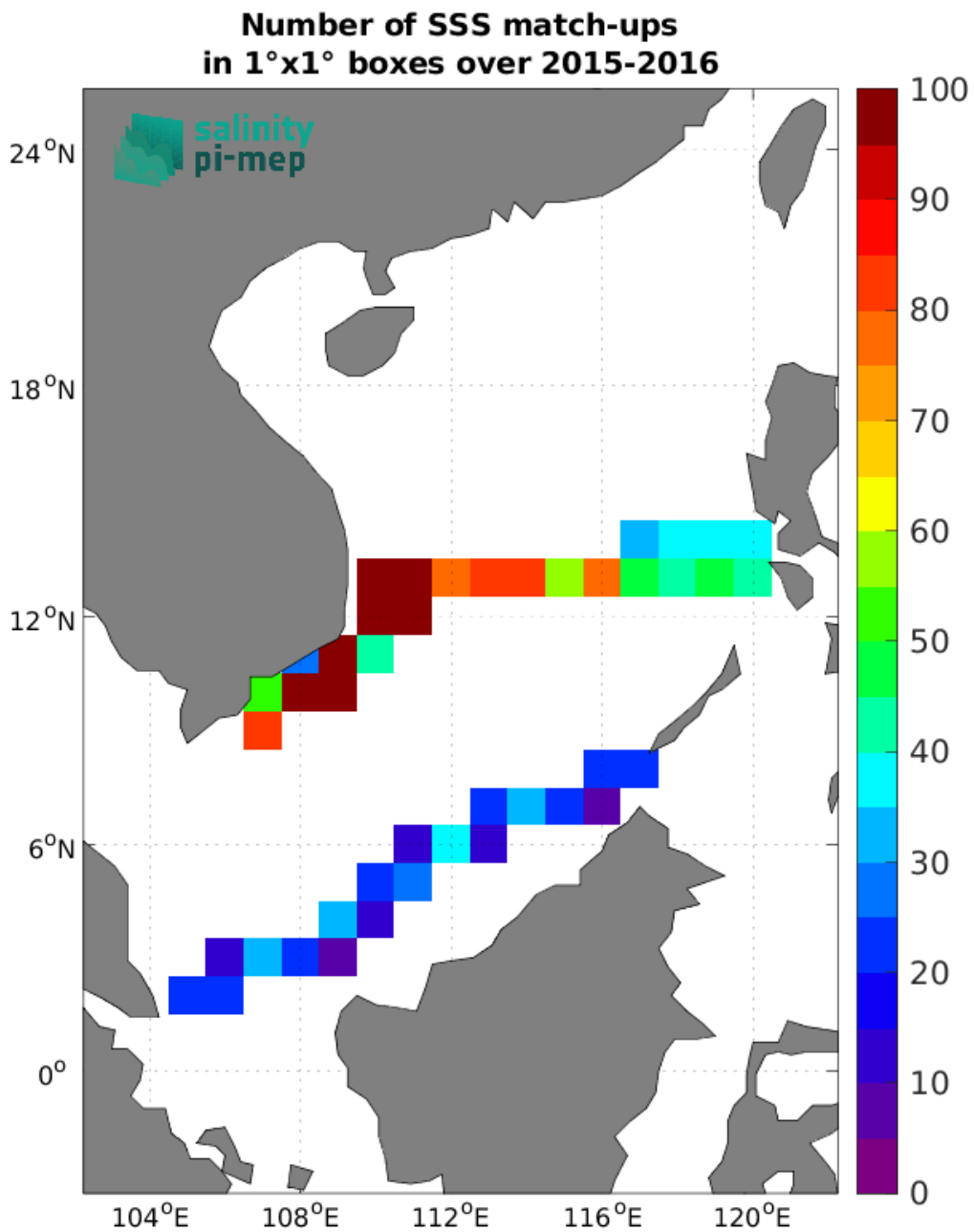
Figure 4: Number of SSS match-ups between TSG (SAMOS) SSS and the SMOS SSS L3 v9 - 18 Days (CATDS-CEC-LOCEAN) SSS product for the South China Sea Pi-MEP region over 1^\circ \times 1^\circ boxes and for the full satellite product period.
