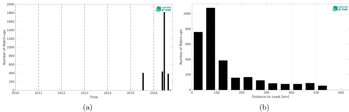
Figure 1: Number of match-ups between TSG (SAMOS) and SMOS SSS L3 v9 - 18 Days (CATDS-CEC-LOCEAN) SSS as a function of time (a) and as function of the distance to coast (b) over the South China Sea Pi-MEP region and for the full satellite product period.
