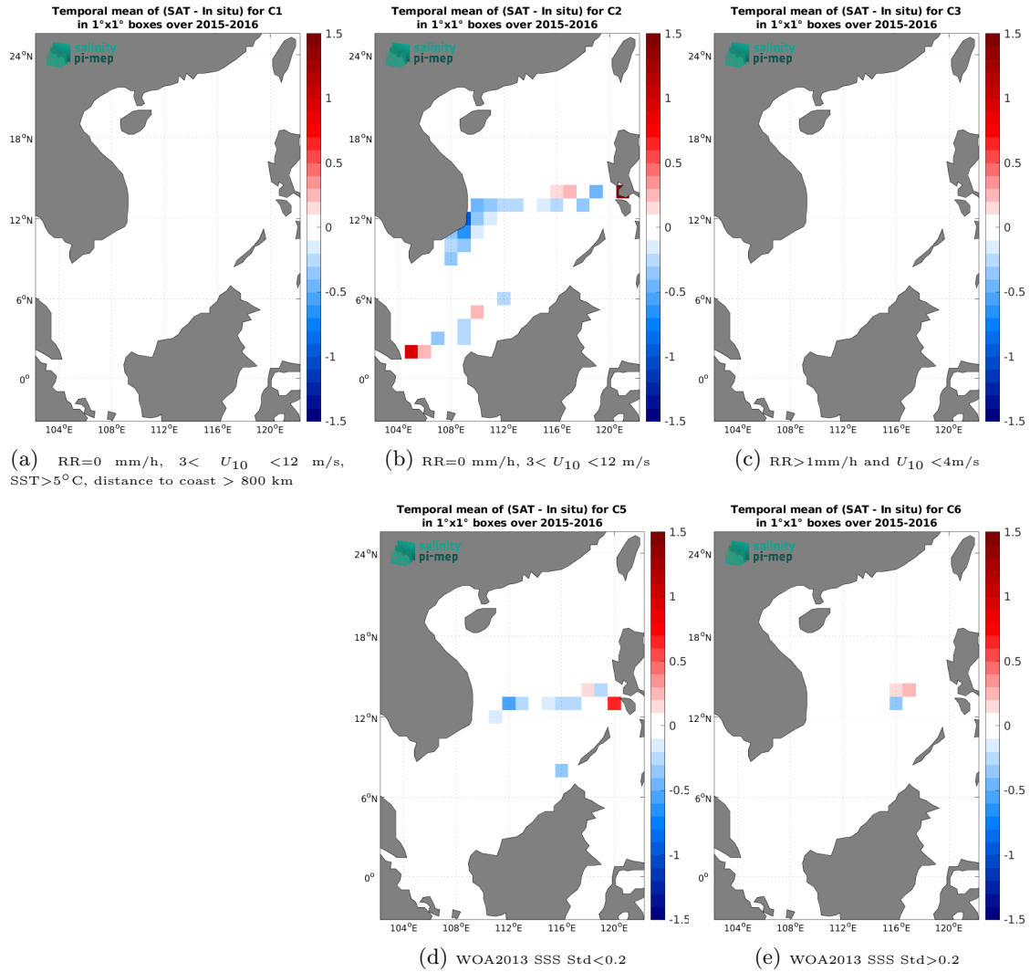
Figure 12: Temporal mean gridded over spatial boxes of size 1^\circ \times 1^\circ of \Delta\text{SSS} (SMOS SSS L3 v9 - 18 Days (CATDS-CEC-LOCEAN) - TSG (SAMOS)) for 5 different subdatasets corresponding to: RR=0 mm/h, 3 < U_{10} < 12 m/s, SST > 5^\circ\text{C} , distance to coast > 800 km (a), RR=0 mm/h, 3 < U_{10} < 12 m/s (b), RR > 1 mm/h and U_{10} < 4 m/s (c), WOA2013 SSS Std < 0.2 (d), WOA2013 SSS Std > 0.2 (e).
