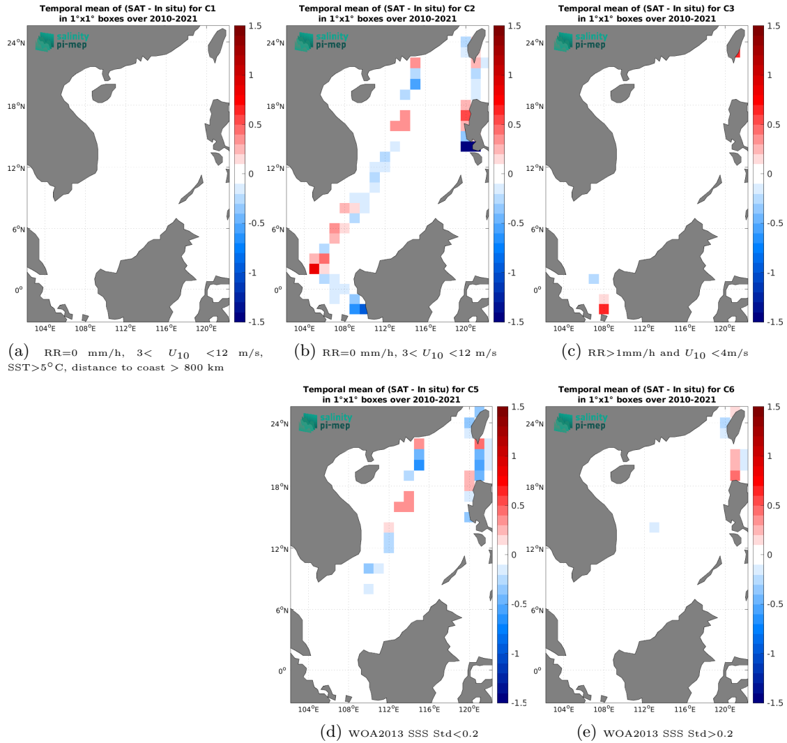
Figure 14: Temporal mean gridded over spatial boxes of size 1^\circ \times 1^\circ of \Delta SSS (SMOS SSS L3 v9 - 18 Days (CATDS-CEC-LOCEAN) - TSG (LEGOS-DM)) for 5 different subdatasets corresponding to:RR=0 mm/h, 3 < U_{10} < 12 m/s, SST>5°C, distance to coast > 800 km (a), RR=0 mm/h, 3 < U_{10} < 12 m/s (b), RR>1mm/h and U_{10} < 4 m/s (c), WOA2013 SSS Std<0.2 (d), WOA2013 SSS Std>0.2 (e).
