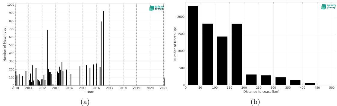
Figure 2: Number of match-ups between TSG (LEGOS-DM) and SMOS SSS L3 v9 - 18 Days (CATDS-CEC-LOCEAN) SSS as a function of time (a) and as function of the distance to coast (b) over the South China Sea Pi-MEP region and for the full satellite product period.
