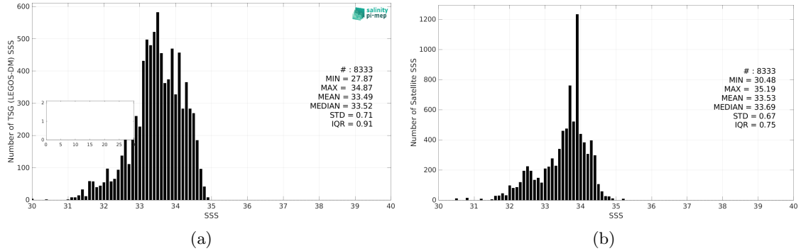
Figure 3: Histograms of SSS from TSG (LEGOS-DM) (a) and SMOS SSS L3 v9 - 18 Days (CATDS-CEC-LOCEAN) (b) considering all match-up pairs per bins of 0.1 over the South China Sea Pi-MEP region and for the full satellite product period.
