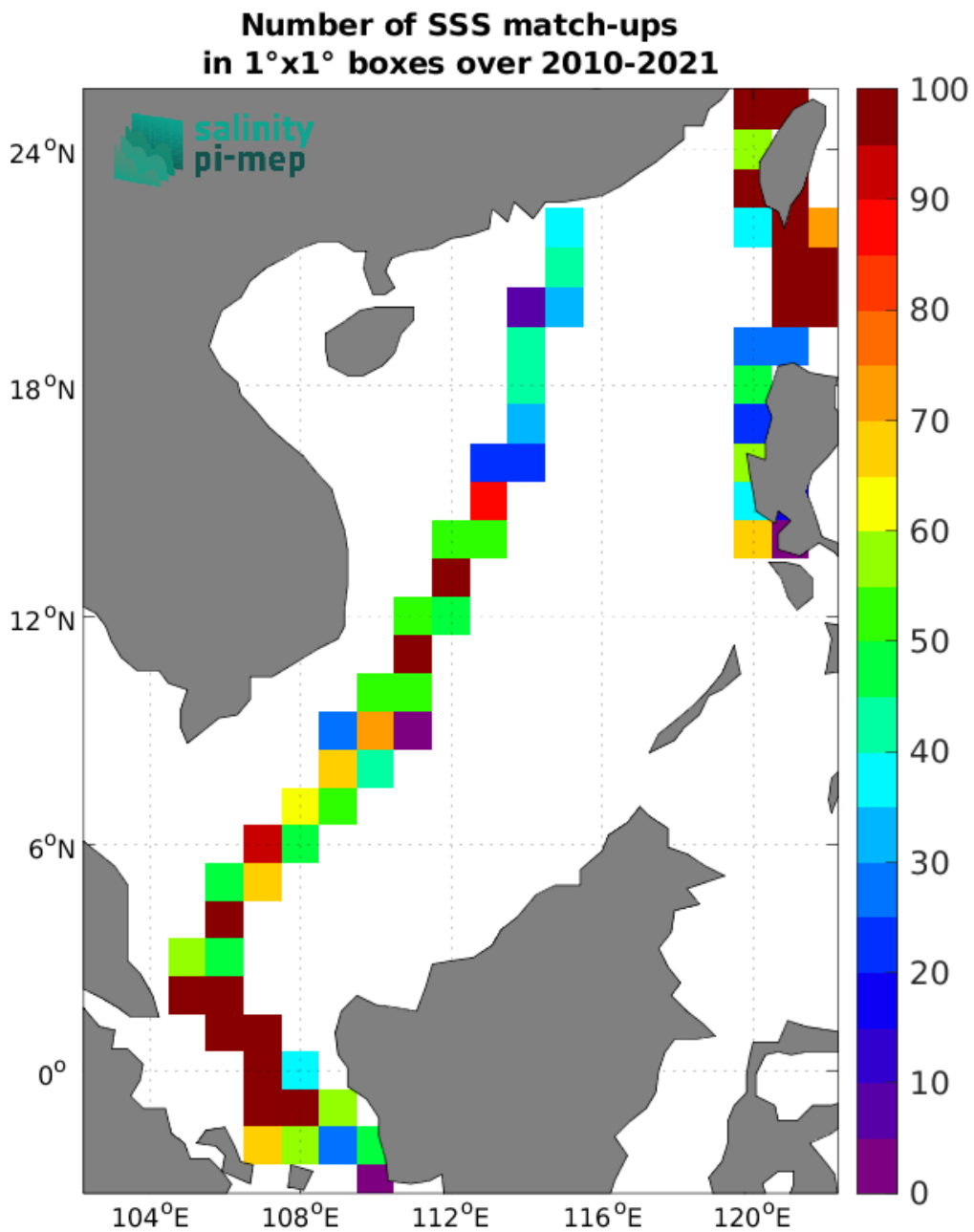
Figure 5: Number of SSS match-ups between TSG (LEGOS-DM) SSS and the SMOS SSS L3 v9 - 18 Days (CATDS-CEC-LOCEAN) SSS product for the South China Sea Pi-MEP region over 1°x1° boxes and for the full satellite product period.
