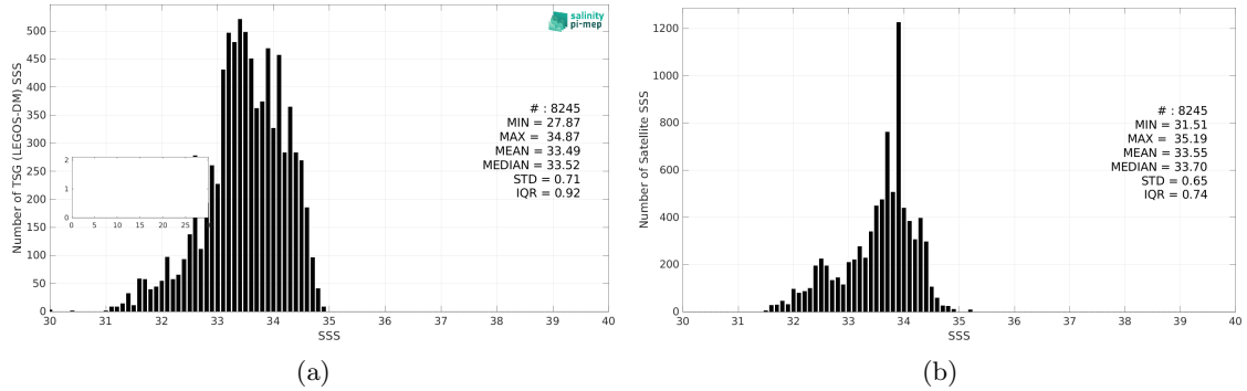
Figure 2: Histograms of SSS from TSG (LEGOS-DM) (a) and SMOS SSS L3 v9 - 18 Days (CATDS-CEC-LOCEAN) (b) considering all match-up pairs per bins of 0.1 over the South China Sea Pi-MEP region and for the full satellite product period.
