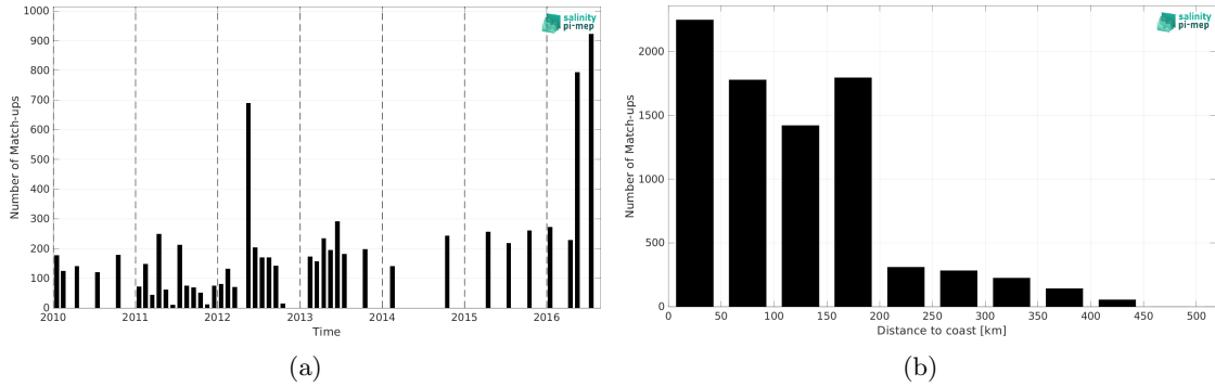
Figure 1: Number of match-ups between TSG (LEGOS-DM) and SMOS SSS L3 v9 - 18 Days (CATDS-CEC-LOCEAN) SSS as a function of time (a) and as function of the distance to coast (b) over the South China Sea Pi-MEP region and for the full satellite product period.
