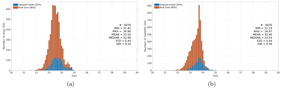
Figure 3: Histograms of SSS from Argo (a) and SMOS SSS L3 v9 - 18 Days (CATDS-CEC-LOCEAN) (b) considering all match-up pairs per bins of 0.1 over the South China Sea Pi-MEP region and for the full satellite product period.
