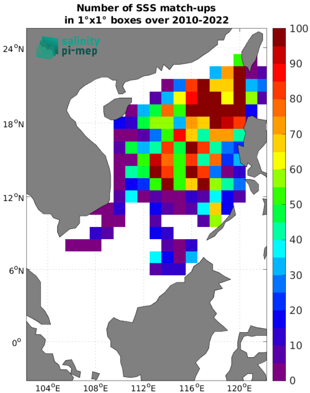
Figure 5: Number of SSS match-ups between Argo SSS and the SMOS SSS L3 v9 - 18 Days (CATDS-CEC-LOCEAN) SSS product for the South China Sea Pi-MEP region over 1°x1° boxes and for the full satellite product period.
