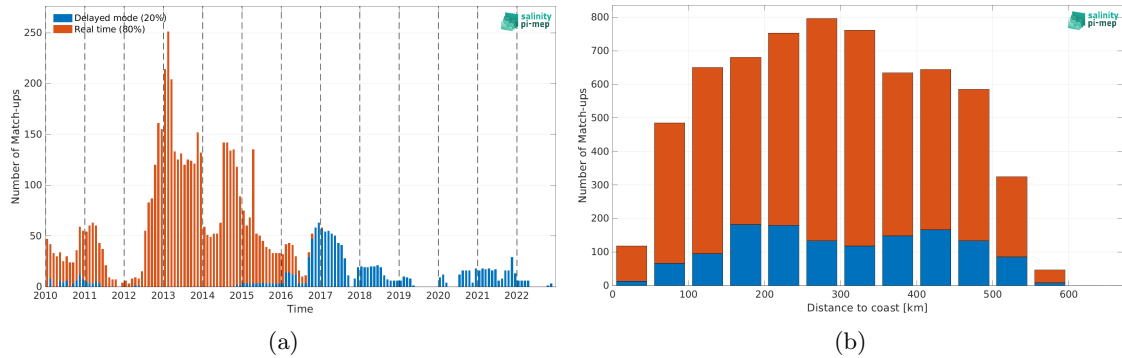
Figure 2: Number of match-ups between Argo and SMOS SSS L3 v9 - 18 Days (CATDS-CEC-LOCEAN) SSS as a function of time (a) and as function of the distance to coast (b) over the South China Sea Pi-MEP region and for the full satellite product period.
