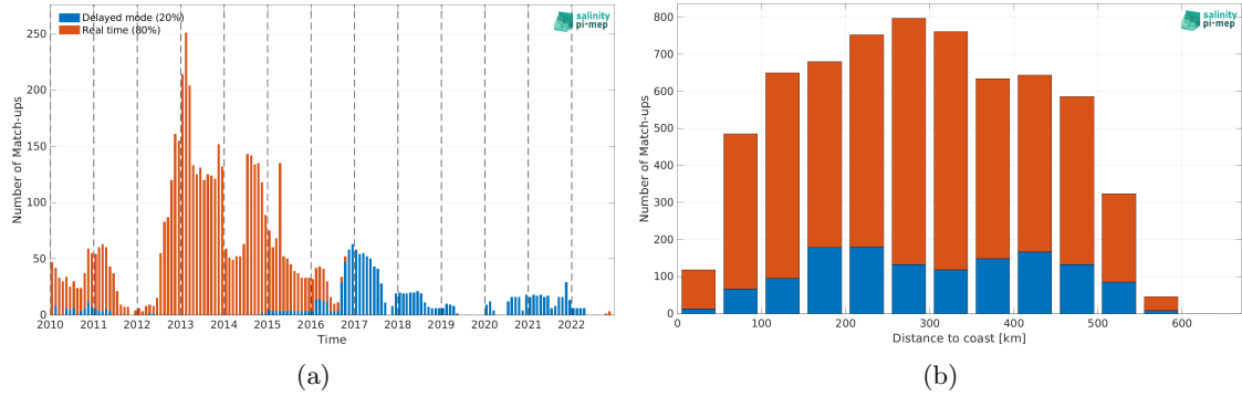
Figure 1: Number of match-ups between Argo and SMOS SSS L3 v9 - 18 Days (CATDS-CEC-LOCEAN) SSS as a function of time (a) and as function of the distance to coast (b) over the South China Sea Pi-MEP region and for the full satellite product period.
