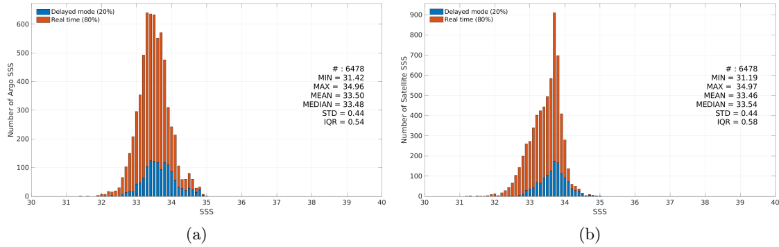
Figure 2: Histograms of SSS from Argo (a) and SMOS SSS L3 v9 - 18 Days (CATDS-CEC-LOCEAN) (b) considering all match-up pairs per bins of 0.1 over the South China Sea Pi-MEP region and for the full satellite product period.
