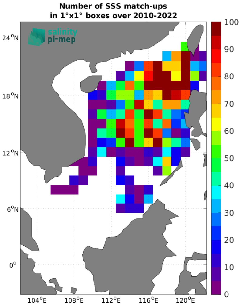
Figure 4: Number of SSS match-ups between Argo SSS and the SMOS SSS L3 v9 - 18 Days (CATDS-CEC-LOCEAN) SSS product for the South China Sea Pi-MEP region over 1^{\circ} \times 1^{\circ} boxes and for the full satellite product period.
