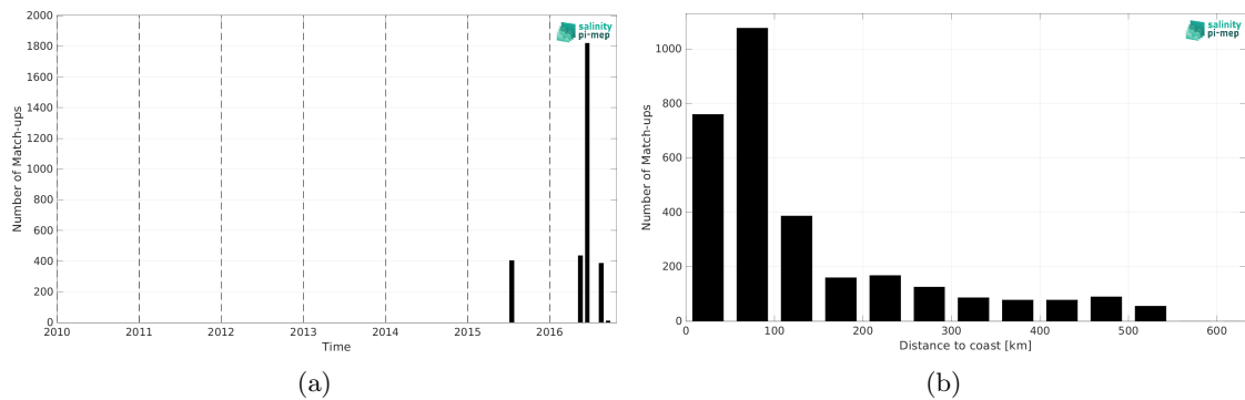
Figure 1: Number of match-ups between TSG (SAMOS) and SMOS SSS L3 v8 - 9 Days (CATDS-CEC-LOCEAN) SSS as a function of time (a) and as function of the distance to coast (b) over the South China Sea Pi-MEP region and for the full satellite product period.
