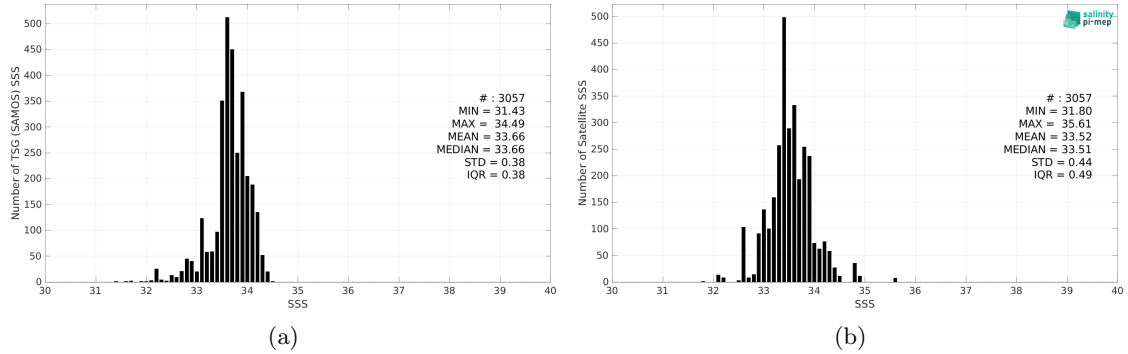
Figure 2: Histograms of SSS from TSG (SAMOS) (a) and SMOS SSS L3 v8 - 9 Days (CATDS-CEC-LOCEAN) (b) considering all match-up pairs per bins of 0.1 over the South China Sea Pi-MEP region and for the full satellite product period.
