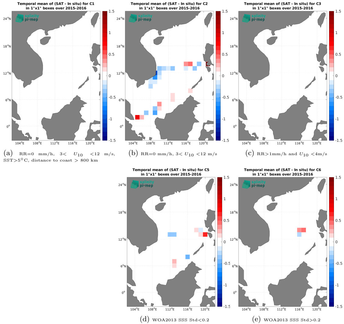
Figure 12: Temporal mean gridded over spatial boxes of size 1^\circ \times 1^\circ of \Delta SSS (SMOS SSS L3 v8 - 9 Days (CATDS-CEC-LOCEAN) - TSG (SAMOS)) for 5 different subdatasets corresponding to:RR=0 mm/h, 3 < U_{10} < 12 m/s, SST>5°C, distance to coast > 800 km (a), RR=0 mm/h, 3 < U_{10} < 12 m/s (b), RR>1mm/h and U_{10} < 4 m/s (c), WOA2013 SSS Std<0.2 (d), WOA2013 SSS Std>0.2 (e).
