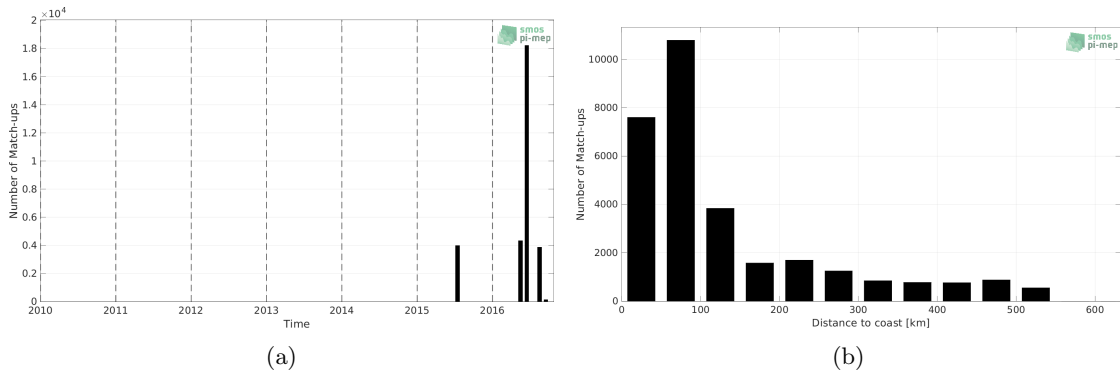
Figure 1: Number of match-ups between TSG (SAMOS) and SMOS SSS L3 v8 - 9 Days (CATDS-CECOS-LOCEAN) SSS as a function of time (a) and as function of the distance to coast (b) over the South China Sea Pi-MEP region and for the full satellite product period.
