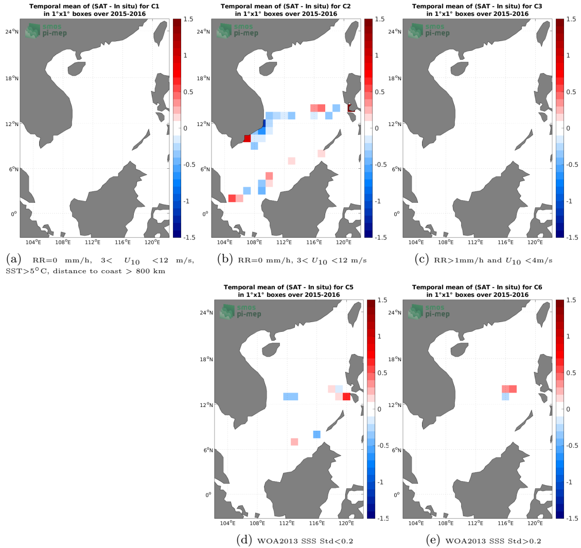
Figure 12: Temporal mean gridded over spatial boxes of size 1^\circ \times 1^\circ of \Delta SSS (SMOS SSS L3 v8 - 9 Days (CATDS-CECOS-LOCEAN) - TSG (SAMOS)) for 5 different subdatasets corresponding to:RR=0 mm/h, 3 < U_{10} < 12 m/s, SST>5°C, distance to coast > 800 km (a), RR=0 mm/h, 3 < U_{10} < 12 m/s (b), RR>1mm/h and U_{10} < 4 m/s (c), WOA2013 SSS Std<0.2 (d), WOA2013 SSS Std>0.2 (e).
