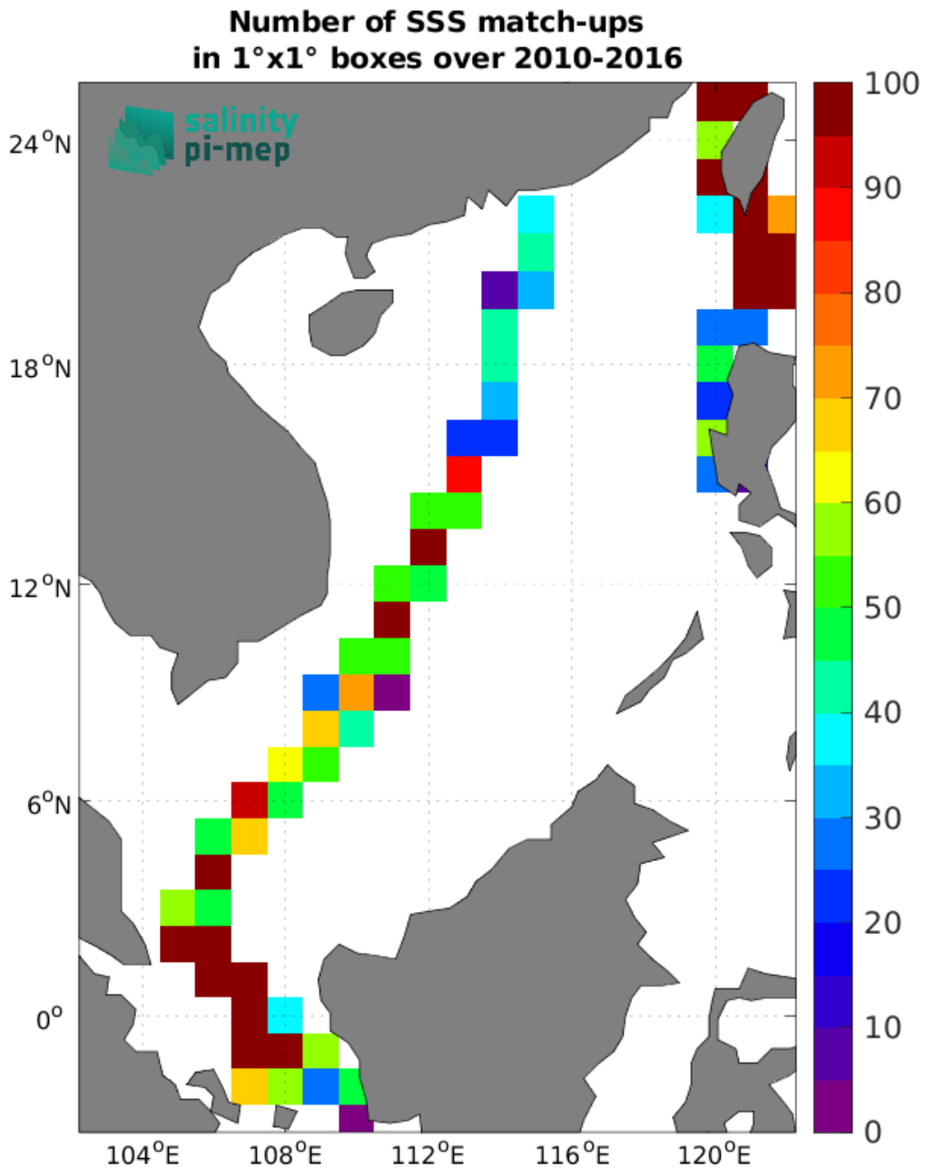
Figure 4: Number of SSS match-ups between TSG (LEGOS-DM) SSS and the SMOS SSS L3 v8 - 9 Days (CATDS-CEC-LOCEAN) SSS product for the South China Sea Pi-MEP region over 1^\circ \times 1^\circ boxes and for the full satellite product period.
