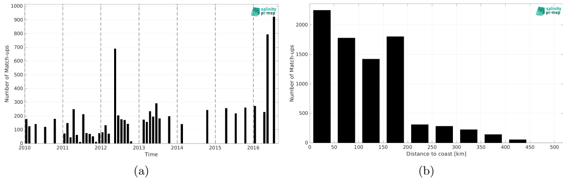
Figure 1: Number of match-ups between TSG (LEGOS-DM) and SMOS SSS L3 v8 - 9 Days (CATDS-CEC-LOCEAN) SSS as a function of time (a) and as function of the distance to coast (b) over the South China Sea Pi-MEP region and for the full satellite product period.
