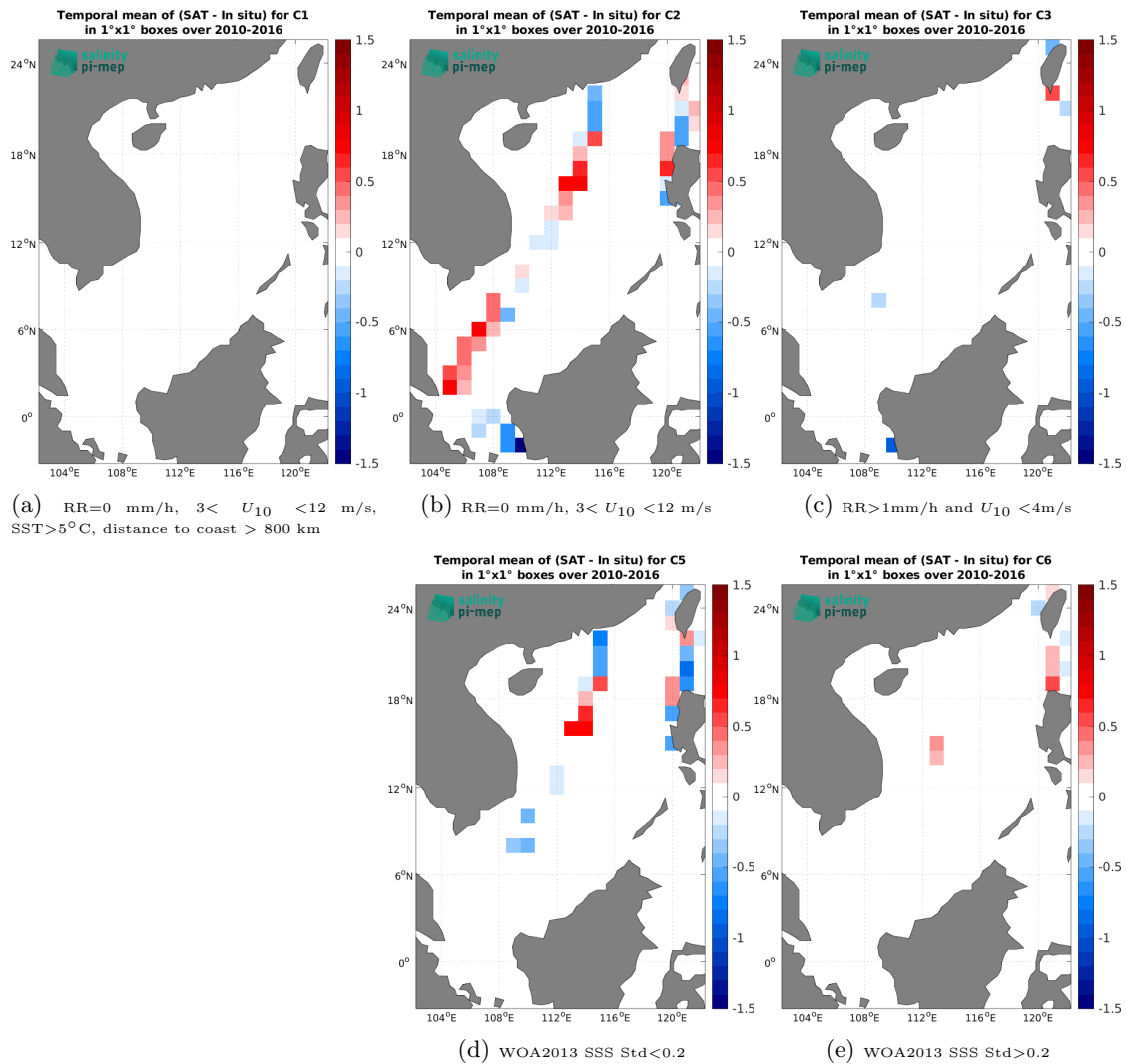
Figure 12: Temporal mean gridded over spatial boxes of size 1^\circ \times 1^\circ of \Delta SSS (SMOS SSS L3 v8 - 9 Days (CATDS-CEC-LOCEAN) - TSG (LEGOS-DM)) for 5 different subdatasets corresponding to:RR=0 mm/h, 3 < U_{10} < 12 m/s, SST>5°C, distance to coast > 800 km (a), RR=0 mm/h, 3 < U_{10} < 12 m/s (b), RR>1mm/h and U_{10} < 4 m/s (c), WOA2013 SSS Std<0.2 (d), WOA2013 SSS Std>0.2 (e).
