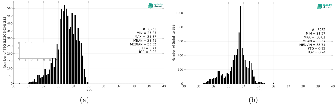
Figure 2: Histograms of SSS from TSG (LEGOS-DM) (a) and SMOS SSS L3 v8 - 9 Days (CATDS-CEC-LOCEAN) (b) considering all match-up pairs per bins of 0.1 over the South China Sea Pi-MEP region and for the full satellite product period.
