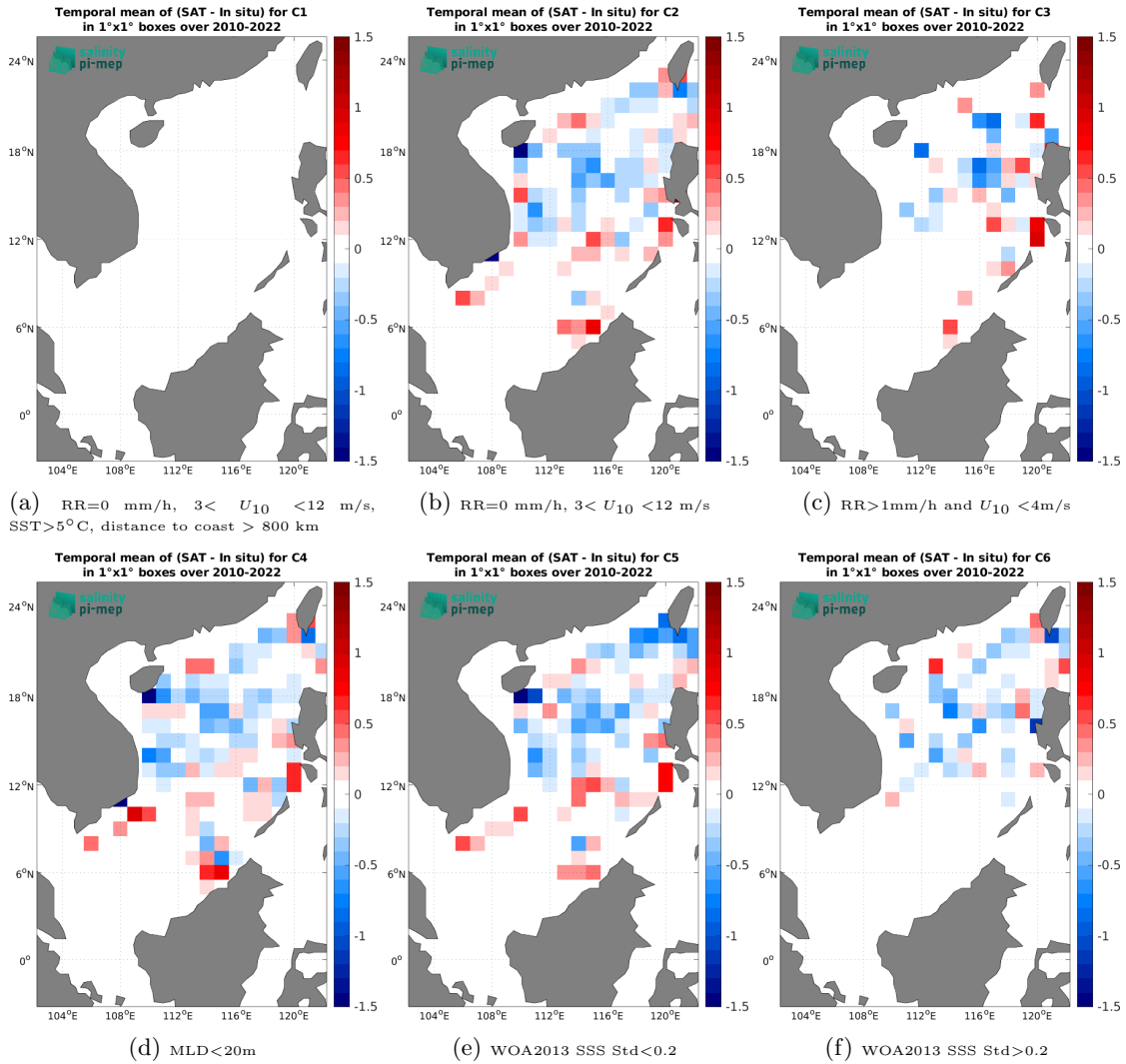
Figure 12: Temporal mean gridded over spatial boxes of size 1^\circ \times 1^\circ of \Delta SSS (SMOS SSS L3 v8 - 9 Days (CATDS-CEC-LOCEAN) - Argo) for 6 different subdatasets corresponding to: RR=0 mm/h, 3 < U_{10} < 12 m/s, SST > 5^\circ\text{C} , distance to coast > 800 km (a), RR=0 mm/h, 3 < U_{10} < 12 m/s (b), RR > 1 mm/h and U_{10} < 4 m/s (c), MLD < 20 m (d), WOA2013 SSS Std < 0.2 (e), WOA2013 SSS Std > 0.2 (f).
