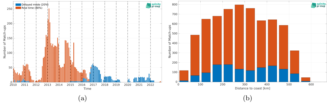
Figure 1: Number of match-ups between Argo and SMOS SSS L3 v8 - 9 Days (CATDS-CEC-LOCEAN) SSS as a function of time (a) and as function of the distance to coast (b) over the South China Sea Pi-MEP region and for the full satellite product period.
