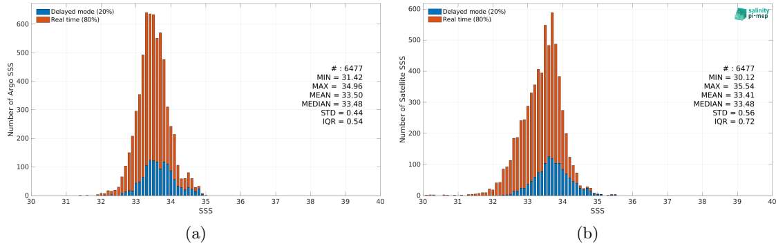
Figure 2: Histograms of SSS from Argo (a) and SMOS SSS L3 v8 - 9 Days (CATDS-CEC-LOCEAN) (b) considering all match-up pairs per bins of 0.1 over the South China Sea Pi-MEP region and for the full satellite product period.
