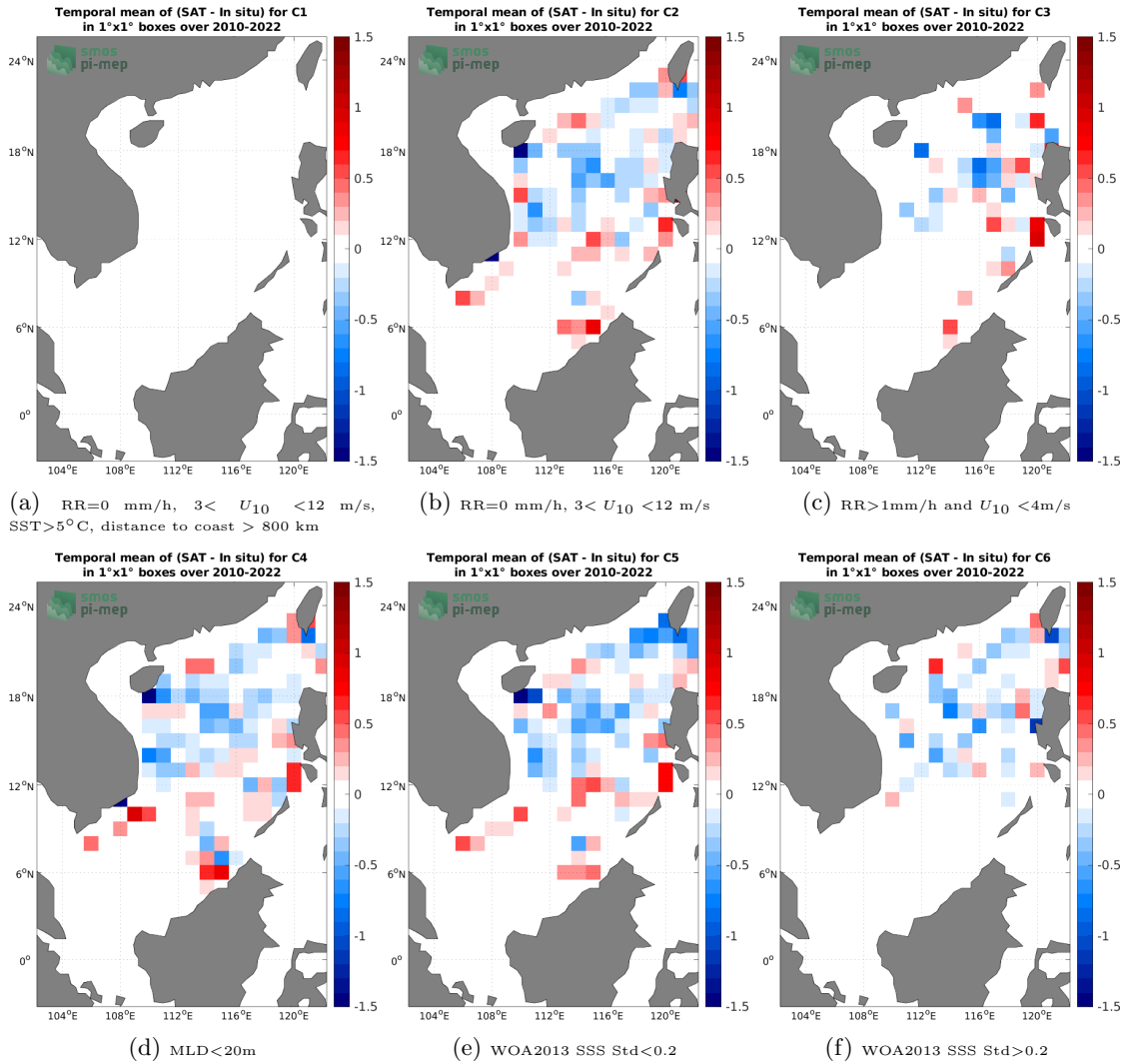
Figure 12: Temporal mean gridded over spatial boxes of size 1^\circ \times 1^\circ of \Delta SSS (SMOS SSS L3 v8 - 9 Days (CATDS-CECOS-LOCEAN) - Argo) for 6 different subdatasets corresponding to:RR=0 mm/h, 3 < U_{10} < 12 m/s, SST>5°C, distance to coast > 800 km (a), RR=0 mm/h, 3 < U_{10} < 12 m/s (b), RR>1mm/h and U_{10} < 4 m/s (c),MLD<20m (d),WOA2013 SSS Std<0.2 (e),WOA2013 SSS Std>0.2 (f).
