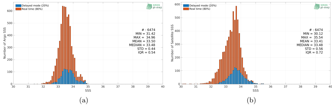
Figure 2: Histograms of SSS from Argo (a) and SMOS SSS L3 v8 - 9 Days (CATDS-CECOS-LOCEAN) (b) considering all match-up pairs per bins of 0.1 over the South China Sea Pi-MEP region and for the full satellite product period.
