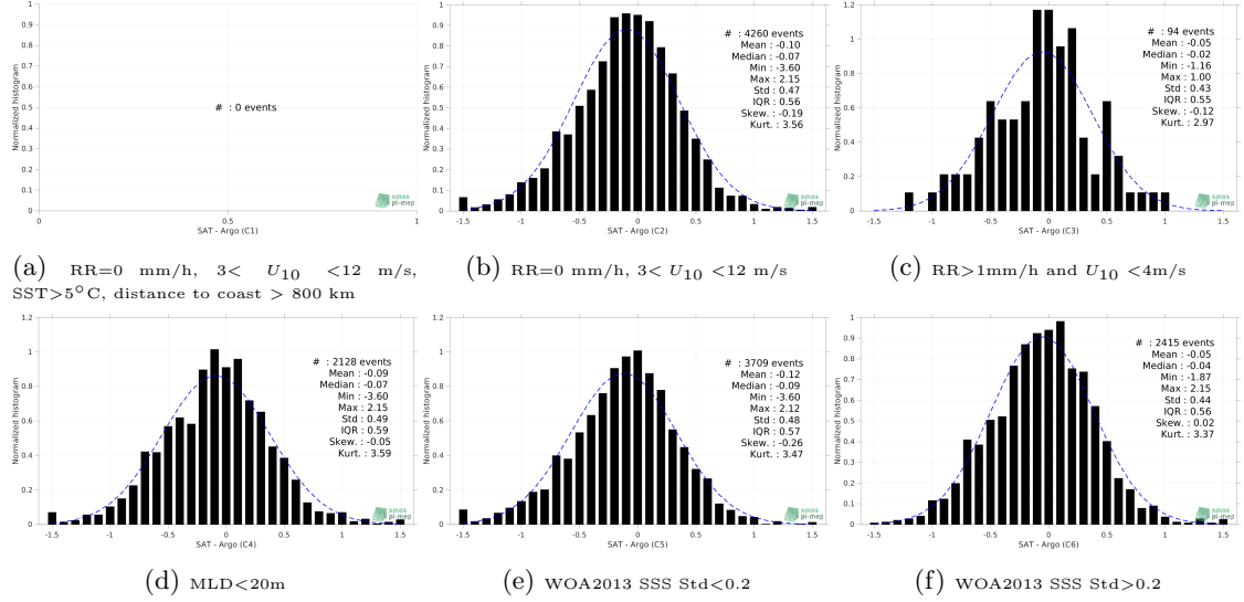
Figure 13: Normalized histogram of \Delta SSS (SMOS SSS L3 v8 - 9 Days (CATDS-CECOS-LOCEAN) - Argo) for 6 different subdatasets corresponding to: RR=0 mm/h, 3 < U_{10} < 12 m/s, SST>5°C, distance to coast > 800 km (a), RR=0 mm/h, 3 < U_{10} < 12 m/s (b), RR>1mm/h and U_{10} < 4 m/s (c), MLD<20m (d), WOA2013 SSS Std<0.2 (e), WOA2013 SSS Std>0.2 (f).
