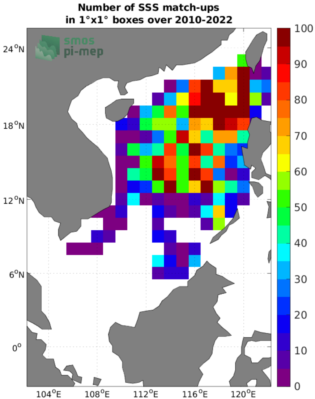
Figure 4: Number of SSS match-ups between Argo SSS and the SMOS SSS L3 v8 - 9 Days (CATDS-CECOS-LOCEAN) SSS product for the South China Sea Pi-MEP region over 1^\circ \times 1^\circ boxes and for the full satellite product period.
