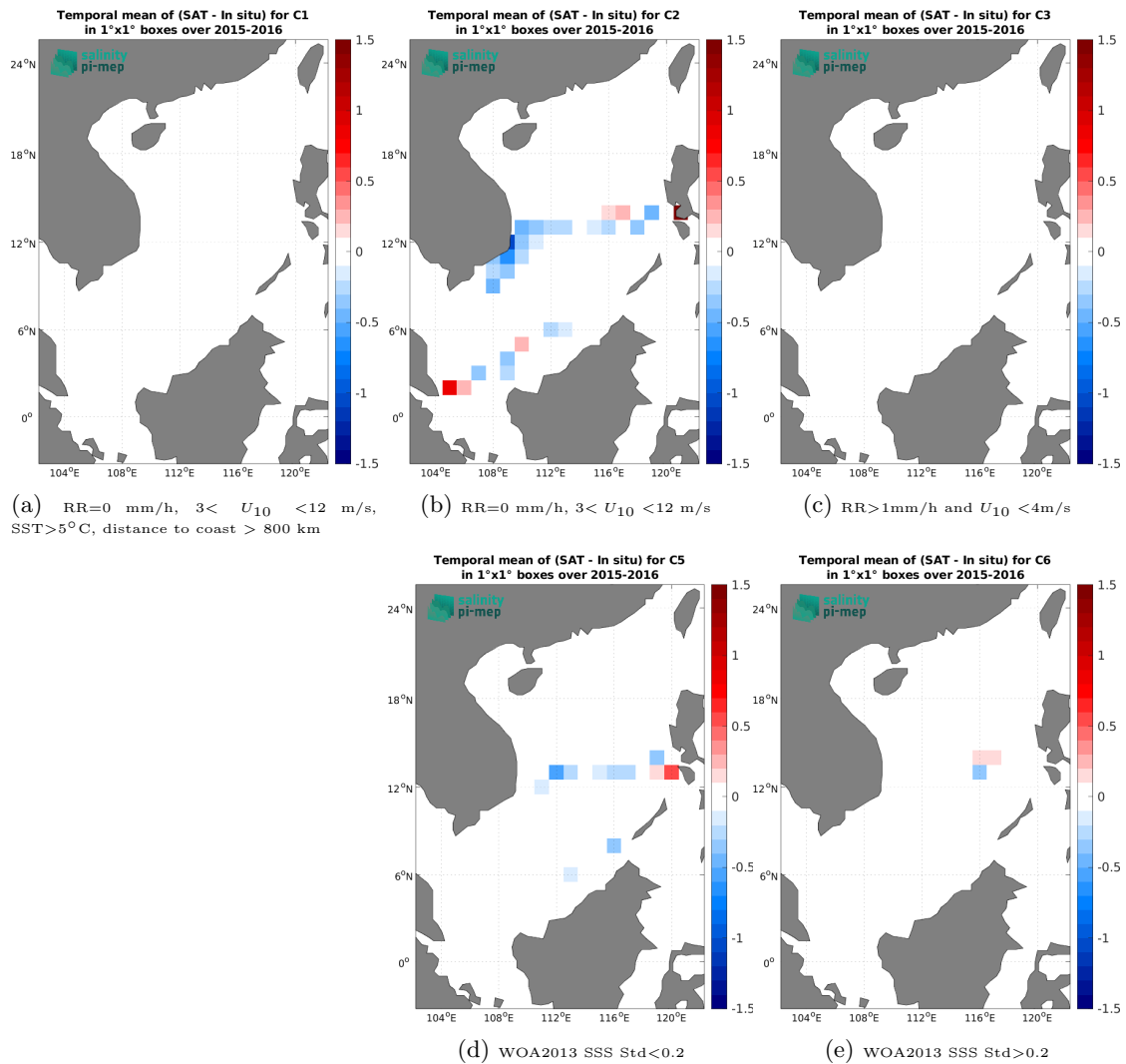
Figure 12: Temporal mean gridded over spatial boxes of size 1^\circ \times 1^\circ of \Delta\text{SSS} (SMOS SSS L3 v8 - 18 Days (CATDS-CEC-LOCEAN) - TSG (SAMOS)) for 5 different subdatasets corresponding to: RR=0 mm/h, 3 < U_{10} < 12 m/s, SST > 5^\circ\text{C} , distance to coast > 800 km (a), RR=0 mm/h, 3 < U_{10} < 12 m/s (b), RR > 1 mm/h and U_{10} < 4 m/s (c), WOA2013 SSS Std < 0.2 (d), WOA2013 SSS Std > 0.2 (e).
