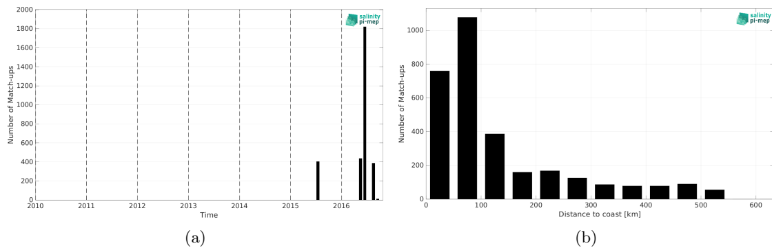
Figure 1: Number of match-ups between TSG (SAMOS) and SMOS SSS L3 v8 - 18 Days (CATDS-CEC-LOCEAN) SSS as a function of time (a) and as function of the distance to coast (b) over the South China Sea Pi-MEP region and for the full satellite product period.
