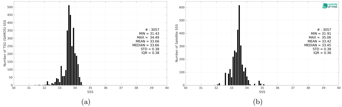
Figure 2: Histograms of SSS from TSG (SAMOS) (a) and SMOS SSS L3 v8 - 18 Days (CATDS-CEC-LOCEAN) (b) considering all match-up pairs per bins of 0.1 over the South China Sea Pi-MEP region and for the full satellite product period.
