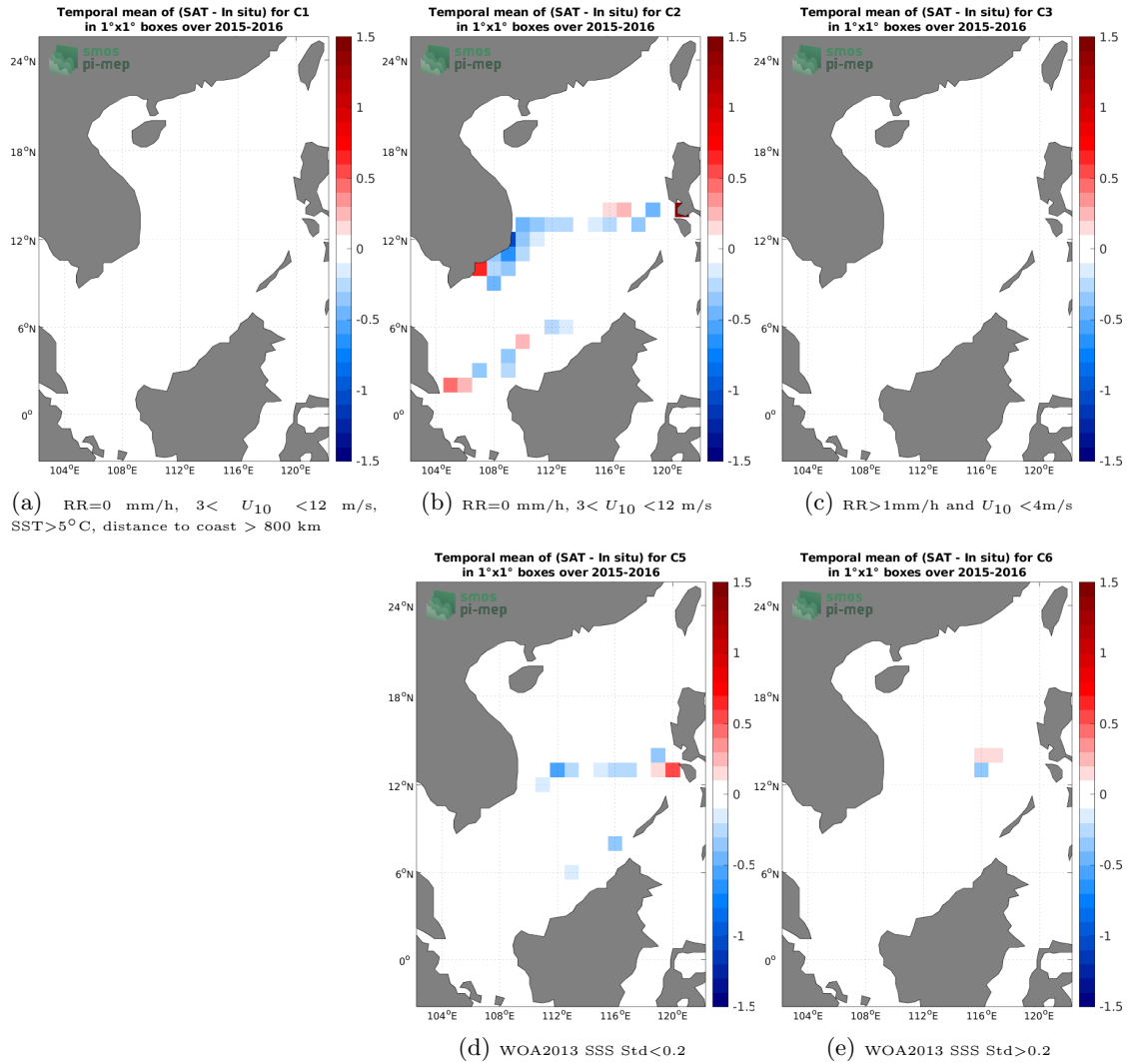
Figure 12: Temporal mean gridded over spatial boxes of size 1^\circ \times 1^\circ of \Delta SSS (SMOS SSS L3 v8 - 18 Days (CATDS-CECOS-LOCEAN) - TSG (SAMOS)) for 5 different subdatasets corresponding to: RR=0 mm/h, 3 < U_{10} < 12 m/s, SST > 5^\circ C , distance to coast > 800 km (a), RR=0 mm/h, 3 < U_{10} < 12 m/s (b), RR > 1 mm/h and U_{10} < 4 m/s (c), WOA2013 SSS Std < 0.2 (d), WOA2013 SSS Std > 0.2 (e).
