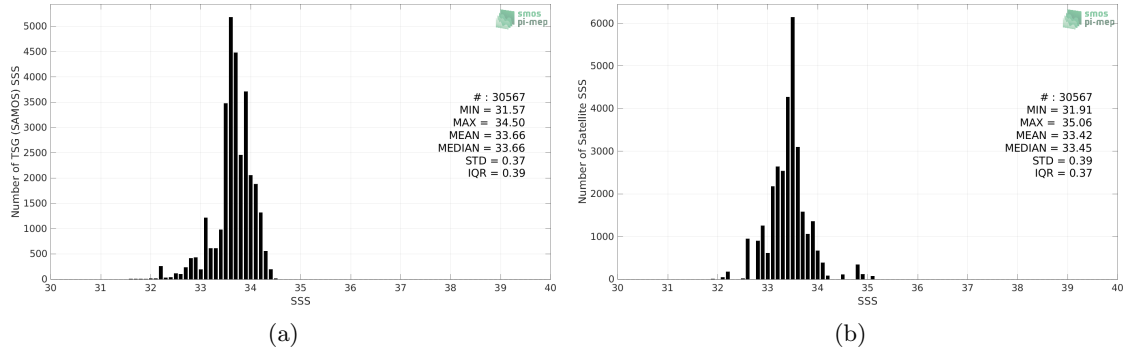
Figure 2: Histograms of SSS from TSG (SAMOS) (a) and SMOS SSS L3 v8 - 18 Days (CATDS-CECOS-LOCEAN) (b) considering all match-up pairs per bins of 0.1 over the South China Sea Pi-MEP region and for the full satellite product period.
