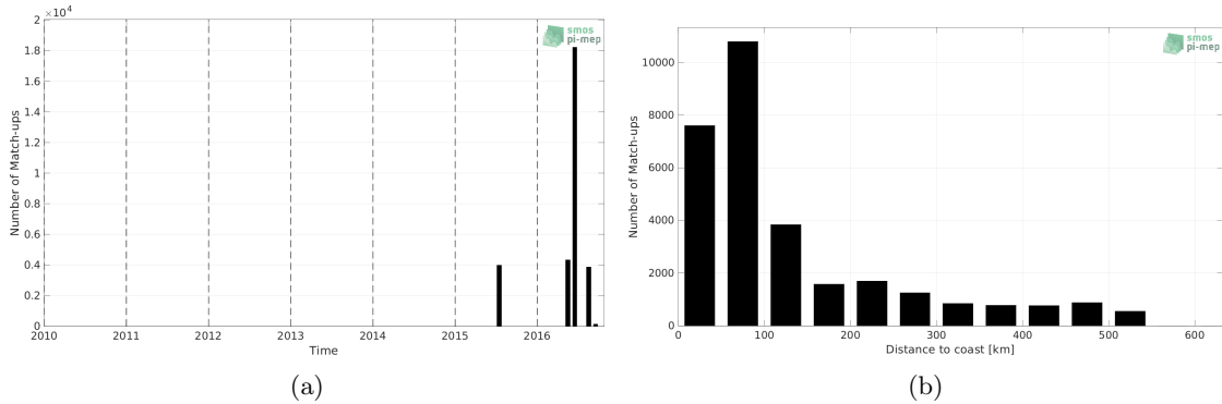
Figure 1: Number of match-ups between TSG (SAMOS) and SMOS SSS L3 v8 - 18 Days (CATDS-CECOS-LOCEAN) SSS as a function of time (a) and as function of the distance to coast (b) over the South China Sea Pi-MEP region and for the full satellite product period.
