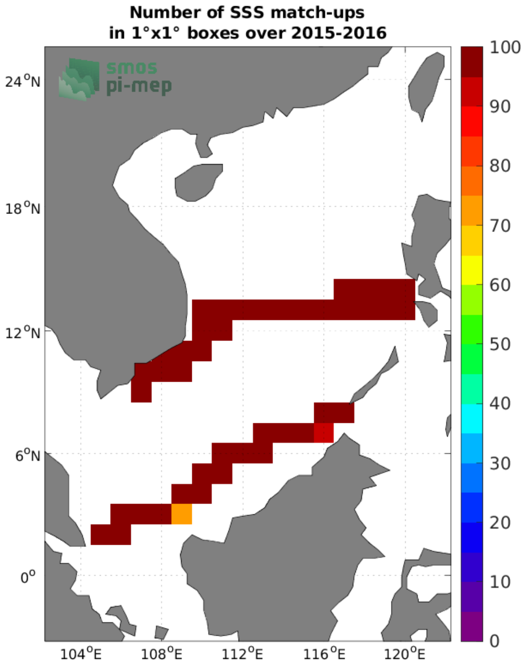
Figure 4: Number of SSS match-ups between TSG (SAMOS) SSS and the SMOS SSS L3 v8 - 18 Days (CATDS-CECOS-LOCEAN) SSS product for the South China Sea Pi-MEP region over 1°x1° boxes and for the full satellite product period.
