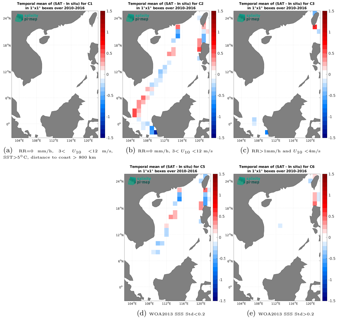
Figure 12: Temporal mean gridded over spatial boxes of size 1^\circ \times 1^\circ of \Delta\text{SSS} (SMOS SSS L3 v8 - 18 Days (CATDS-CEC-LOCEAN) - TSG (LEGOS-DM)) for 5 different subdatasets corresponding to: RR=0 mm/h, 3 < U_{10} < 12 m/s, SST > 5^\circ\text{C} , distance to coast > 800 km (a), RR=0 mm/h, 3 < U_{10} < 12 m/s (b), RR > 1 mm/h and U_{10} < 4 m/s (c), WOA2013 SSS Std < 0.2 (d), WOA2013 SSS Std > 0.2 (e).
