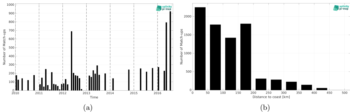
Figure 1: Number of match-ups between TSG (LEGOS-DM) and SMOS SSS L3 v8 - 18 Days (CATDS-CEC-LOCEAN) SSS as a function of time (a) and as function of the distance to coast (b) over the South China Sea Pi-MEP region and for the full satellite product period.
