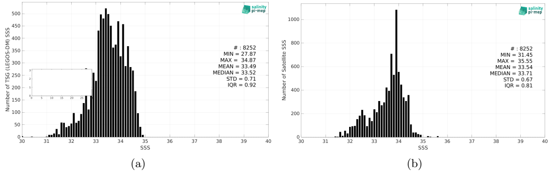
Figure 2: Histograms of SSS from TSG (LEGOS-DM) (a) and SMOS SSS L3 v8 - 18 Days (CATDS-CEC-LOCEAN) (b) considering all match-up pairs per bins of 0.1 over the South China Sea Pi-MEP region and for the full satellite product period.
