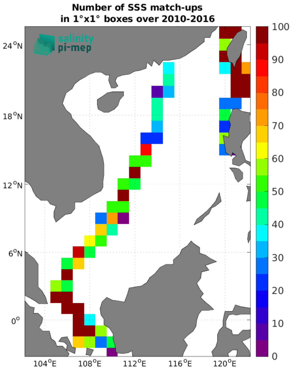
Figure 4: Number of SSS match-ups between TSG (LEGOS-DM) SSS and the SMOS SSS L3 v8 - 18 Days (CATDS-CEC-LOCEAN) SSS product for the South China Sea Pi-MEP region over 1^\circ \times 1^\circ boxes and for the full satellite product period.
