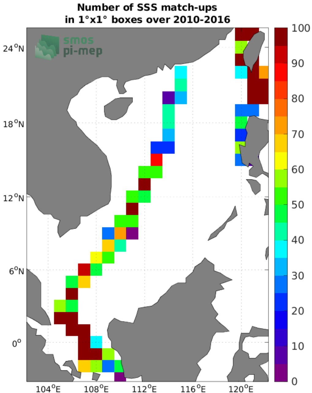
Figure 4: Number of SSS match-ups between TSG (LEGOS-DM) SSS and the SMOS SSS L3 v8 - 18 Days (CATDS-CECOS-LOCEAN) SSS product for the South China Sea Pi-MEP region over 1°x1° boxes and for the full satellite product period.
