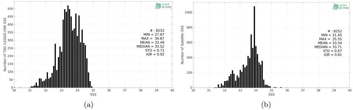
Figure 2: Histograms of SSS from TSG (LEGOS-DM) (a) and SMOS SSS L3 v8 - 18 Days (CATDS-CECOS-LOCEAN) (b) considering all match-up pairs per bins of 0.1 over the South China Sea Pi-MEP region and for the full satellite product period.
