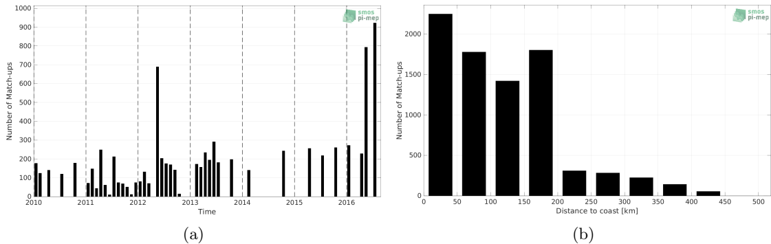
Figure 1: Number of match-ups between TSG (LEGOS-DM) and SMOS SSS L3 v8 - 18 Days (CATDS-CECOS-LOCEAN) SSS as a function of time (a) and as function of the distance to coast (b) over the South China Sea Pi-MEP region and for the full satellite product period.
