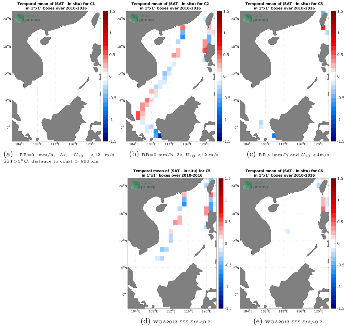
Figure 12: Temporal mean gridded over spatial boxes of size 1^\circ \times 1^\circ of \Delta\text{SSS} (SMOS SSS L3 v8 - 18 Days (CATDS-CECOS-LOCEAN) - TSG (LEGOS-DM)) for 5 different subdatasets corresponding to: RR=0 mm/h, 3 < U_{10} < 12 m/s, SST > 5^\circ\text{C} , distance to coast > 800 km (a), RR=0 mm/h, 3 < U_{10} < 12 m/s (b), RR > 1 mm/h and U_{10} < 4 m/s (c), WOA2013 SSS Std < 0.2 (d), WOA2013 SSS Std > 0.2 (e).
