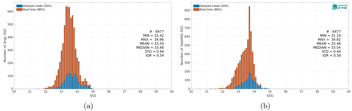
Figure 2: Histograms of SSS from Argo (a) and SMOS SSS L3 v8 - 18 Days (CATDS-CEC-LOCEAN) (b) considering all match-up pairs per bins of 0.1 over the South China Sea Pi-MEP region and for the full satellite product period.
