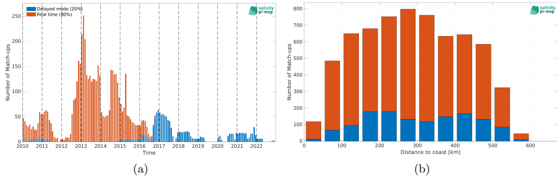
Figure 1: Number of match-ups between Argo and SMOS SSS L3 v8 - 18 Days (CATDS-CEC-LOCEAN) SSS as a function of time (a) and as function of the distance to coast (b) over the South China Sea Pi-MEP region and for the full satellite product period.
